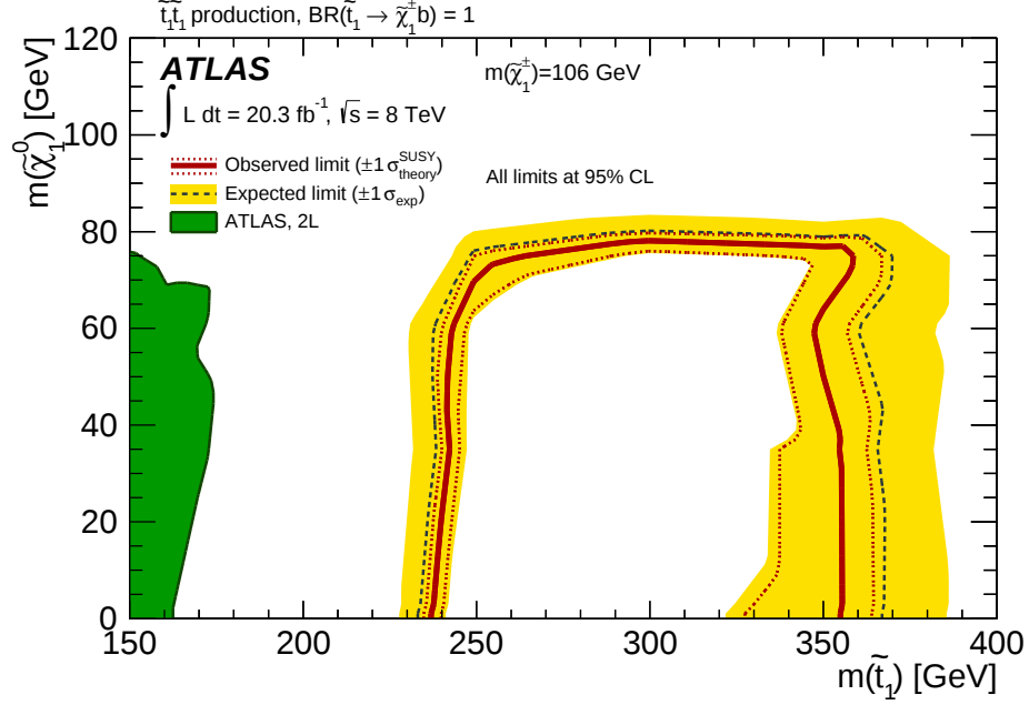
Figure 20. Observed and expected exclusion contours at 95% CL in the (\tilde{t}_1, \tilde{\chi}_1^0) mass plane for a fixed value of m(\tilde{\chi}_1^\pm) = 106 GeV. The dashed and solid lines show the 95% CL expected and observed limits, respectively, including all uncertainties except for the theoretical signal cross-section uncertainty (PDF and scale). The band around the expected limit shows the \pm 1\sigma expectation. The dotted \pm 1\sigma lines around the observed limit represent the results obtained when moving the nominal signal cross-section up or down by the theoretical uncertainty. The solid green area shows the excluded region from a previous ATLAS two-lepton analysis [19].
