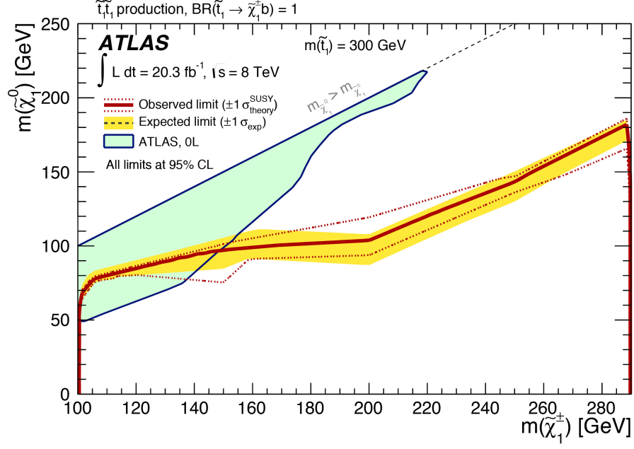
Figure 16. Observed and expected exclusion contours at 95% CL in the (\tilde{\chi}_1^+, \tilde{\chi}_1^0) mass plane for a fixed value of m(\tilde{t}_1) = 300 \text{ GeV} . The dashed and solid lines show the 95% CL expected and observed limits, respectively, including all uncertainties except for the theoretical signal cross-section uncertainty (PDF and scale). The band around the expected limit shows the \pm 1\sigma expectation. The dotted \pm 1\sigma lines around the observed limit represent the results obtained when moving the nominal signal cross-section up or down by the theoretical uncertainty. The solid light azure area labelled 0L is the exclusion contour from the ATLAS zero lepton direct top squark analysis [21].
