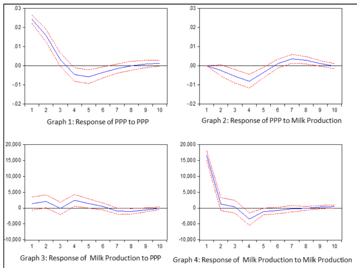
Figure 10 – Impulse response function analysis
