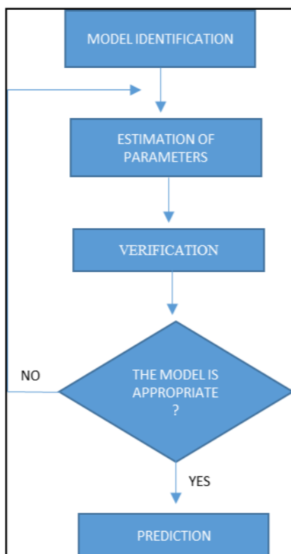
Figure 1 – Box and Jenkins iterative cycle flowchart
