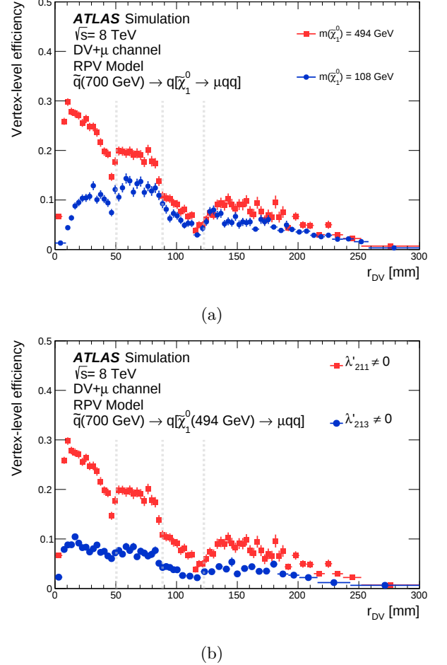
FIG. 3: Comparisons of the vertex-level efficiency as a function of the vertex radial position r_{\text{DV}} for different RPV samples. The vertical gray lines show the position of the first, second, and third pixel layers. (a) For the \tilde{q} \rightarrow q[\tilde{\chi}_1^0 \rightarrow \mu qq] ( \lambda'_{211} ) samples with m_{\tilde{q}} = 700 GeV, comparing two cases of different LLP masses: m_{\tilde{\chi}_1^0} = 494 GeV, and m_{\tilde{\chi}_1^0} = 108 GeV. (b) For the \tilde{q} \rightarrow q[\tilde{\chi}_1^0 \rightarrow \mu qq] ( \lambda'_{211} ) and \tilde{q} \rightarrow q[\tilde{\chi}_1^0 \rightarrow \mu qb] ( \lambda'_{213} ) samples, indicated by the relevant nonzero RPV couplings.
