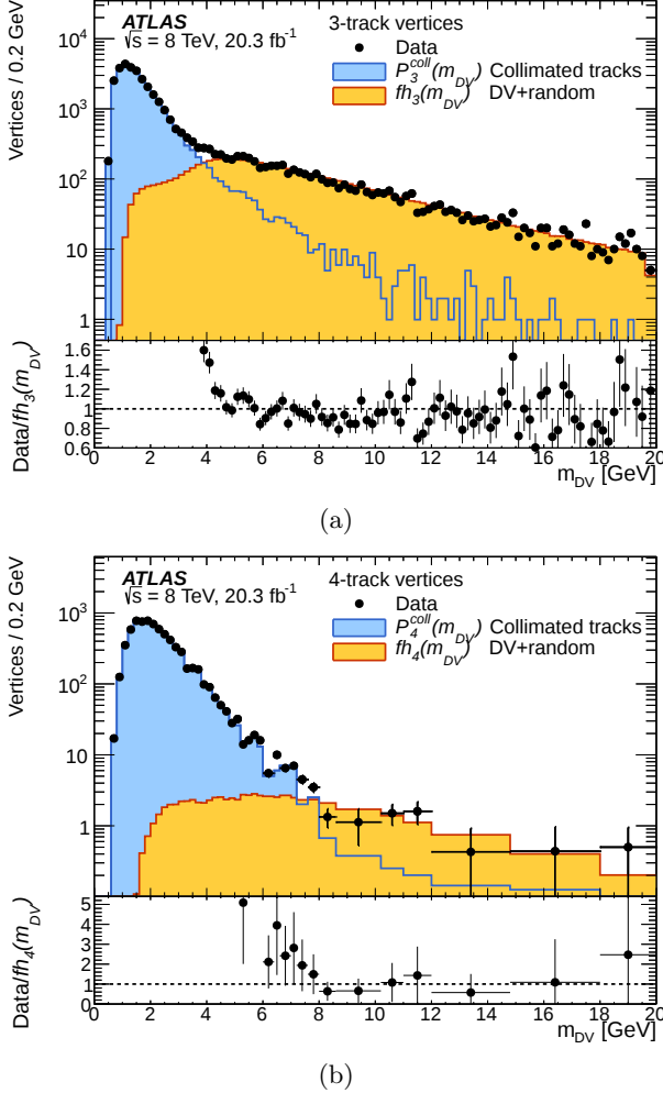
FIG. 5: The mass distribution for (a) 3-track and (b) 4-track vertices (data points) from the jets+ E_{\text{T}}^{\text{miss}} stream in Region 6, overlaid with the model fh_3(m_{\text{DV}}) of Eq. (5) (yellow-shaded histogram) at high mass. The lower panel of each plot shows the ratio of the data to this model. The model for the collimated-track contribution P_3^{\text{coll}}(m_{\text{DV}}) (blue-shaded histogram), which is correlated with the low-mass data but not used for estimating the signal-region background, is also shown.
