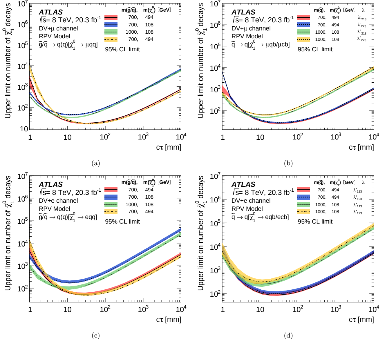
FIG. 12: RPV-scenario upper limits at 95% confidence level on the number of neutralinos in 20.3 \text{ fb}^{-1} that decay into (a) \mu q q (with q indicating a u - or d -quark), (b) \mu q b and \mu c b (indicated by the nonzero RPV couplings \lambda'_{213} and \lambda'_{223} , respectively), (c) e q q , and (d) e q b and e c b ( \lambda'_{113} and \lambda'_{123} , respectively). The upper limits account for the vertex-level efficiency for each value of the neutralino proper decay distance c\tau . The different curves show the results for different masses of the primary gluino or squark and of the long-lived neutralino, while the shaded bands indicate \pm 1\sigma variations in the expected limit.
