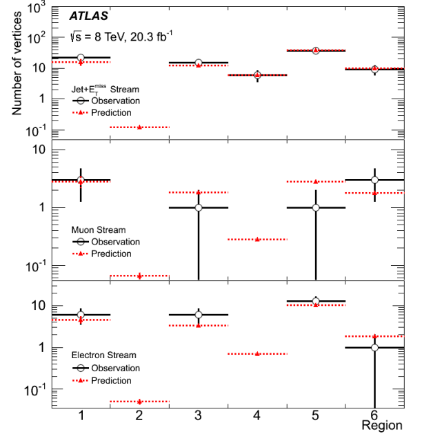
FIG. 6: Summary of the number of observed (black open circles) 4-track, high- m_{\text{DV}} vertices in each of the radial regions and filter-selection streams and the predicted number (red triangles), from Eq. (7). In Region 1, the prediction includes the contribution from merging of two 2-track vertices (see Sec. VIA 2). The error bars on the prediction are too small to be visible, and in some bins no events are observed.
