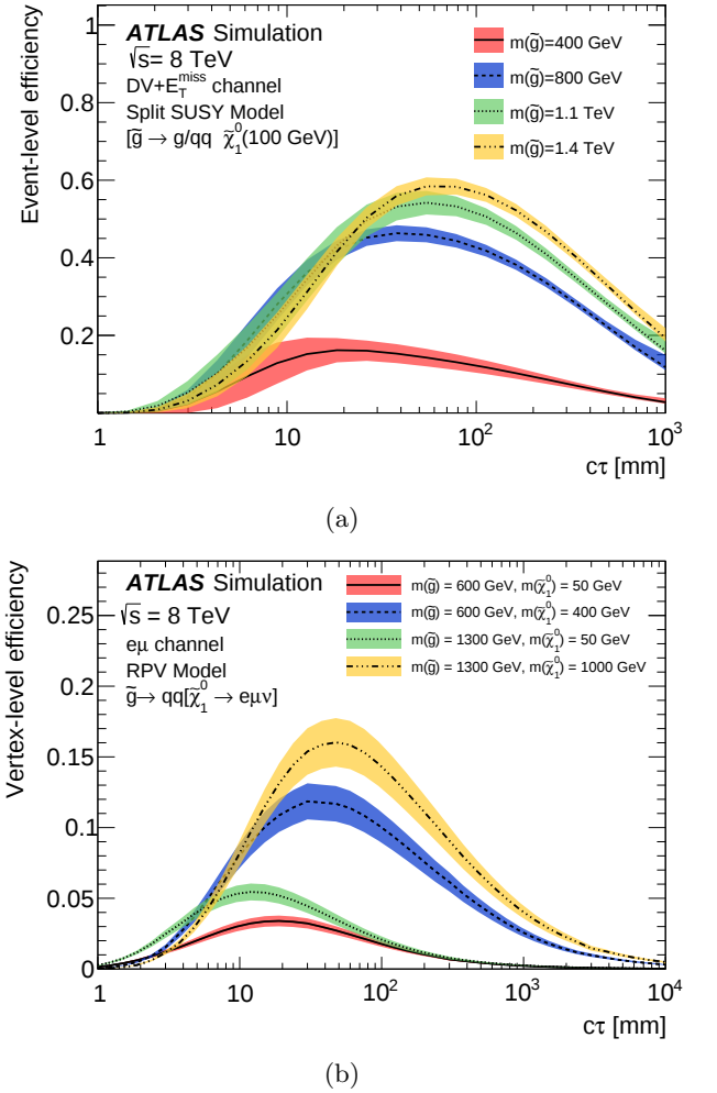
FIG. 4: (a) The event-level efficiency as a function of c\tau for split-supersymmetry [ \tilde{g} \rightarrow g/q\bar{q}\tilde{\chi}_1^0(100 \text{ GeV}) ] samples with various gluino masses, reconstructed in the DV+ E_T^{\text{miss}} channel. (b) The vertex-level efficiency for the RPV \tilde{g} \rightarrow qq[\tilde{\chi}_1^0 \rightarrow e\mu\nu] samples with combinations of gluino and neutralino masses, reconstructed in the e\mu dilepton channel. The total uncertainties on the efficiencies are shown as bands (see Sec. VII).
