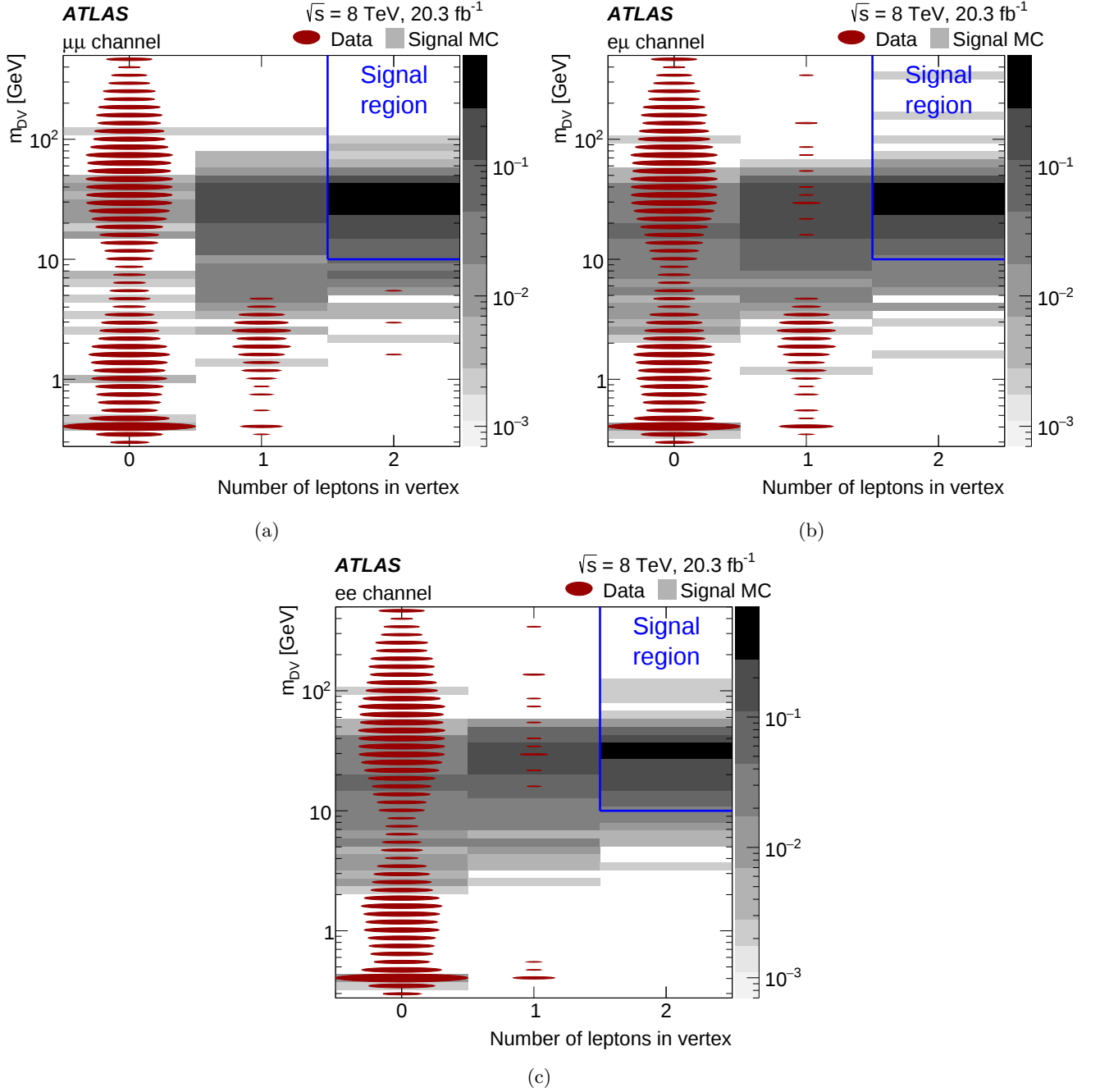
FIG. 9: The distribution of dilepton-vertex candidates in terms of the vertex mass versus the number of lepton candidates in the vertex, in the (a) \mu^+\mu^- , (b) e^\pm\mu^\mp , and (c) e^+e^- search channels. The data distributions are shown with red ovals, the area of the oval being proportional to the logarithm of the number of vertex candidates in that bin. The gray squares show the \tilde{g}(600 \text{ GeV}) \rightarrow qq[\tilde{\chi}_1^0(50 \text{ GeV}) \rightarrow \mu\mu\nu/e\mu\nu/ee\nu] signal MC sample. The shape of the background m_{DV} distribution arises partly from the lepton-candidate p_T requirements. The signal region defined by the two-lepton and m_{DV} > 10 \text{ GeV} requirements is indicated.
