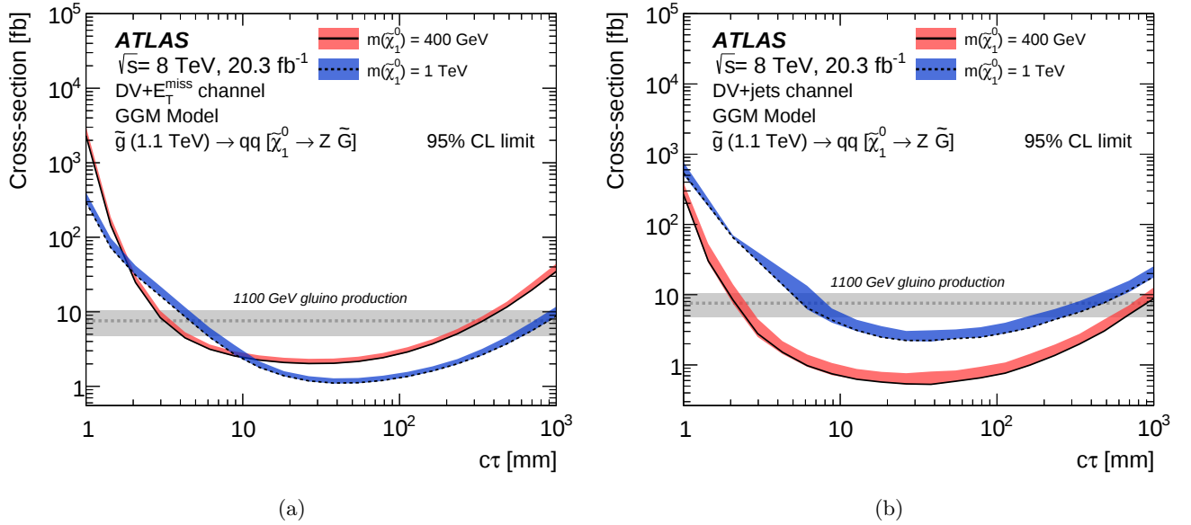
FIG. 17: The 95% confidence-level upper limits, obtained from the (a) DV+ E_T^{\text{miss}} and (b) DV+jets searches, on the production cross section for a pair of gluinos of mass 1.1 TeV that decay into two quarks and a long-lived neutralino in the GGM scenario. For further details see Fig. 14.
