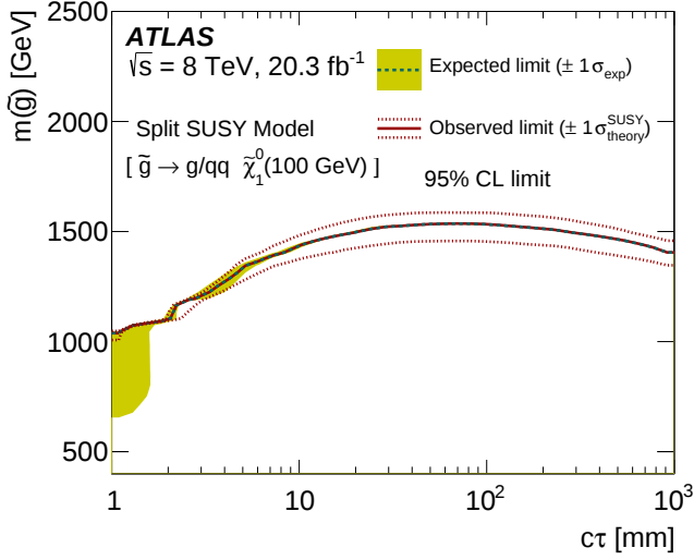
FIG. 19: The 95% confidence-level excluded regions lie below the curves shown in the mass-versus- c\tau plane for the split-supersymmetry samples, with the gluino decaying into a gluon or light quarks, plus a 100 GeV neutralino. The shaded bands indicate \pm 1\sigma variations in the expected limit, while the dotted lines indicate the effect of varying the production cross section by 1 standard deviation. The expected and observed limits are identical.
