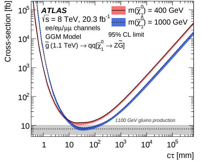
FIG. 15: The 95% confidence-level upper limits, obtained from the dilepton search, on the production cross section for a pair of gluinos of mass 1.1 TeV that decay into two quarks and a long-lived neutralino in the GGM scenario for two values of the neutralino mass.. For further details see Fig. 14.
