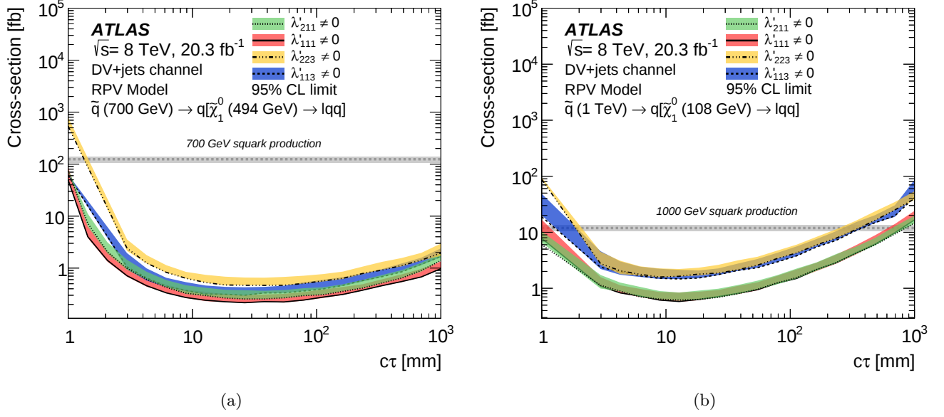
FIG. 16: The 95% confidence-level upper limits, obtained from the DV+jets search, on the production cross section for a pair of squarks in the RPV scenario, with the neutralino decaying to a lepton and two quarks, according to the nonzero \lambda' couplings indicated in each case. The squark and neutralino masses are (a) 700 GeV and 494 GeV or (b) 1 TeV and 108 GeV, respectively, representing the results for different neutralino masses and boosts. For further details see Fig. 14.
