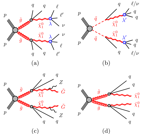
FIG. 1: Diagrams representing some of the processes under study, corresponding to the simulated event samples. In RPV scenarios, the long-lived neutralino may decay via the (a) \lambda_{ijk} or (b) \lambda'_{ijk} couplings. (c) Long-lived neutralino decay in a GGM scenario. (d) Long-lived R -hadron decay in a split-supersymmetry scenario. The quarks and leptons shown may have different flavors. Filled circles indicate effective interactions.
