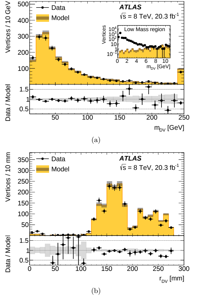
FIG. 8: Distributions of the (a) vertex mass and (b) vertex position radius for vertices composed of two nonlepton tracks in the data sample (data points), and the predicted model distribution obtained from vertices formed by combining tracks from two different data events (shaded histograms). The ratio of the data to the model distributions is shown below each plot. The gray bands indicate the statistical uncertainties for the predicted distributions. The inset shows the mass distribution in the low-mass region, elsewhere m_{DV} > 10 GeV is required. In (a), the highest bin shows the histogram overflow.
