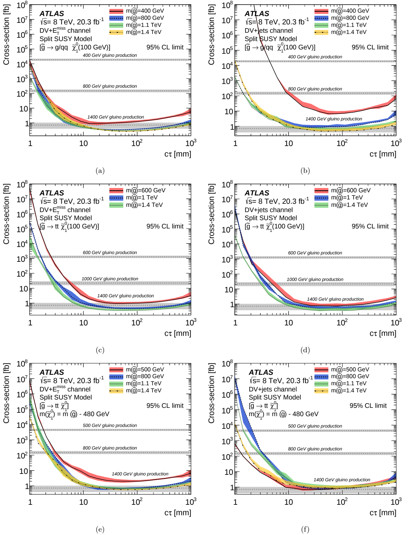
FIG. 18: The 95% confidence-level upper limits, obtained from the (a, c, e) DV+ E_T^{\text{miss}} and (b, d, f) DV+jets searches, on the cross section for gluino pair production in the split-supersymmetry model, with the gluino decaying to a neutralino plus either (a, b) a gluon or a light-quark pair or (c, d, e, f) a pair of top quarks. The mass of the neutralino is 100 GeV in (a, b, c, d) and is 480 GeV smaller than the gluino mass in (e, f). For further details see Fig. 14.
