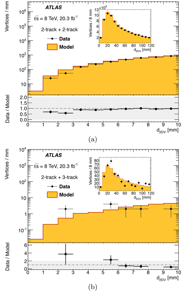
FIG. 7: The distribution of the distance d_{2DV} between (a) two 2-track vertices and (b) a 2-track vertex and a 3-track vertex with a combined mass above 10 GeV for the jets+ E_T^{miss} stream data (data points) and in the model sample, in which the two vertices are in different events (histogram). A conservative 100% uncertainty on the model is shown in the data/model ratio plot. The inset shows the d_{2DV} distance up to values of 120 mm. The merged-vertex background estimate is determined from the area under the model distribution in the range d_{2DV} < 1 mm in (b).
