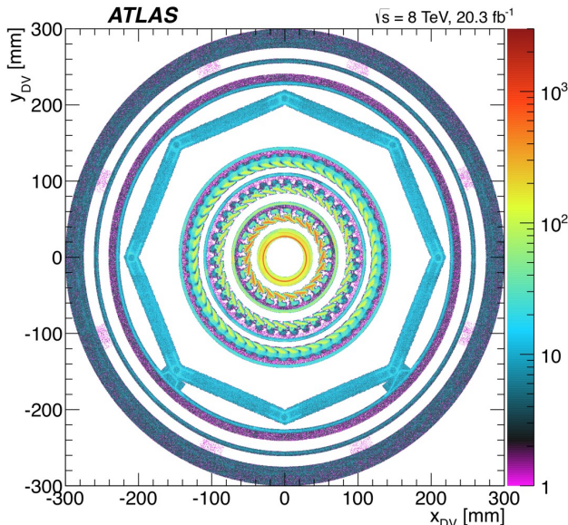
FIG. 2: Transverse-plane density (in arbitrary units) of vertices with fewer than five tracks in material regions that are excluded by the material veto in the region |z| < 300 mm. The innermost circle corresponds to the beam pipe. This is surrounded by the three pixel layers. The octagonal shape and outermost circles are due to support structures separating the pixel and SCT detectors.
