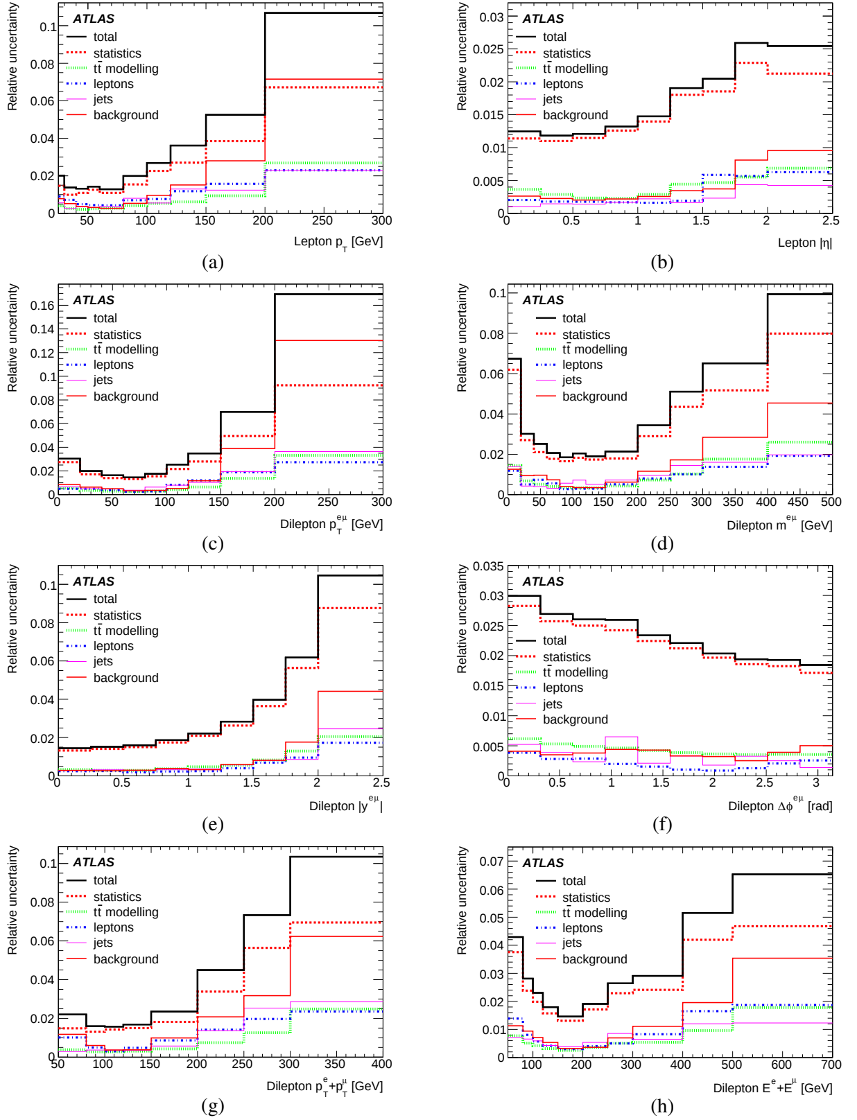
Figure 6: Relative uncertainties on the measured normalised differential cross-sections coming from data statistics, t\bar{t} modelling, leptons, jets and background, as a function of each lepton or dilepton differential variable. The total uncertainty is shown by the black lines, and also includes small contributions from the integrated luminosity and LHC beam energy uncertainties.
