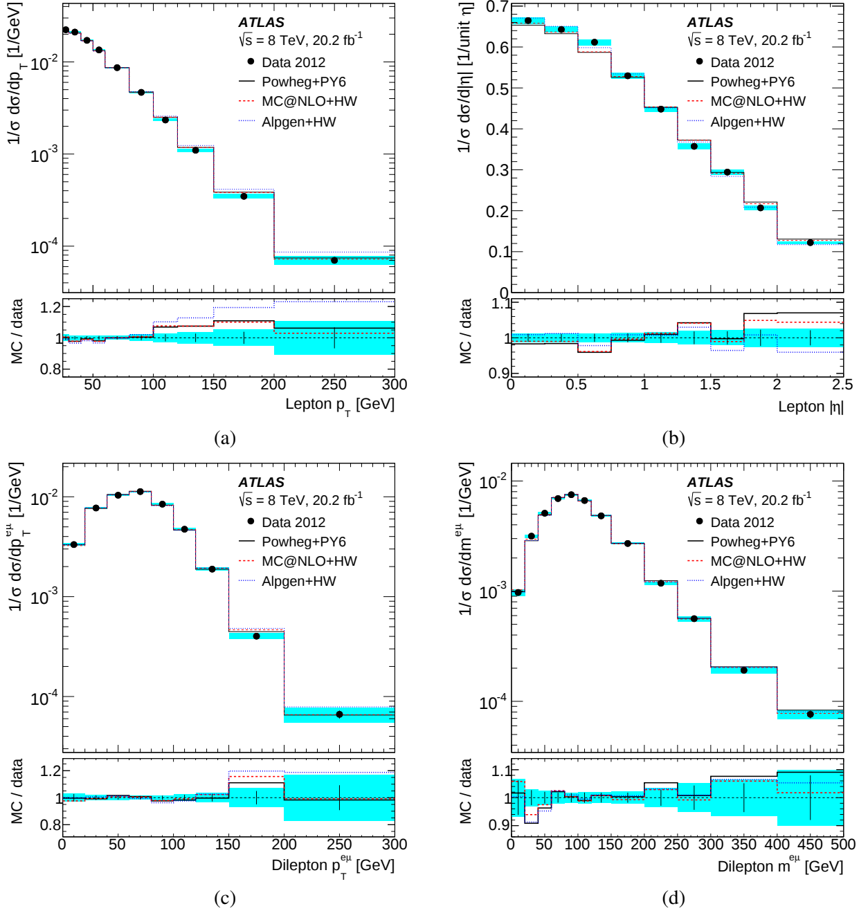
Figure 7: Normalised differential cross-sections as a function of (a) p_T^\ell , (b) |\eta^\ell| , (c) p_T^{e\mu} and (d) m^{e\mu} . The measured values are shown by the black points with error bars corresponding to the data statistical uncertainties and cyan bands corresponding to the total uncertainties in each bin, and include the contributions via W \rightarrow \tau \rightarrow e/\mu decays. The results are compared to the predictions from the POWHEG + PYTHIA6, MC@NLO + HERWIG and ALPGEN + HERWIG t\bar{t} simulation samples. The lower plots show the ratios of predictions to data, with the error bars indicating the data statistical uncertainties and the cyan bands indicating the total uncertainties in the measurements.
