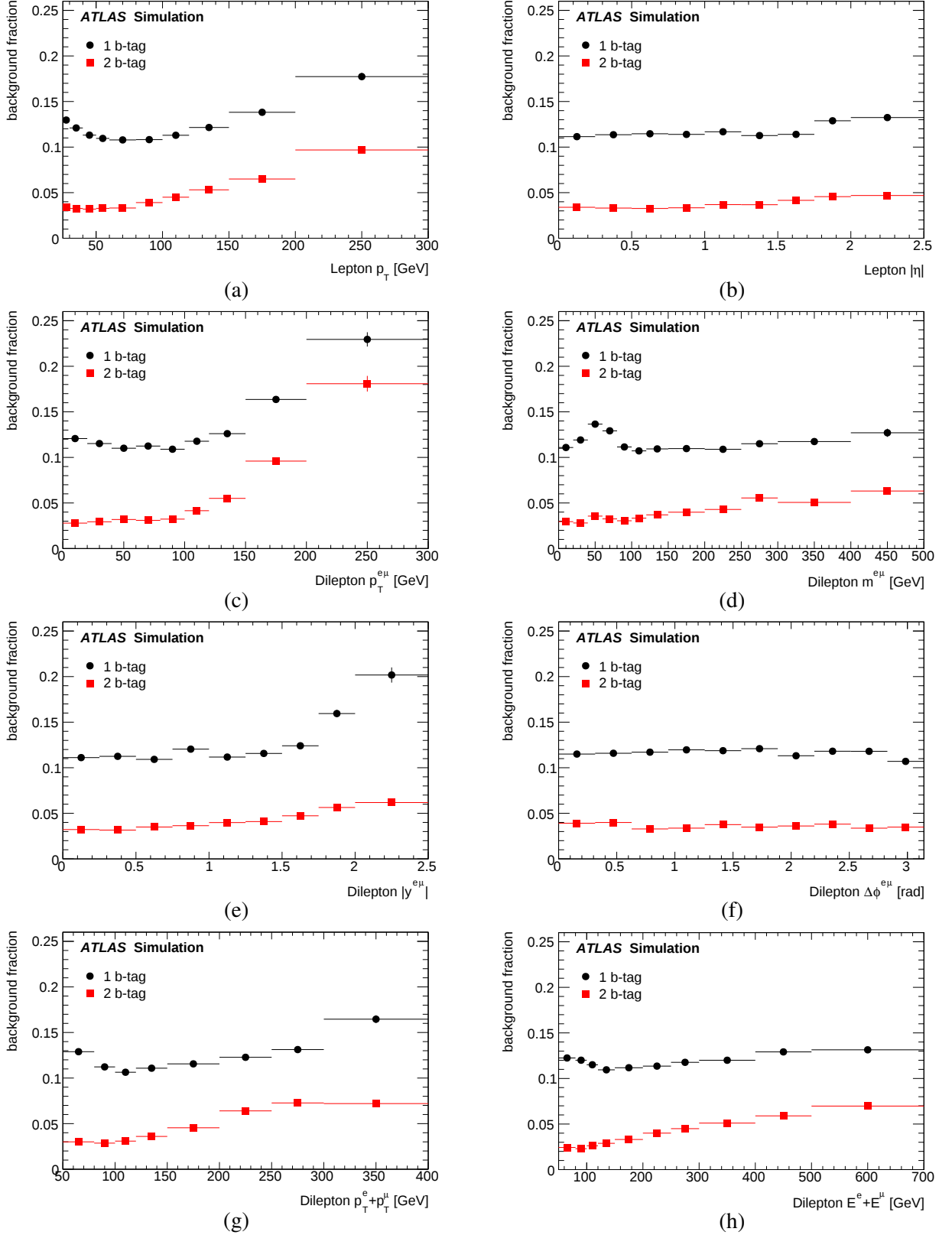
Figure 3: Estimated background fractions in the one and two b -tagged samples as functions of each lepton and dilepton differential variable, estimated from simulation alone. The error bars correspond to the statistical uncertainties of the simulation samples, and are often smaller than the marker size.
