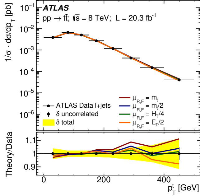
Figure 20: Measurement of the top quark p_T spectrum in pp collisions at \sqrt{s} = 8 TeV from ATLAS events with a lepton and at least four jets [20], compared to the predictions from MCFM as used in this analysis with NNPDF 3.0, m_t = 173.3 GeV, and QCD scale choices of \mu_F = \mu_R = m_t/2 , H_T/4 and E_T/2 , as well as with \mu_F = \mu_R = m_t . The measurement uncertainties are represented by the yellow band, with the uncorrelated component shown by the black error bar. The lower plots show the ratios of the different predictions to the data.
