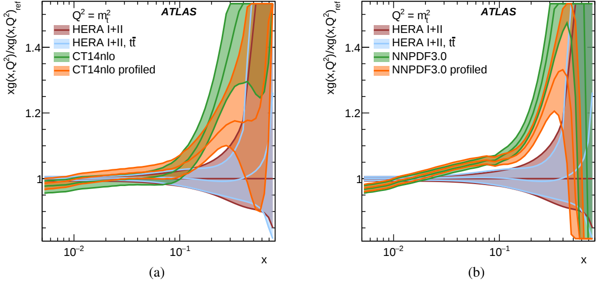
Figure 16: Ratios of various gluon PDFs and their uncertainty bands to the gluon PDF determined from HERA I+II data alone (red shading). The blue shaded band shows the gluon PDF from the fit to HERA I+II data plus the normalised differential cross-section distributions as a function of |\eta^\ell| , |y^{e\mu}| and E^e + E^\mu in t\bar{t} events. The green band shows the gluon PDF from the CT14 [103] PDF set in (a) and the NNPDF 3.0 [105] PDF set in (b). The orange bands show the result of profiling these PDFs to the t\bar{t} normalised differential cross-section data.
