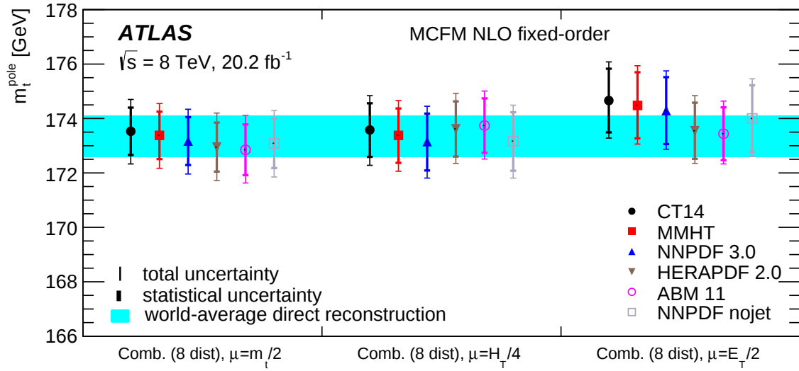
Figure 21: Measurements of the top quark mass using predictions derived from MCFM with the CT14, MMHT, NNPDF 3.0, HERAPDF 2.0, ABM 11 and NNPDF 3.0_nojet PDF sets, and the central QCD factorisation and renormalisation scales \mu_F and \mu_R set to m_t/2 , H_T/4 and E_T/2 . The results are derived from a combined fit to all eight lepton and dilepton distributions. For comparison, the world-average of mass measurements from reconstruction of the top quark decay products [121] is shown by the cyan band.
