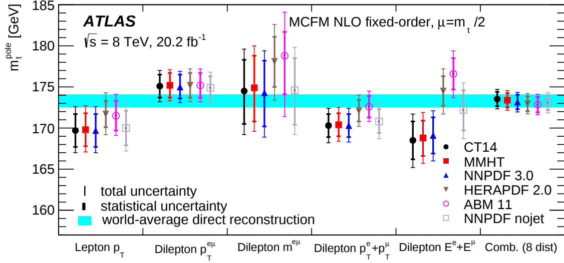
Figure 19: Measurements of the top quark mass using predictions derived from MCFM with the CT14, MMHT, NNPDF 3.0, HERAPDF 2.0, ABM 11 and NNPDF 3.0_nojet PDF sets. The central factorisation and renormalisation scales are set to \mu_F = \mu_R = m_t/2 . The results from fitting templates of the single lepton p_T^\ell and dilepton p_T^{e\mu} , m^{e\mu} , p_T^e + p_T^\mu and E^e + E^\mu distributions one at a time, and of a combined fit to these five distributions plus the |\eta^\ell| , |y^{e\mu}| and \Delta\phi^{e\mu} distributions together, are shown. For comparison, the world-average of mass measurements from reconstruction of the top quark decay products and its uncertainty [121] is shown by the cyan band.
