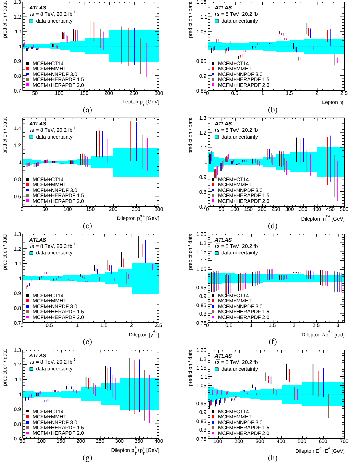
Figure 14: Ratios of MCFM fixed-order predictions of normalised differential cross-sections to data as a function of lepton and dilepton variables, using the CT14, MMHT, NNPDF 3.0, HERAPDF 1.5 and HERAPDF 2.0 PDF sets for the predictions. Contributions via W \rightarrow \tau \rightarrow e/\mu decays are not included, and the MCFM predictions have been corrected to include QED final-state radiation effects. The total data uncertainties are shown by the cyan bands around unity, and the total uncertainty for each prediction (including QCD scales, PDFs, and the strong coupling constant \alpha_s ) are shown by the vertical bars.
