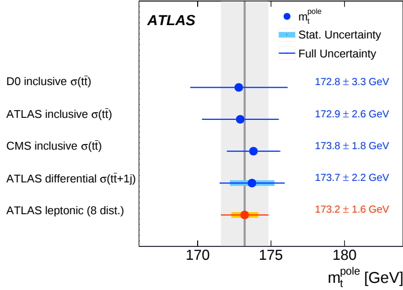
Figure 22: Result of the top quark pole mass determination from the combined fit to eight leptonic distributions (shown by the red point and grey band), compared to other determinations from inclusive and differential cross-section measurements in t\bar{t} events [13, 15, 40, 41]. The statistical uncertainties are shown separately by the thick error bars where available.
