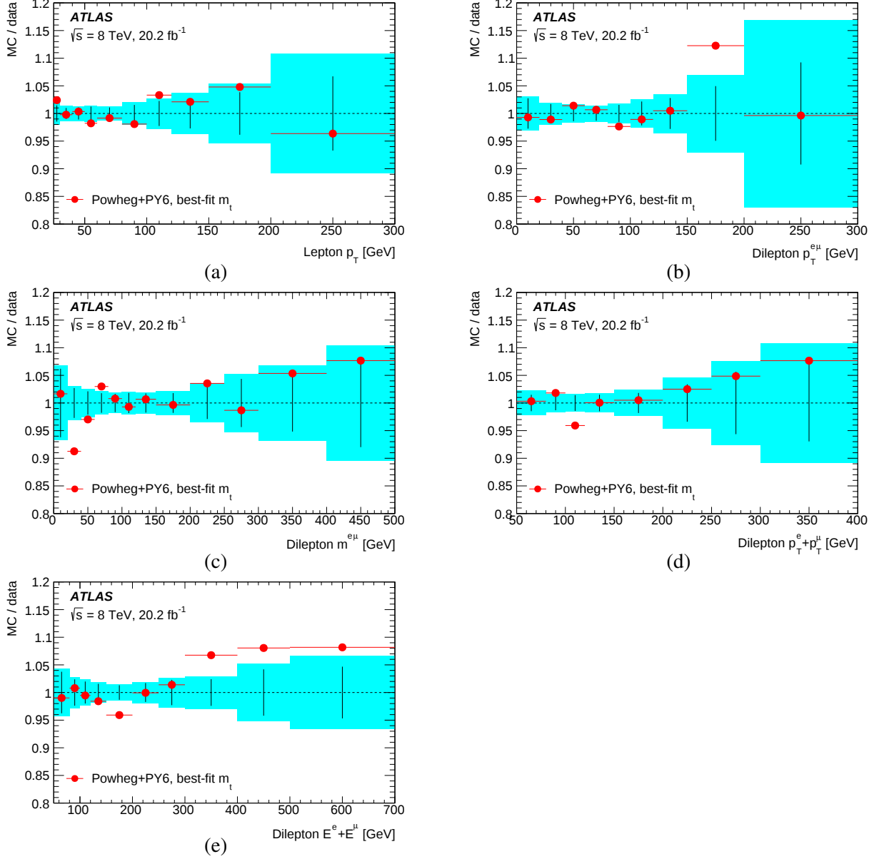
Figure 18: Ratios of predictions of normalised differential cross-sections to data as a function of (a) p_T^\ell , (b) p_T^{e\mu} , (c) m^{e\mu} , (d) p_T^e + p_T^\mu and (e) E^e + E^\mu , with the prediction taken from POWHEG + PYTHIA6 with the CT10 PDF at the best-fit top quark mass m_t for each distribution. The data statistical uncertainties are shown by the black error bars around a ratio of unity, and the total experimental uncertainties by the cyan band.
