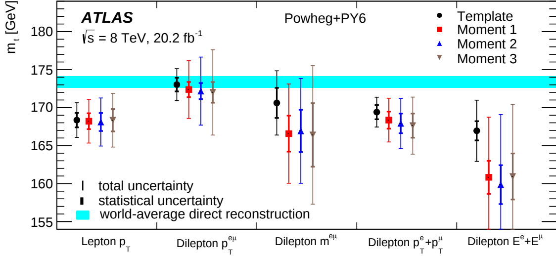
Figure 17: Measurements of the top quark mass using templates derived from POWHEG + PYTHIA6 with the CT10 PDF set. The results from fitting templates of the single lepton p_T^\ell and dilepton p_T^{e\mu} , m^{e\mu} , p_T^e + p_T^\mu and E^e + E^\mu distributions, and from the first, second and third moments of these distributions, are shown. For comparison, the world-average of mass measurements from reconstruction of the top quark decay products and its uncertainty [121] is shown by the cyan band.
