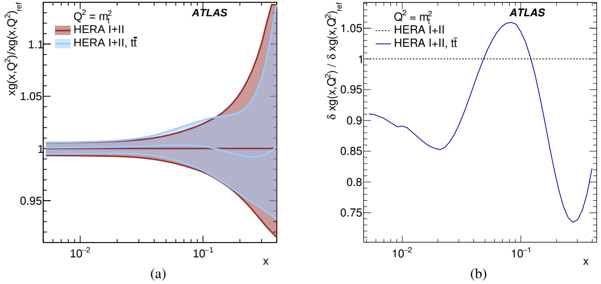
Figure 15: (a) Ratio of the gluon PDF determined from the fit using HERA I+II data plus the normalised differential cross-section distributions as a function of |\eta^\ell| , |y^{e\mu}| and E^e + E^\mu in t\bar{t} events, to the gluon PDF determined from the fit using HERA I+II data alone, as a function of Bjorken- x . The uncertainty bands are shown on the two PDFs as the blue and red shading. (b) Ratio of the relative uncertainty in the gluon PDF determined from the fit to HERA I+II plus t\bar{t} data to that from HERA data alone. The PDFs are shown evolved to the scale Q^2 = m_t^2 in both cases.
