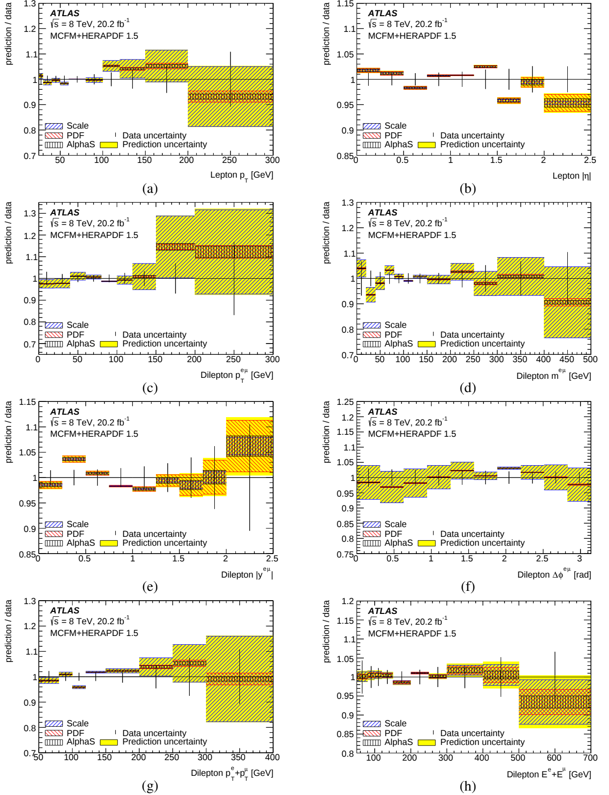
Figure 13: Ratios of MCFM + HERAPDF 1.5 fixed-order predictions of normalised differential cross-sections to data as a function of lepton and dilepton variables. Contributions via W \rightarrow \tau \rightarrow e/\mu decays are not included, and the MCFM predictions have been corrected to include QED final-state radiation effects. The total data uncertainties are shown by the error bars around unity. The separate uncertainties in the predictions from QCD scales, PDFs and the strong coupling constant \alpha_S are shown by the hatched bands, and the total uncertainties in the predictions are shown by the yellow band.
