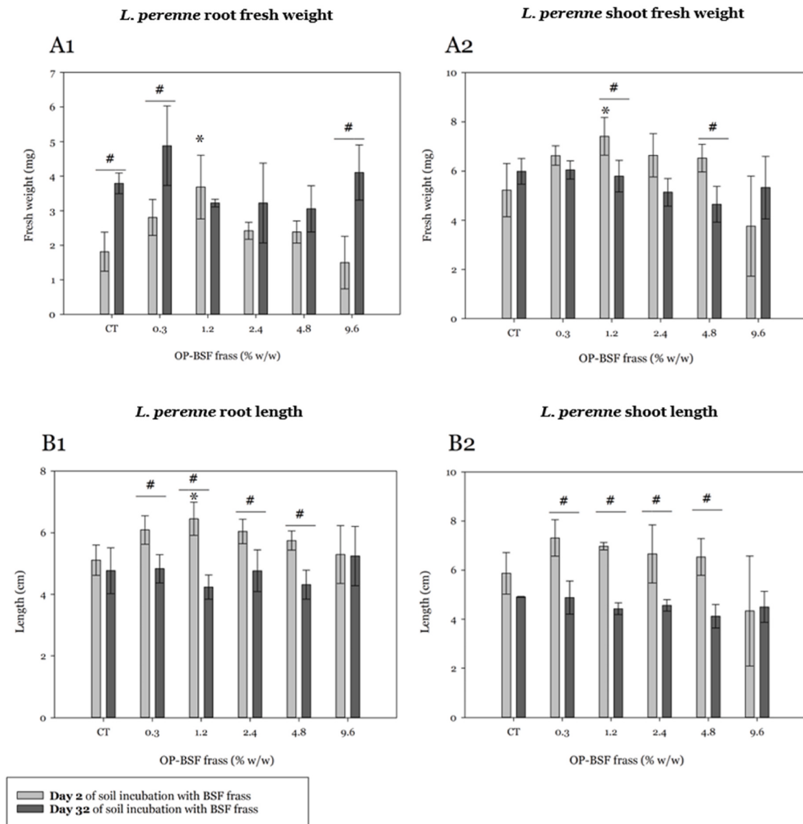
Fig. 3. Lolium perenne root (A1) and shoot (A2) fresh weight (FW), root (B1), and shoot (B2) length in plants exposed after three days of germination to soil amended with increased concentrations of olive pomace-derived frass (OP-BSF frass ). Two-way ANOVA analysis was conducted based on OP-BSF frass concentrations and incubation period. (*) significant differences in comparison with the respective control (CT) group (Dunnett's Method p \leq 0.001 ). (#) represents significant differences between both incubation periods (Dunnett's Method p \leq 0.001 ).
