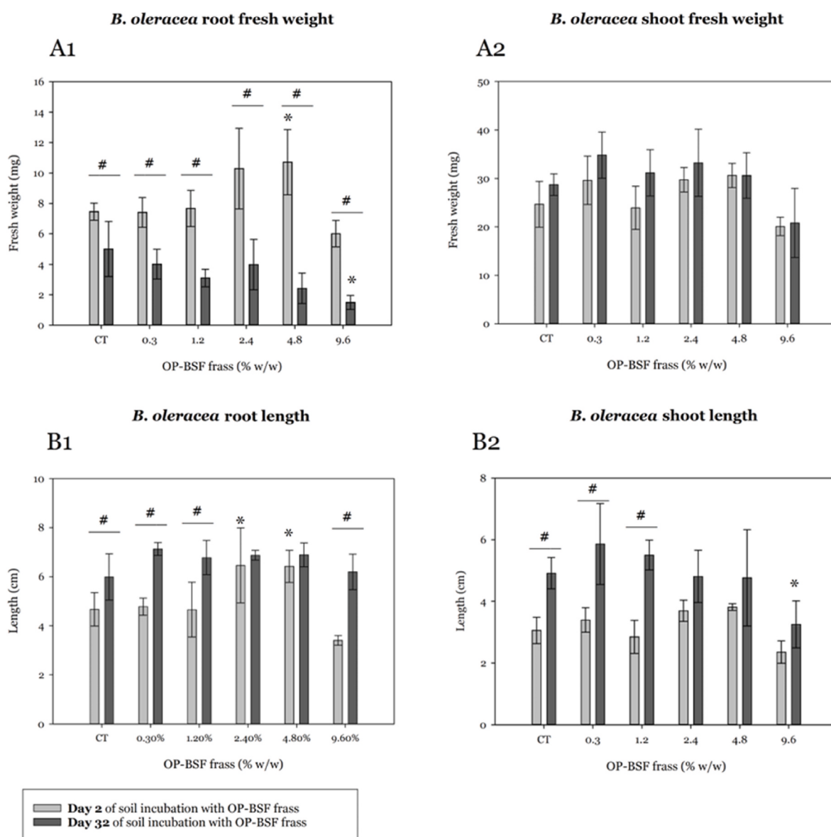
Fig. 2. Brassica oleracea root (A1) and shoot (A2) fresh weight and root (B1) and shoot (B2) length of plants exposed after 3 days of germination to soil amended with increased concentrations of olive pomace-derived frass (OP-BSF frass ). Two-way ANOVA analysis was conducted based on OP-BSF frass concentrations and incubation period. (*) significant differences in comparison with the respective control (CT) group (Dunnett's Method p \leq 0.001 ). (#) represents significant differences in the incubation period (Dunnett's test p \leq 0.001 ).
