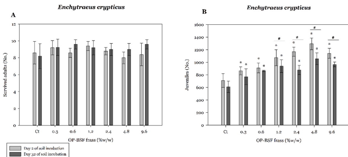
Fig. 1. Enchytraeus crypticus adult survival (A) and reproduction (B) after a 21d experiment with different olive pomace-derived frass (OP-BSF frass ) concentrations with 2 and 32 days of incubation. Data is presented as mean with standard deviation, and statistical analysis was performed using two-way ANOVA (OP-BSF frass concentrations and incubation period as factors) to determine significant differences in both endpoints. (*) significant differences in reproduction compared to the respective control (Ct) group (Dunnett's Method p \leq 0.001 ) at each sampling time. (#) represents significant differences in the same OP-BSF frass concentration in soil, comparing both incubation periods (Dunnett's test p \leq 0.001 ).
