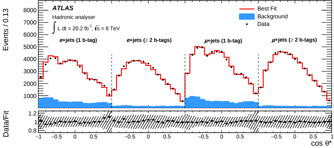
Figure 5: Post-fit distribution of \cos \theta^* for the hadronic analyser, in which the combination of four channels is performed (electron and muon, with exactly 1 b -tag and \geq 2 b -tags). The uncertainty band represents the total uncertainty in the fit result.
