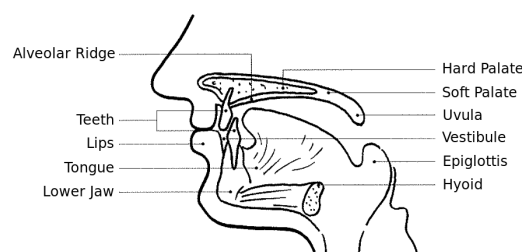
Figure 1. Main places of articulation in the vocal tract, adapted from Reference [5].
