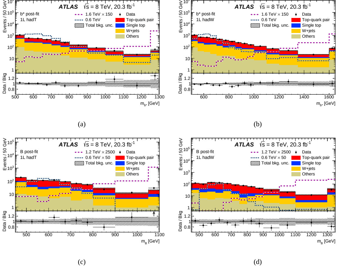
Figure 6: Distributions of the reconstructed mass in the b^* (top row) and B (bottom row) selection of the single-lepton analysis for the SM background processes, data and two b^* (top row) or B (bottom row) signal masses in the (a) b^* 1L hadT, (b) b^* 1L hadW, (c) B 1L hadT and (d) B 1L hadW signal regions. The signal distributions are scaled to the theory cross-sections multiplied by the indicated factor for better visibility and the background processes are normalised to their post-fit normalisation. The uncertainty band includes statistical and all systematic uncertainties. The first and last bin include the underflow and overflow, respectively. The binning of the figures is the same as used in the binned likelihood fit function.
