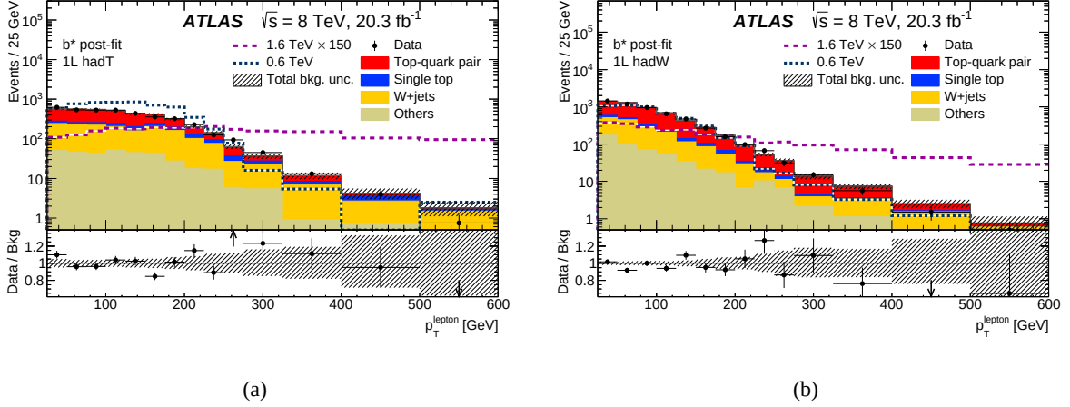
Figure 4: Distributions of the lepton transverse momentum in the b^* selection of the single-lepton analysis for the data, SM background processes and two b^* signal masses in the (a) b^* 1L \text{ hadT} and (b) b^* 1L \text{ hadW} signal regions. The signal distributions are scaled to the theory cross-sections multiplied by the indicated factor for better visibility and the background processes are normalised to their post-fit normalisation. The uncertainty band includes statistical and all systematic uncertainties. The last bin includes the overflow.
