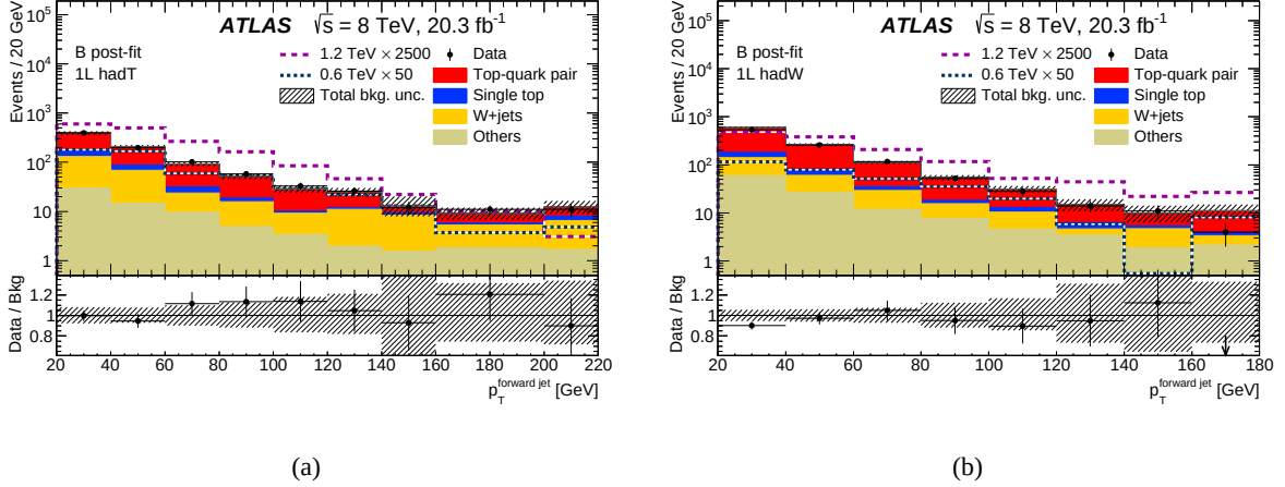
Figure 5: Distributions of the leading forward-jet transverse momentum in the B selection of the single-lepton analysis for the data events, SM background processes and two B signal masses in the (a) B 1L hadT and (b) B 1L hadW signal region. The signal distributions are scaled to the theory cross-sections multiplied by the indicated factor for better visibility and the background processes are normalised to their post-fit normalisation. The uncertainty band includes statistical and all systematic uncertainties. The last bin includes the overflow.
