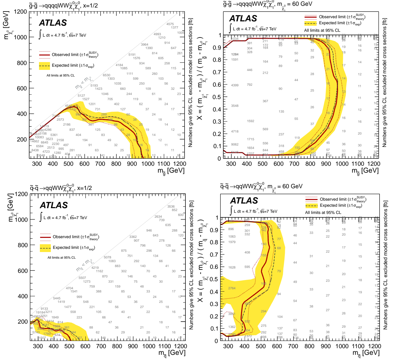
FIG. 10. Excluded regions at 95% confidence level in the parameter space of one-step simplified models. Top row: gluino pair production with \tilde{g} \rightarrow q\tilde{q}'\tilde{\chi}_1^\pm \rightarrow q\tilde{q}'W^\pm\tilde{\chi}_1^0 . Bottom row: squark pair production with \tilde{q}_L \rightarrow q'\tilde{\chi}_1^\pm \rightarrow q'W^\pm\tilde{\chi}_1^0 . In the left column, the chargino mass is set to be halfway between gluino (top) or squark (bottom) and LSP masses. In the right column, the LSP mass is fixed at 60 GeV and the masses of the chargino and gluino (top) or squark (bottom) are varied. The band around the median expected limit shows the \pm 1\sigma variations, including all uncertainties except theoretical uncertainties on the signal. The dotted lines around the observed limit indicate the sensitivity to \pm 1\sigma variations on these theoretical uncertainties. The plots are from the combination of the hard and soft single-lepton channels. The numbers indicate the excluded cross section in fb. A smaller excluded cross section implies a more stringent limit.
