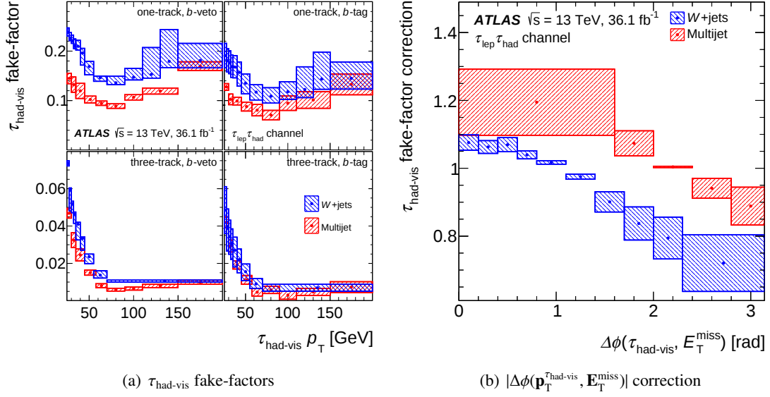
Figure 4: The \tau_{\text{had-vis}} identification fake-factors and the sequential |\Delta\phi(\mathbf{p}_T^{\tau_{\text{had-vis}}}, \mathbf{E}_T^{\text{miss}})| correction in the \tau_{\text{lep}} \tau_{\text{had}} channel. The multijet fake-factors are for the 2016 dataset only. The bands include all uncertainties.
