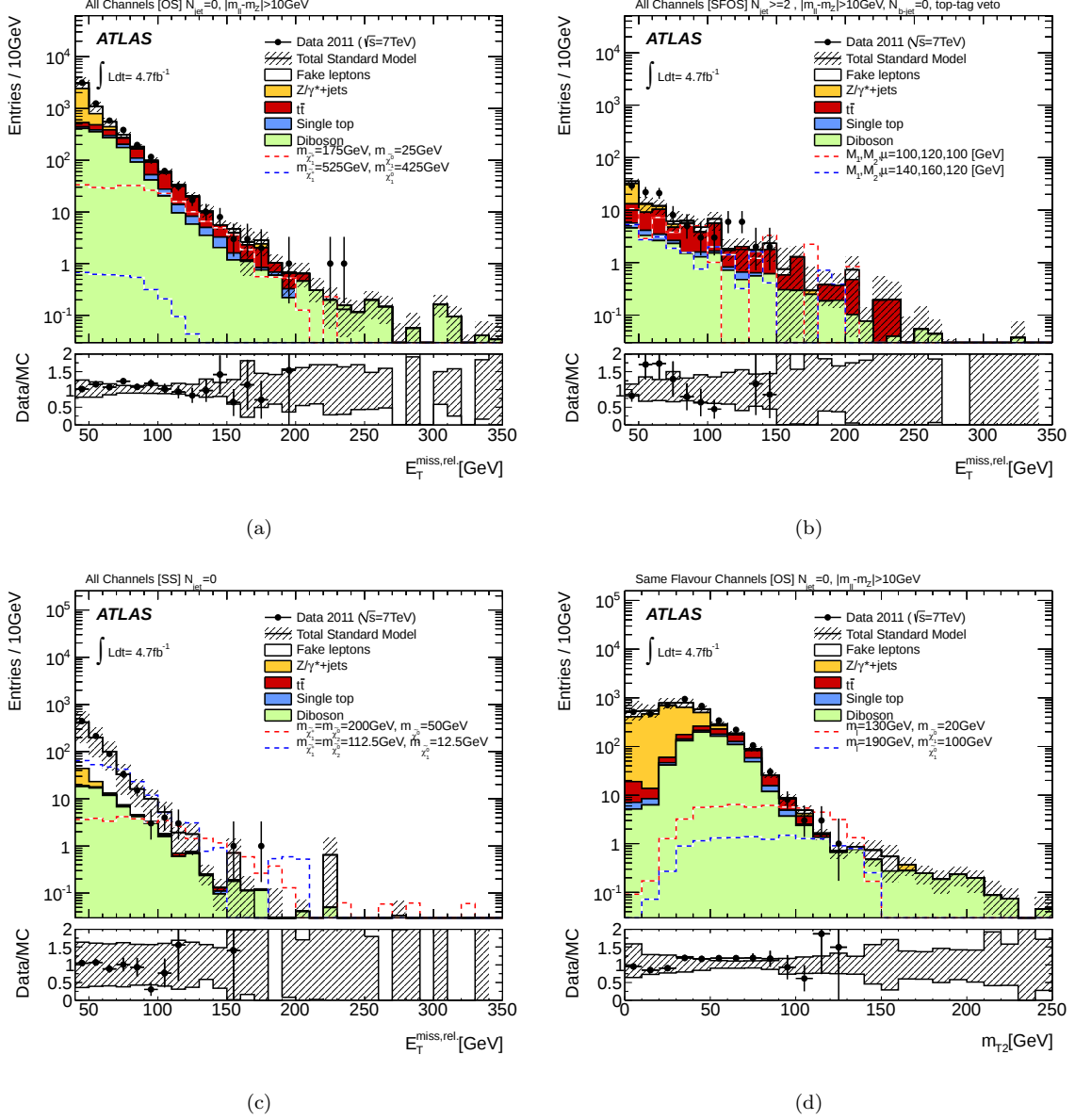
Figure 1: The E_T^{\text{miss,rel}} distributions prior to the final requirement on E_T^{\text{miss,rel}} for (a) SR-OSjveto, (b) SR-2jets and (c) SR-SSjveto, and (d) m_{T2} in SR- m_{T2} , prior to the application of the m_{T2} requirement. In (d) only the SF channels are shown. The hatched bands indicate the experimental uncertainties on the background expectations. All components are from MC except for that labelled “Fake leptons”. The contribution labelled “Diboson” accounts for WW , WZ and ZZ processes. The bottom panels show the ratio of the data to the expected background (points) and the systematic uncertainty on the background (shaded area). In each figure two signal points are illustrated. In (d) two models of direct slepton pair production are illustrated, with (\tilde{\ell}, \chi_1^0) masses of (130,20) and (190,100) GeV. In (a) the two points illustrated are for \tilde{\chi}_1^\pm \tilde{\chi}_1^\mp production in the simplified model with (\tilde{\chi}_1^\pm, \tilde{\chi}_1^0) masses of (175,25) and (525,425) GeV. In (c) the simplified model points illustrated have (\tilde{\chi}_1^\pm, \tilde{\chi}_1^0) masses of (200,50) and (112.5,12.5) GeV. In (b) two pMSSM model points with masses (M_1, M_2, M_\mu) of (100,120,100) and (140,160,300) GeV are illustrated.
