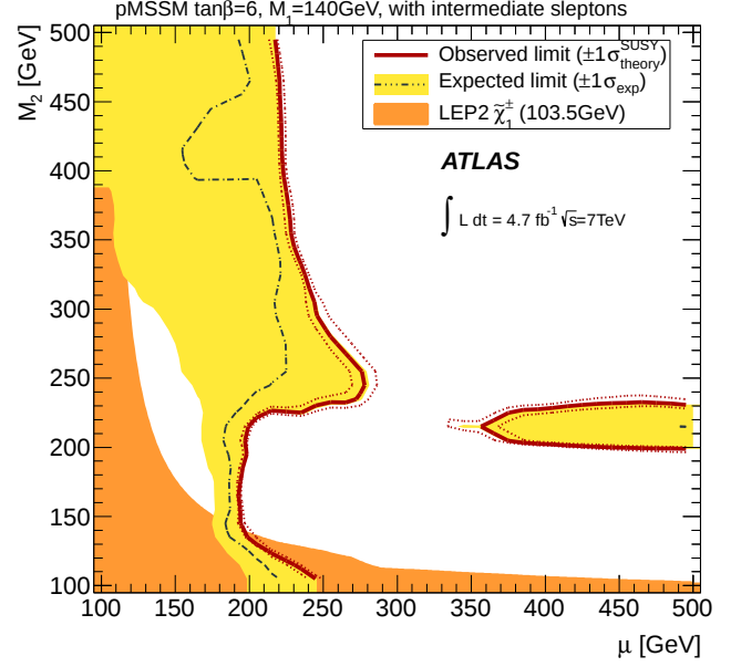
(b) M_1 = 140 \text{ GeV}
