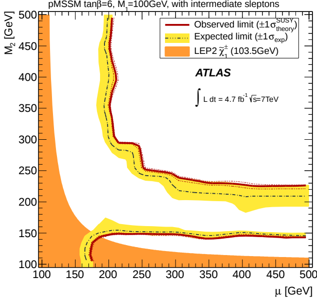
(a) M_1 = 100 \text{ GeV}
