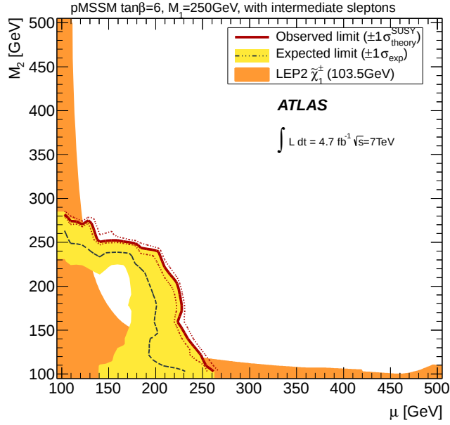
(c) M_1 = 250 \text{ GeV}
