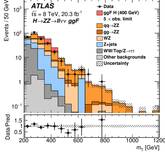
Figure 2: The distribution used in the likelihood fit of the transverse mass m_T^{ZZ} reconstructed from the momentum of the dilepton system and the missing transverse momentum for the H \rightarrow ZZ \rightarrow \ell^+ \ell^- \nu \bar{\nu} search in the ggF channel. The simulated signal is normalized to a cross-section corresponding to five times the observed limit given in Section 11. The contribution labelled as ‘Top’ includes both the t\bar{t} and single-top processes. The bottom pane shows the ratio of the observed data to the predicted background.
