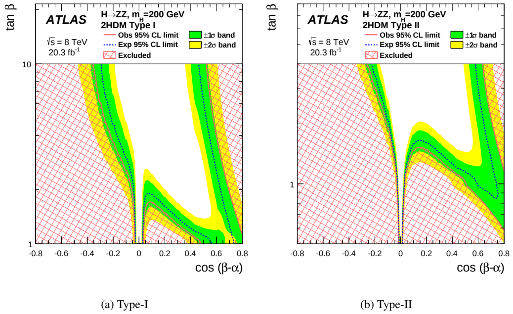
Figure 13: 95% CL exclusion contours in the 2HDM (a) Type-I and (b) Type-II models for m_H = 200 GeV, shown as a function of the parameters \cos(\beta - \alpha) and \tan\beta . The red hashed area shows the observed exclusion, with the solid red line denoting the edge of the excluded region. The dashed blue line represents the expected exclusion contour and the shaded bands the 1\text{-}\sigma and 2\text{-}\sigma uncertainties on the expectation. The vertical axis range is set such that regions where the light Higgs couplings are enhanced by more than a factor of three from their SM values are avoided.
