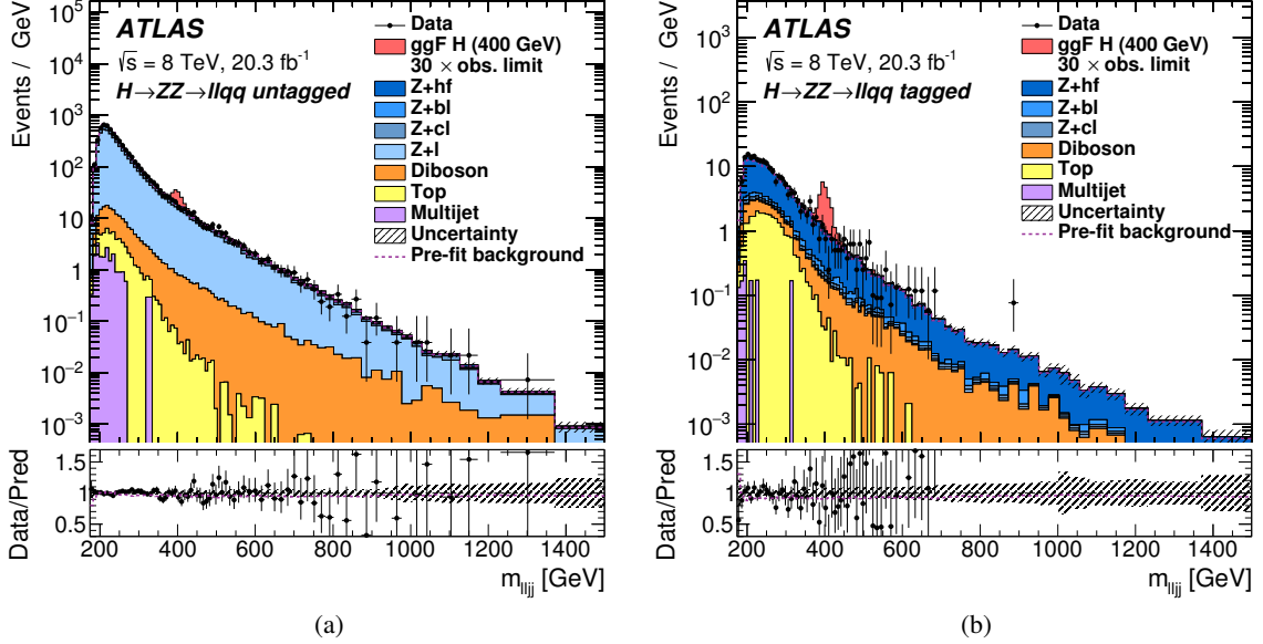
Figure 3: The distributions used in the likelihood fit of the invariant mass of dilepton+dijet system m_{\ell\ell jj} for the H \rightarrow ZZ \rightarrow \ell^+ \ell^- q\bar{q} search in the (a) untagged and (b) tagged resolved ggF subchannels. The dashed line shows the total background used as input to the fit. The simulated signal is normalized to a cross-section corresponding to thirty times the observed limit given in Section 11. The contribution labelled as ‘Top’ includes both the t\bar{t} and single-top processes. The bottom panes show the ratio of the observed data to the predicted background.
