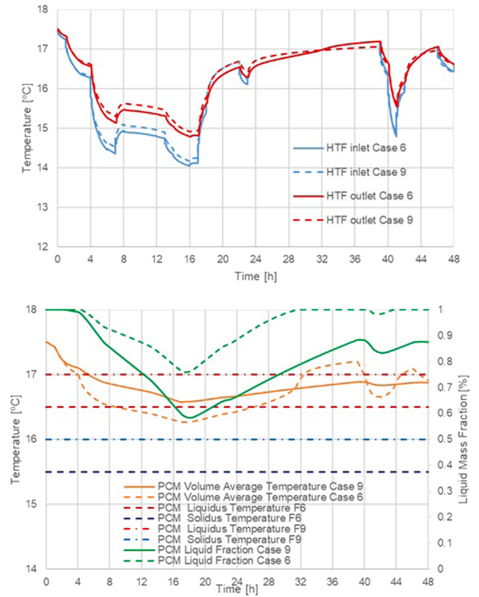
Fig. 11. Comparison of the inlet and outlet temperatures of the HTF and PCM volume average temperature and liquid mass fraction for cases 6 and 9.
