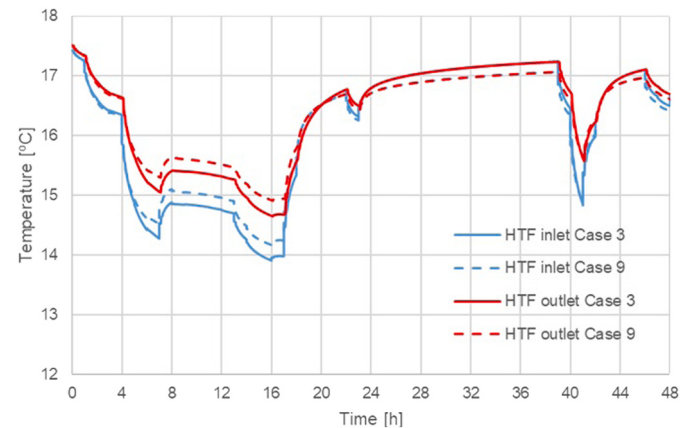
Fig. 12. Comparison of the inlet and outlet temperatures of the HTF for cases 3 and 9.
