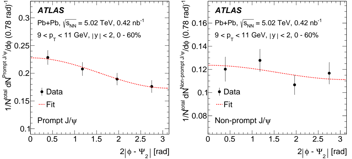
Figure 2: The azimuthal distribution of prompt (left) and non-prompt (right) J/\psi yields for the lowest p_T bin studied. The yields are normalised by the inclusive J/\psi signal and the error bars are fit uncertainties associated with the signal extraction. The dotted red line is the result of the simultaneous fit used to compute v_2 .
