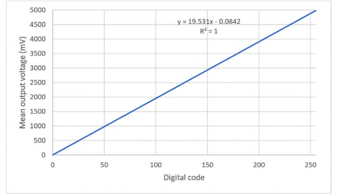
Fig. 9. Static characteristic.
