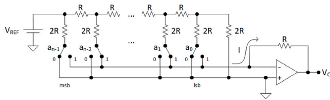
Fig. 2. R-2R ladder network.
