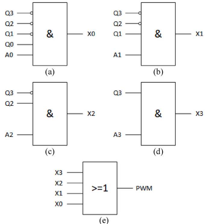
Fig. 7. Pulse filtering from the LSB ( X_0 ) to the MSB ( X_3 ) followed by adding (OR gate).
