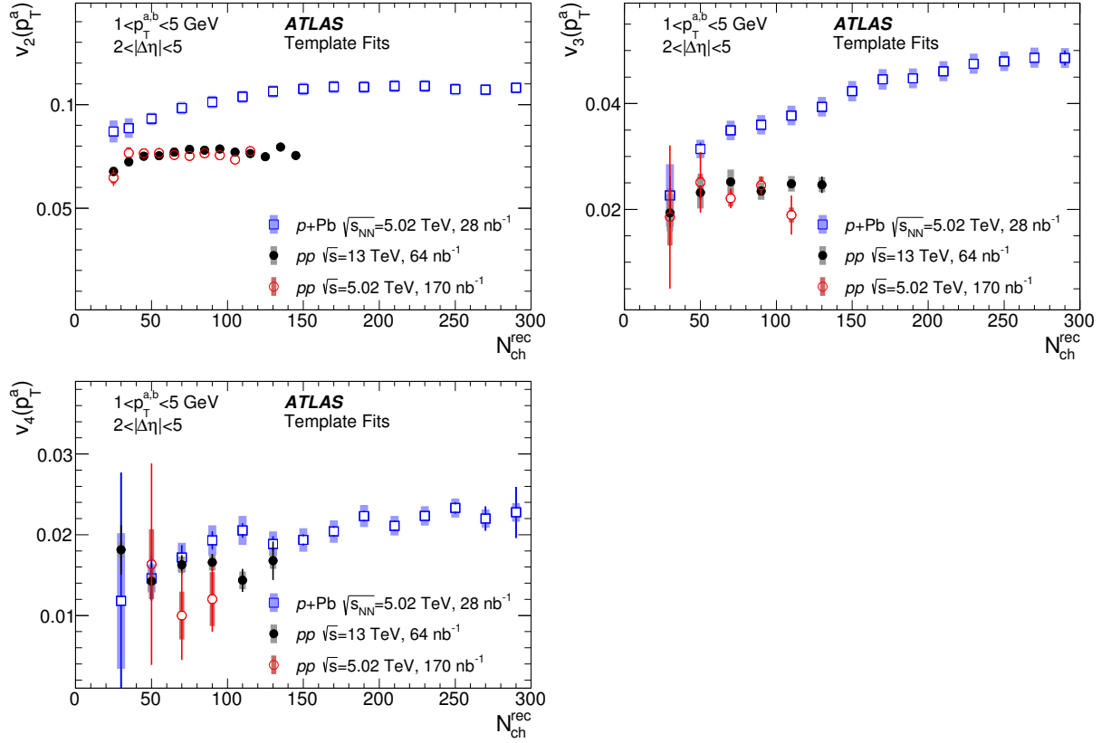
Figure 18: Comparison of the v_n obtained from the template fitting procedure in the 13 TeV pp , 5.02 TeV pp , and 5.02 TeV p +Pb data, as a function of N_{\text{ch}}^{\text{rec}} . The results are for 1 < p_{\text{T}}^{a,b} < 5 GeV. The three panels correspond to n=2, 3 and 4 . The error bars and shaded bands indicate statistical and systematic uncertainties, respectively.
