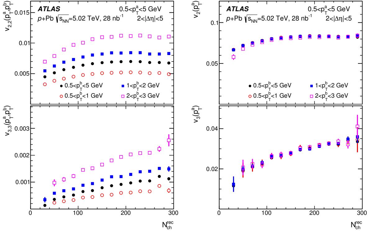
Figure 10: The left panels show v_{2,2} (top) and v_{3,3} (bottom) as a function of N_{\text{ch}}^{\text{rec}} in the 5.02 TeV p+\text{Pb} data, for 0.5 < p_T^a < 5 GeV and for different choices of the p_T^b interval. The right panels show the corresponding v_2 (top) and v_3 (bottom) values obtained using Eq. (4). The error bars indicate statistical uncertainties only.
