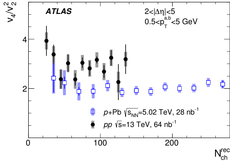
Figure 19: Ratio of v_4 to v_2^2 as a function of N_{\text{ch}}^{\text{rec}} in the 13 TeV pp and 5.02 TeV p +Pb data. The results are for 0.5 < p_{\text{T}}^{a,b} < 5 GeV. The error bars and shaded bands indicate statistical and systematic uncertainties, respectively.
