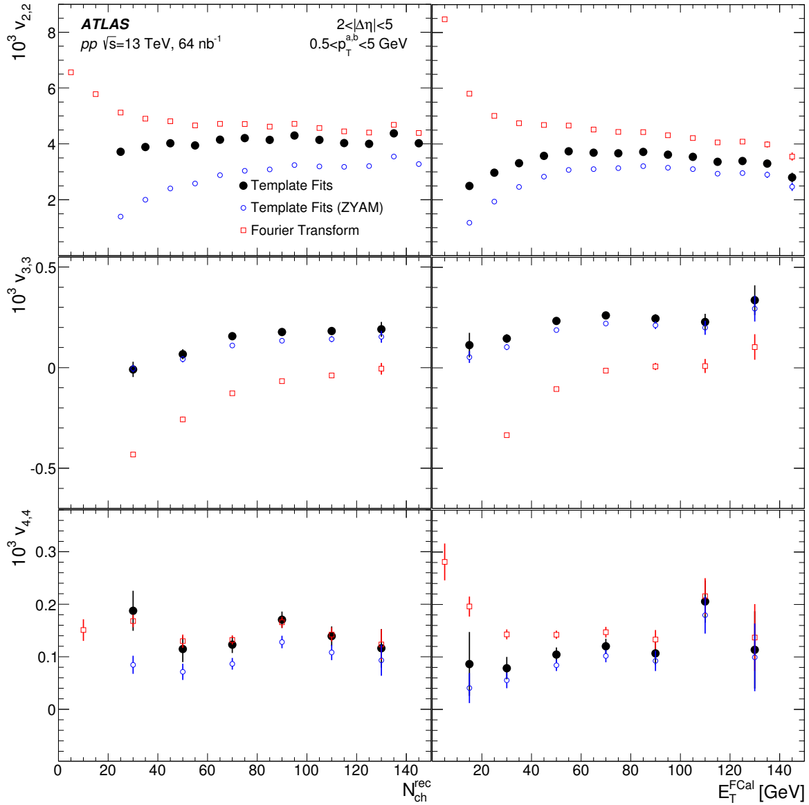
Figure 6: The v_{n,n} obtained from the template fitting procedure in the 13 TeV pp data, as a function of N_{ch}^{rec} (left panels), and as a function of E_T^{FCal} (right panels). The top, middle and bottom panels correspond to v_{2,2} , v_{3,3} , and v_{4,4} , respectively. The results are for 0.5 < p_T^{a,b} < 5 GeV. The error bars indicate statistical uncertainties. The v_{n,n} obtained from a direct Fourier transform of Y(\Delta\phi) and from the ZYAM-based template fits are also shown for comparison.
