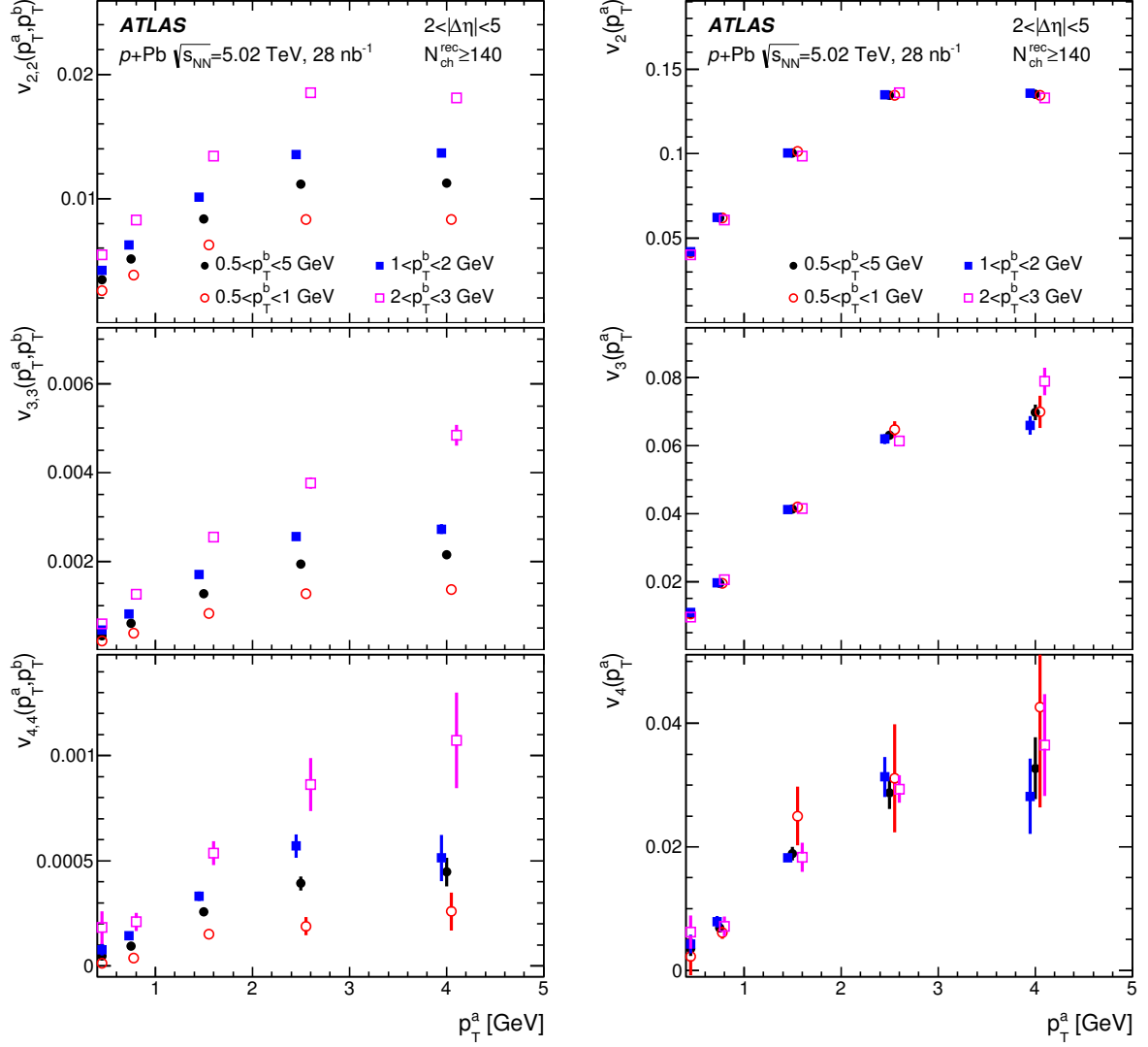
Figure 12: The left panels show the v_{n,n} as a function of p_T^a in the 5.02 TeV p +Pb data, for N_{ch}^{rec} \geq 140 and for different choices of the p_T^b interval. From top to bottom, the three rows correspond to n=2, 3 and 4 . The right panels show the corresponding v_n values obtained using Eq. (4). The error bars indicate statistical uncertainties only. The p_T^a intervals plotted are 0.4–0.5, 0.5–1, 1–2, 2–3 and 3–5 GeV. In some cases, the data points have been slightly shifted along the x -axis, for clarity.
