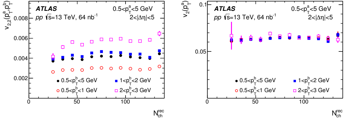
Figure 9: The left panel shows v_{2,2} as a function of N_{ch}^{rec} in the 13 TeV pp data, for 0.5 < p_T^a < 5 \text{ GeV} and for different choices of the p_T^b interval. The right panel shows the corresponding v_2 values obtained using Eq. (4). The error bars indicate statistical uncertainties only.
