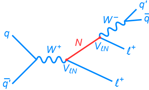
Figure 1: The lowest-order Feynman diagram for production of a heavy Majorana neutrino N . The charge-conjugate diagram also contributes and results in a \ell^-\ell^-\bar{q}\bar{q}' final state.
