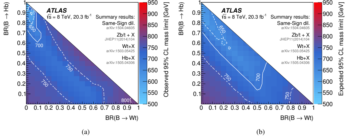
Figure 25: Summary of the most restrictive (a) observed and (b) expected limit (95% CL) on the mass of the B quark in the plane of \text{BR}(B \rightarrow Hb) versus \text{BR}(B \rightarrow Wt) from all ATLAS searches for B\bar{B} production (see text for details). Contour lines are provided to guide the eye.
