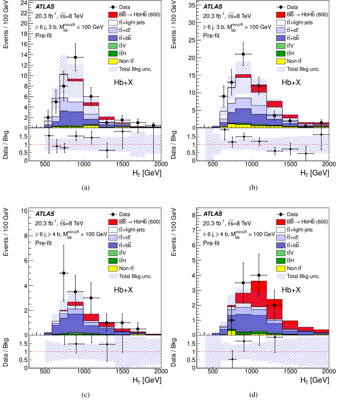
Figure 13: B\bar{B} \rightarrow Hb\bar{H}\bar{b} search: comparison between data and prediction for the distribution of the scalar sum ( H_T ) of the transverse momenta of the lepton, the selected jets and the missing transverse momentum in each of the analysed channels after final selection: (a) ( \geq 6 j, 3 b, low M_{bb}^{\text{min}\Delta R} ), (b) ( \geq 6 j, 3 b, high M_{bb}^{\text{min}\Delta R} ), (c) ( \geq 6 j, \geq 4 b, low M_{bb}^{\text{min}\Delta R} ), and (d) ( \geq 6 j, \geq 4 b, high M_{bb}^{\text{min}\Delta R} ). The background prediction is shown before the fit to data. The contributions from W/Z +jets, single top, diboson and multijet backgrounds are combined into a single background source referred to as “Non- t\bar{t} ”. Also shown is the expected signal contribution from a vector-like B quark with mass m_B = 600 GeV under the assumption \text{BR}(B \rightarrow Hb) = 1 . The last bin in all figures contains the overflow. The bottom panel displays the ratio of data to the total background prediction. The hashed area represents the total uncertainty on the background.
