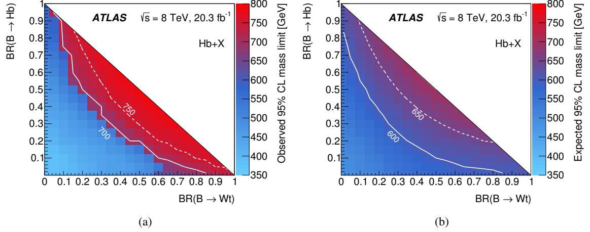
Figure 24: (a) Observed and (b) expected limit (95% CL) on the mass of the B quark in the plane of \text{BR}(B \rightarrow Hb) versus \text{BR}(B \rightarrow Wt) for the B\bar{B} \rightarrow Hb+X search. Contour lines are provided to guide the eye.
