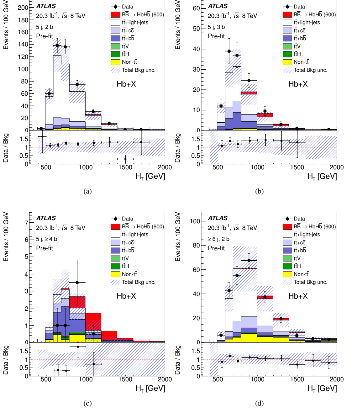
Figure 12: B\bar{B} \rightarrow HbH\bar{b} search: comparison between data and prediction for the distribution of the scalar sum ( H_T ) of the transverse momenta of the lepton, the selected jets and the missing transverse momentum in each of the analysed channels after final selection: a) (5 j, 2 b), (b) (5 j, 3 b), (c) (5 j, \geq 4 b), and (d) ( \geq 6 j, 2 b). The background prediction is shown before the fit to data. The contributions from W/Z +jets, single top, diboson and multijet backgrounds are combined into a single background source referred to as “Non- t\bar{t} ”. Also shown is the expected signal contribution from a vector-like B quark with mass m_B = 600 GeV under the assumption \text{BR}(B \rightarrow Hb) = 1 . The last bin in all figures contains the overflow. The bottom panel displays the ratio of data to the total background prediction. The hashed area represents the total uncertainty on the background.
