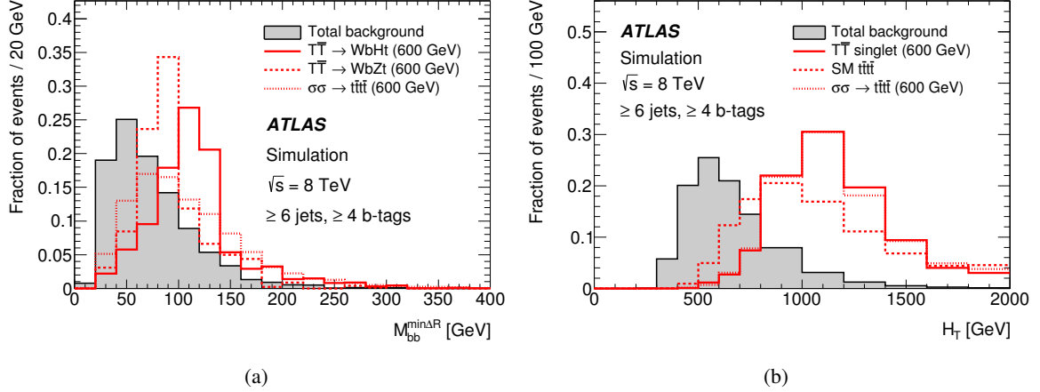
Figure 8: T\bar{T} \rightarrow Ht+X search (simulated events): comparison of the distributions of (a) the invariant mass of the two b -tagged jets with lowest \Delta R separation ( M_{bb}^{\min\Delta R} ), and (b) the scalar sum of the transverse momenta of the lepton, the selected jets and the missing transverse momentum ( H_T ), between the total background (shaded histogram) and several signal scenarios considered in this search: T\bar{T} \rightarrow WbHt (red solid histogram), T\bar{T} \rightarrow WbZt or SM t\bar{t}t\bar{t} production (red dashed histograms), and sgluon pair production giving a t\bar{t}t\bar{t} final state (red dotted histogram). A mass of 600 GeV is assumed for the T quark and the sgluon. The selection used in both (a) and (b) corresponds to events satisfying the preselection requirements and with \geq 6 jets and \geq 4 b -tagged jets.
