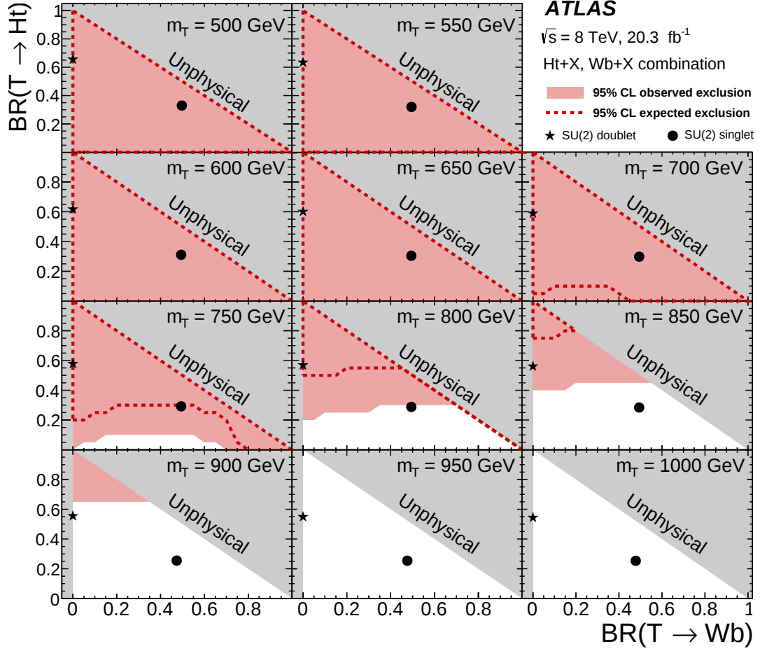
Figure 19: Observed (red filled area) and expected (red dashed line) 95% CL exclusion in the plane of \text{BR}(T \rightarrow Wb) versus \text{BR}(T \rightarrow Ht) from the combination of the T\bar{T} \rightarrow Wb+X and T\bar{T} \rightarrow Ht+X searches, for different values of the vector-like T quark mass. The grey (dark shaded) area corresponds to the unphysical region where the sum of branching ratios exceeds unity. The default branching ratio values from the PROPOS event generator for the weak-isospin singlet and doublet cases are shown as plain circle and star symbols respectively.
