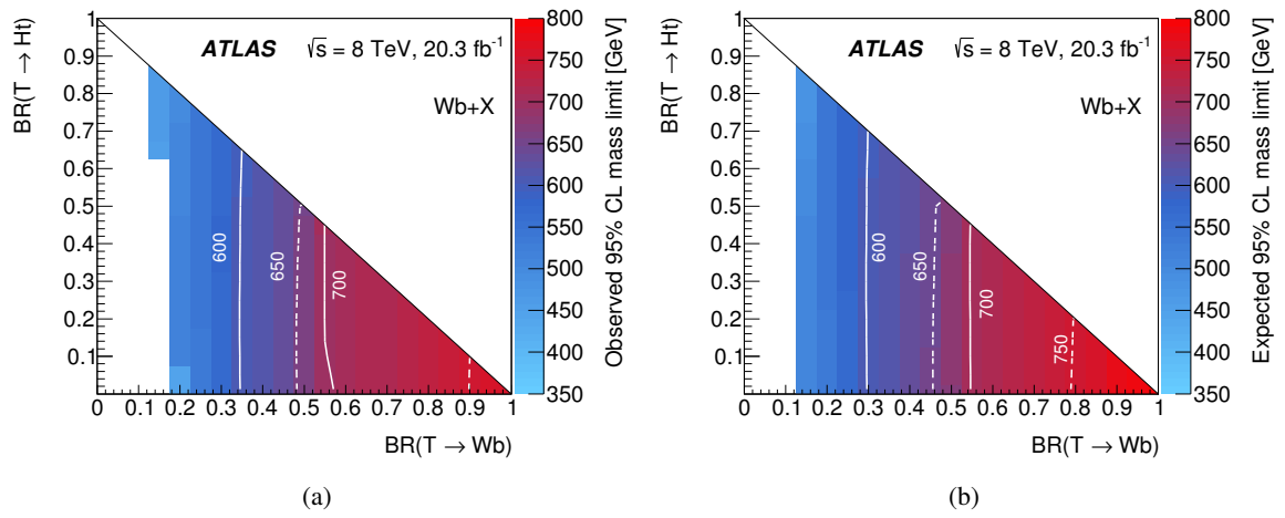
Figure 31: (a) Observed and (b) expected limit (95% CL) on the mass of the T quark in the plane of BR(T \rightarrow Ht) versus BR(T \rightarrow Wb) for the T\bar{T} \rightarrow Wb+X search. Contour lines are provided to guide the eye. The region shown in white is not excluded for any values of the T quark mass probed.
