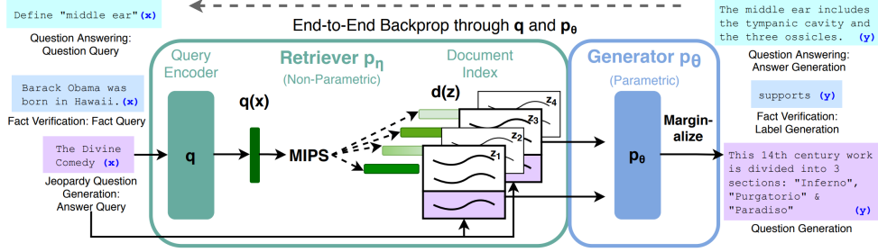
Figure 8: RAG implementation overview[35]
