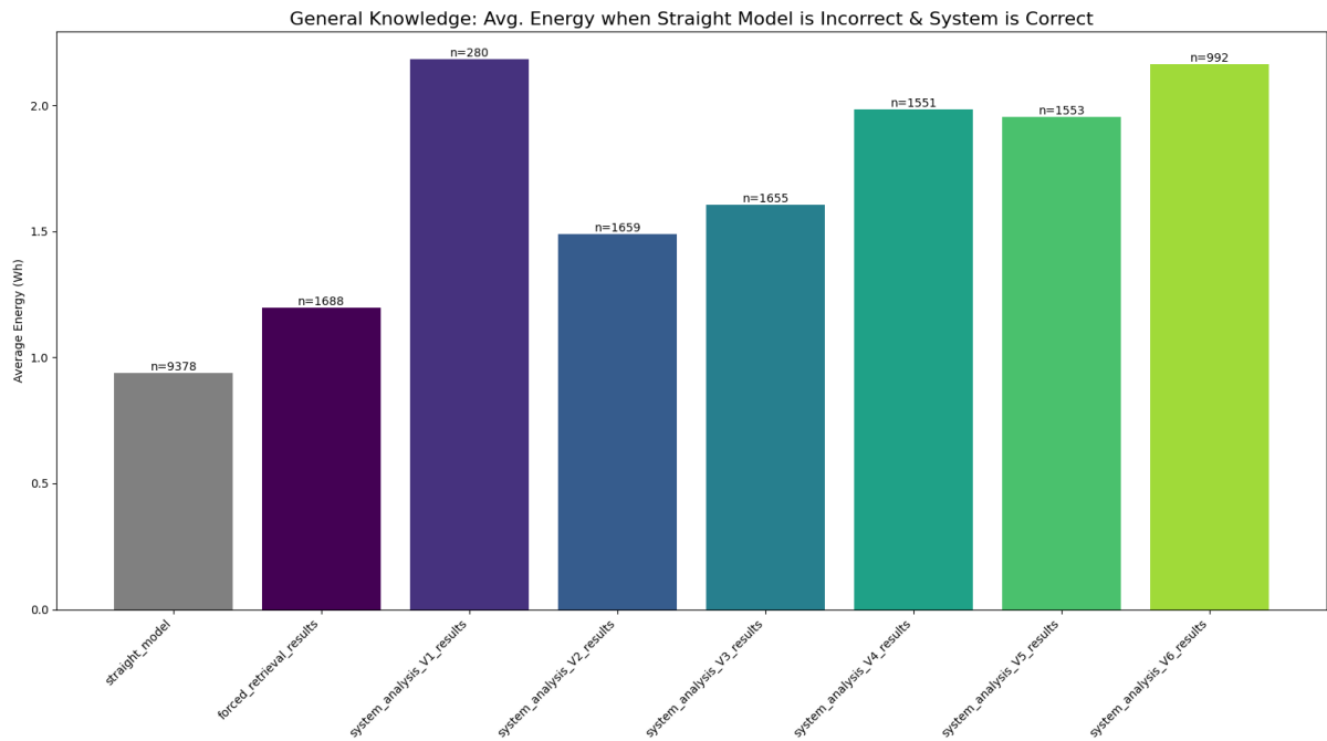
Figure 49: General Knowledge: Avg. Energy when Straight Model is Incorrect & System is Correct
