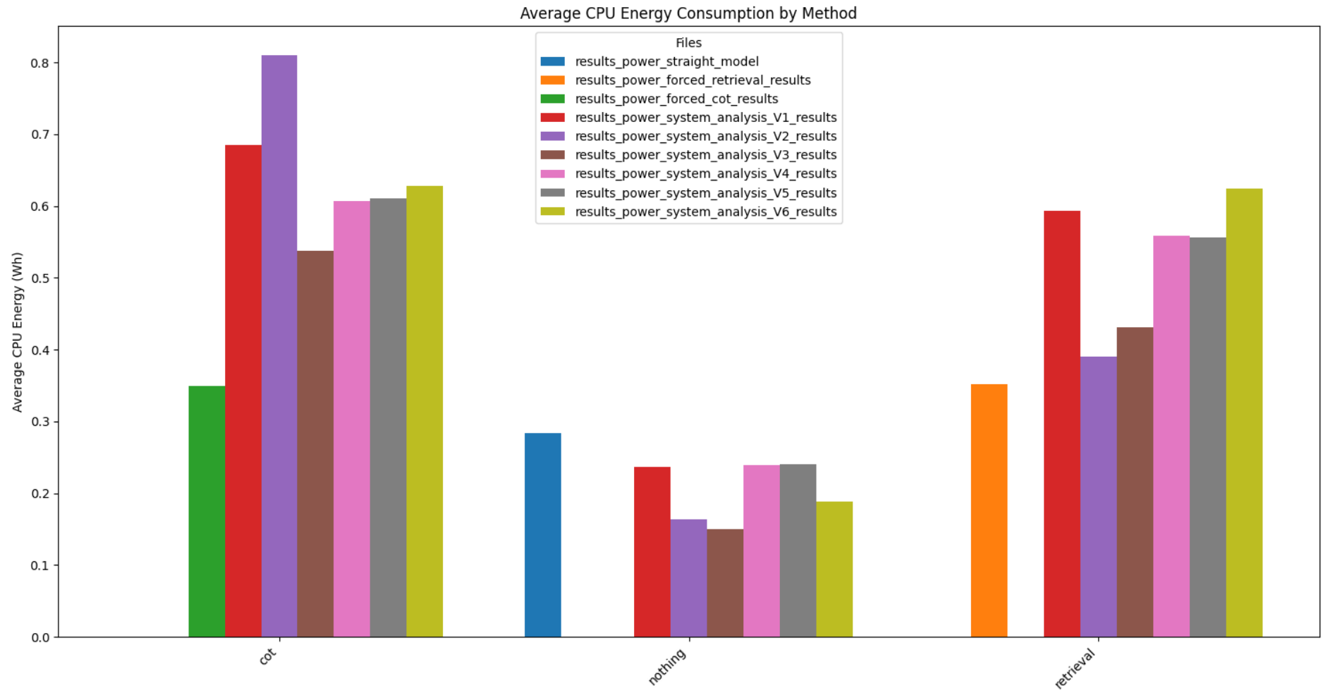
Figure 61: Average CPU Energy Consumption by Method.
