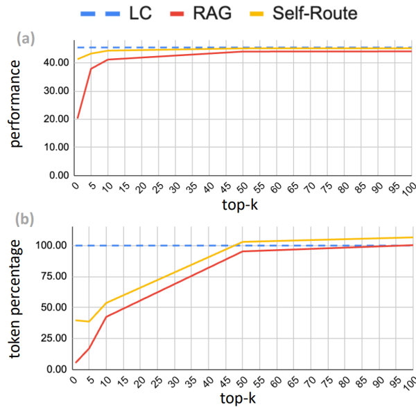
Figure 13: Trade-off curves between (a) model performance and (b) token percentage as a function of k . [45]
