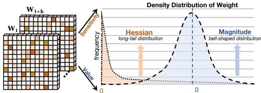
Figure 3: The Hessian metrics (sensitivity) and magnitude (value) of weights in LLMs. The weights of different layers in LLMs are characterized by bell-shaped distribution, accompanied by a few salient values.[24]
