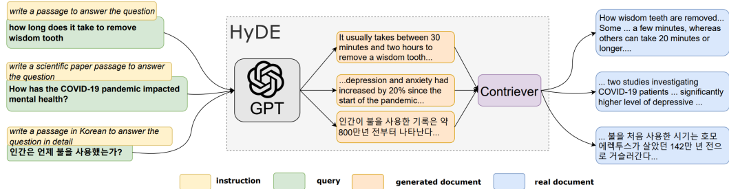
Figure 9: An illustration of the HyDE model.[40]
