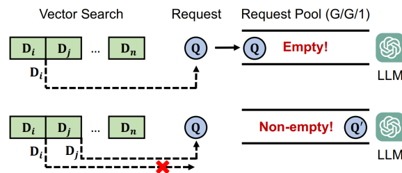
Figure 19: Optimal speculative pipelining strategy [44]
