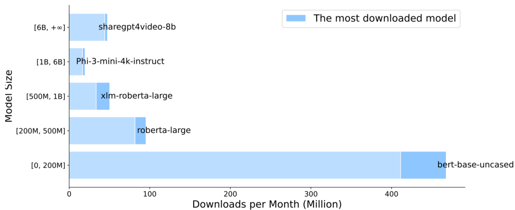
Figure 25: Relationship between model size and monthly downloads[68]
