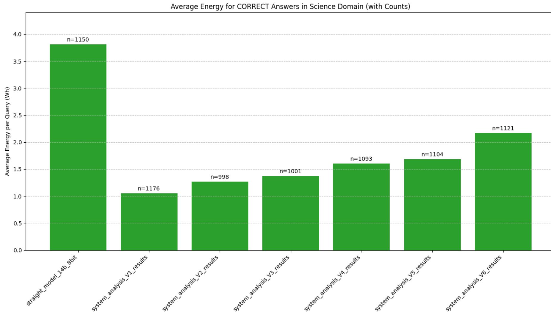
Figure 68: Average Energy for CORRECT Answers in Science Domain (with Counts).
