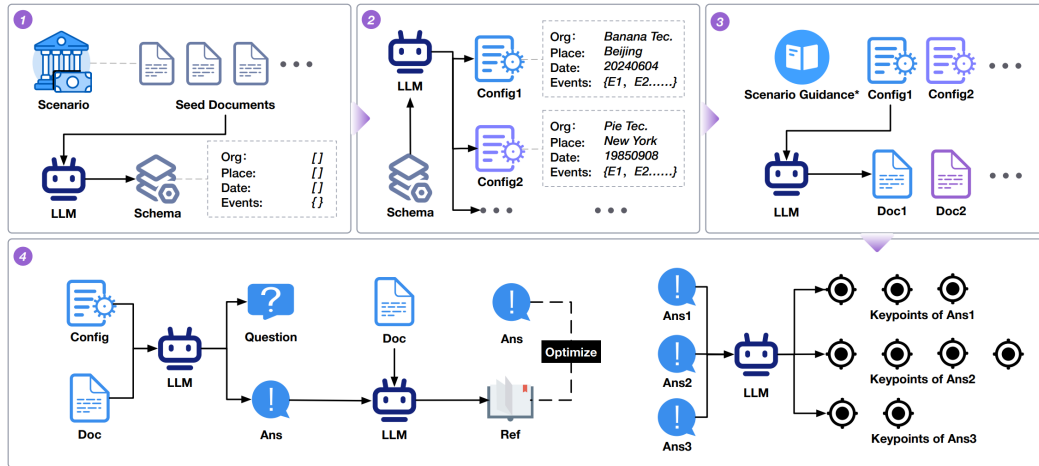
Figure 24: RAGEval System: 1 summarizing a schema containing specific knowledge from seed documents. 2 filling in factual information based on this schema to generate diverse configurations. 3 generating documents according to the configurations. 4 creating evaluation data composed of questions, answers, and references derived from the configurations and documents.[65]
