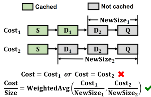
Figure 16: Cost estimation PGDSF[44]
