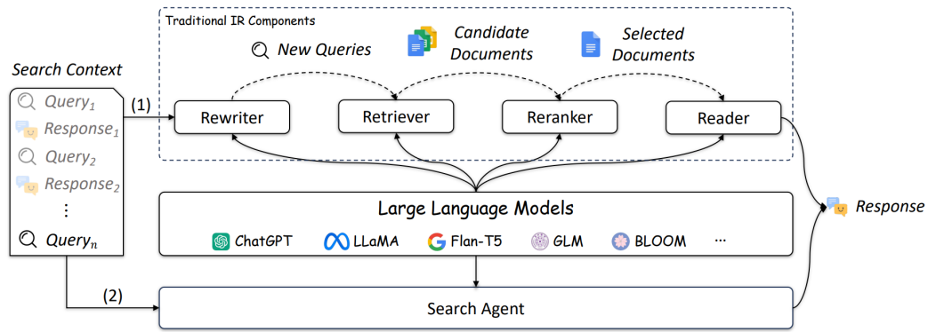
Figure 26: Traditional information retrieval architecture[68]
