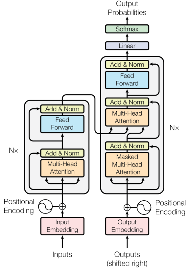
Figure 1: Transformer model architecture [5]
