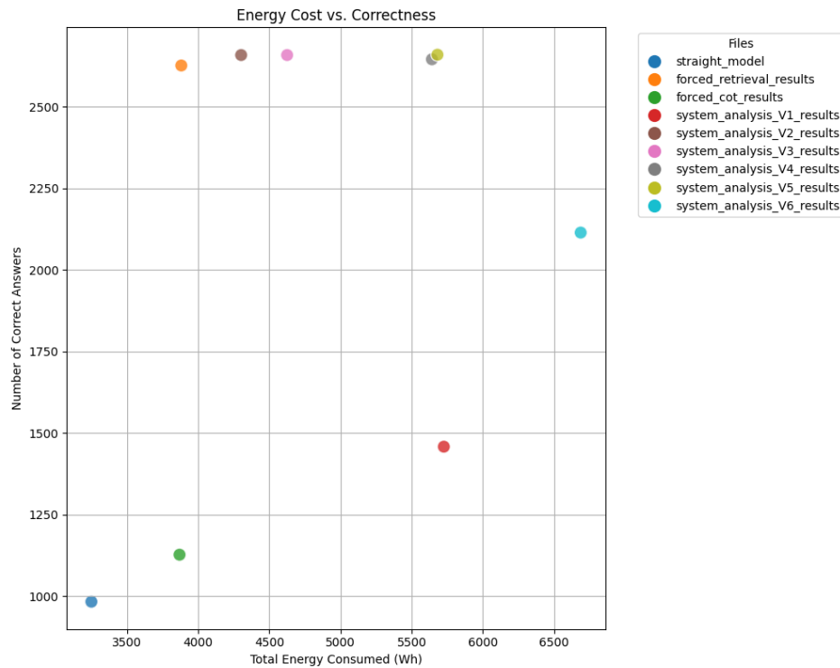
Figure 42: Energy Costs vs. Correctness Scatterplot
