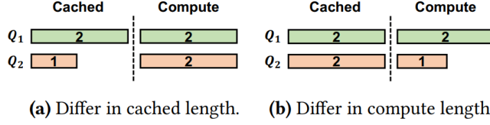
Figure 17: Cache aware Reordering[44]
