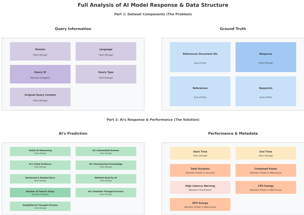
Figure 29: Jsonl Data Structure
