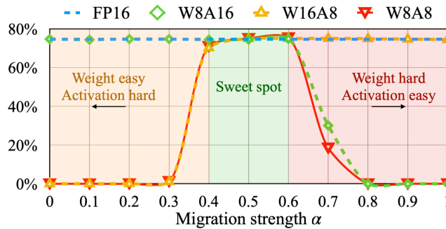
Figure 6: Finding the sweet spot for the migration strength[29]
