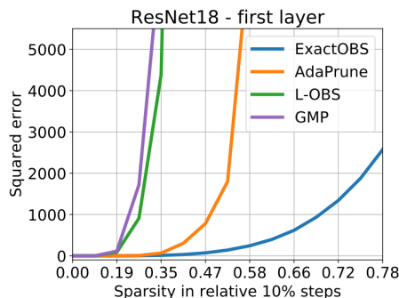
Figure 2: RN18 squared error. [21]
