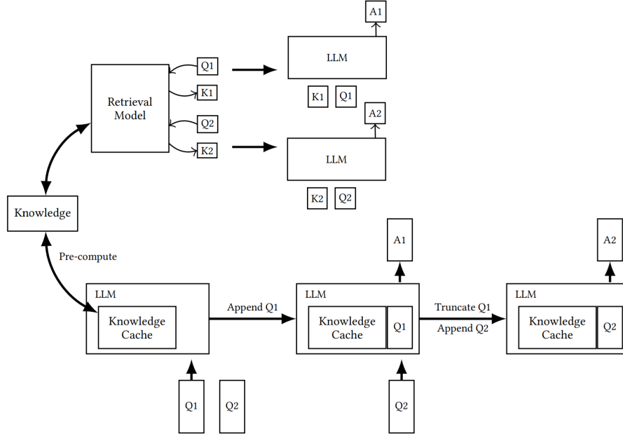
Figure 10: Comparison RAG on the top and CAG on the bottom [43]
