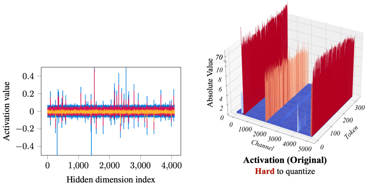
(a) The distributions of activations at the input to the FFN block in LLAMA2-7B model[28]
