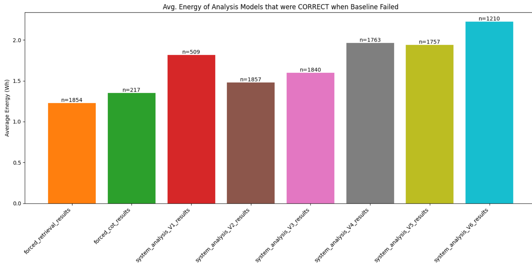
Figure 59: Avg. Energy of Analysis Models that were CORRECT when Baseline Failed.
