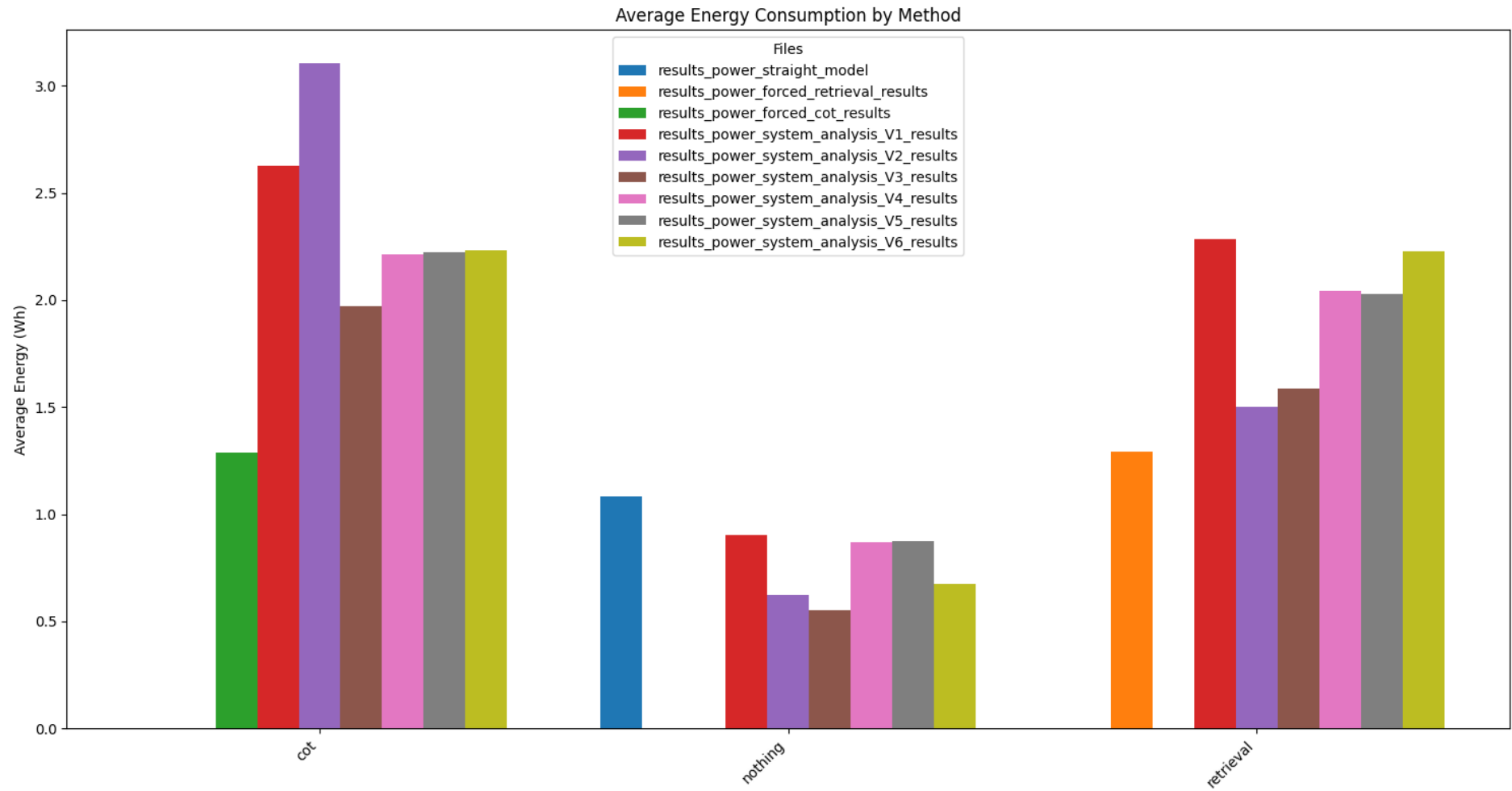
Figure 64: Average Energy Consumption by Method.
