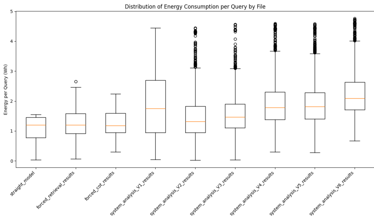
Figure 52: Distribution of Energy Consumption per Query by File
