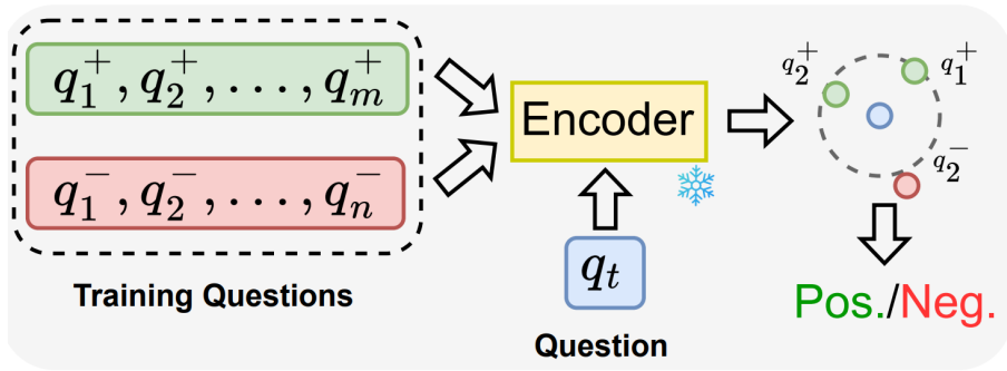
Figure 23: k -nearest-neighbor to understand model knowledge [52]
