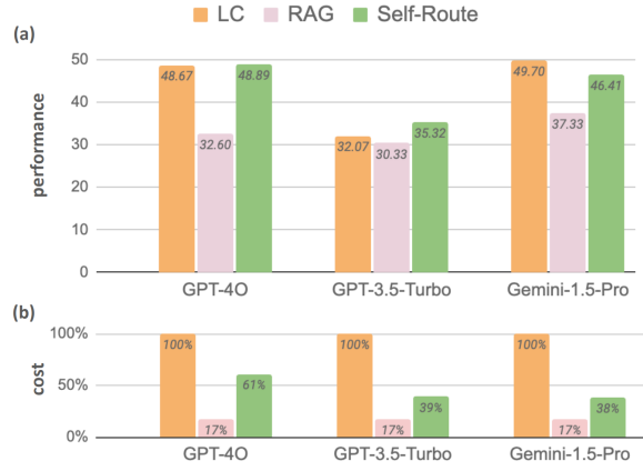
Figure 11: Comparison between performance and costs on multiple models using LC, RAG and Self-Route[45]
