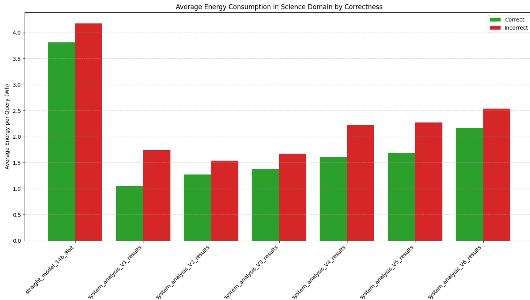
Figure 67: Average Energy Consumption in Science Domain by Correctness.
