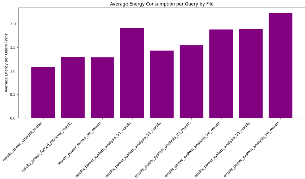
Figure 46: Average Energy Consumption per Query by File
