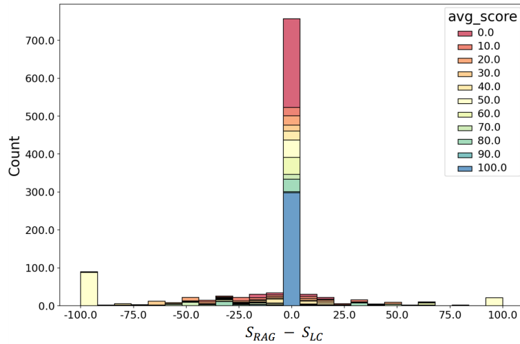
Figure 12: Distribution of the difference of prediction scores between RAG and LC[45]
