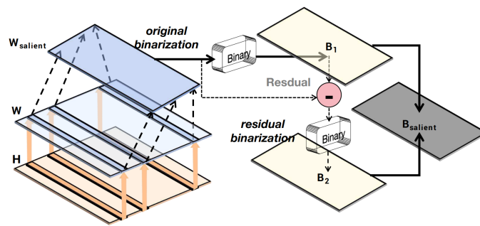
Figure 4: Illustration of salient weight binarization. The B1 binarized from salient weight is made into a residual with the original value and then binarized again to obtain B2.[24]
