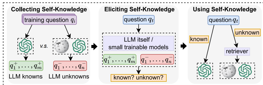
Figure 20: The SKR Pipeline and its component interactions.[52]
