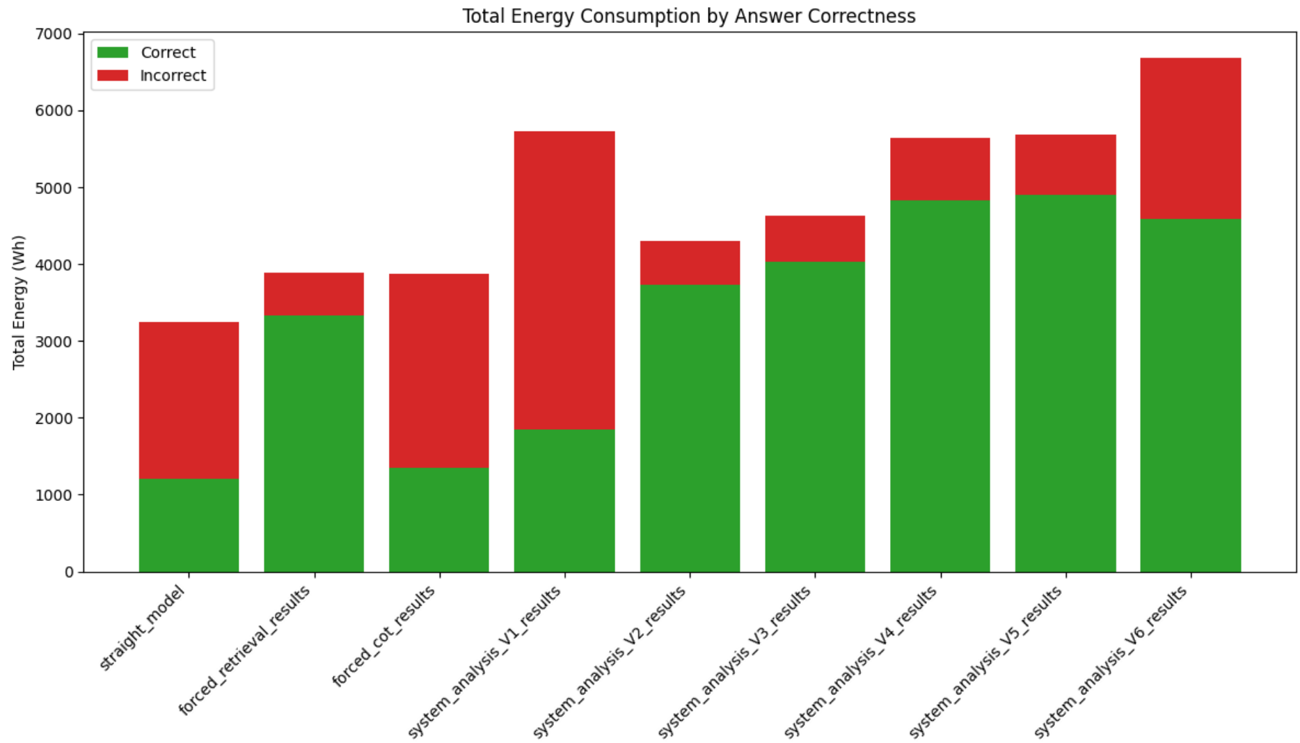
Figure 66: Total Energy Consumption by Answer.
