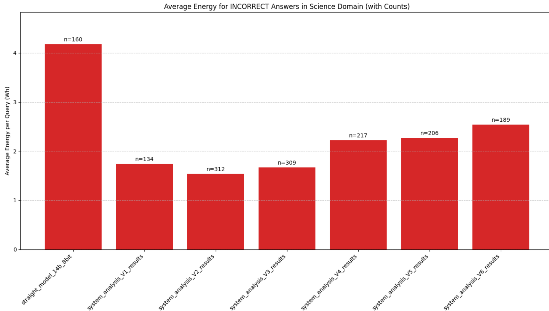
Figure 70: Average Energy for INCORRECT Answers in Science Domain (with Counts).
