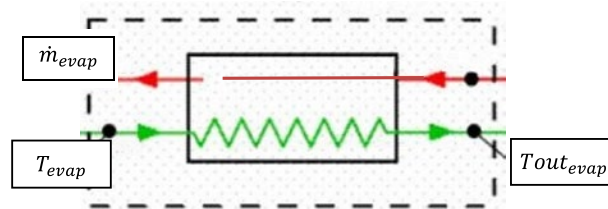
Figure 4. Evaporator: control volume.
