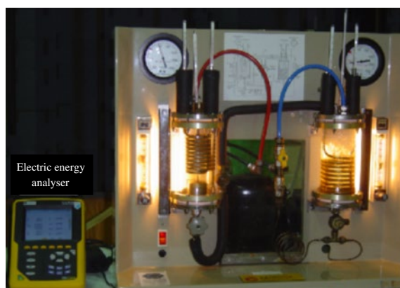
Figure 1. Refrigeration cycle.
