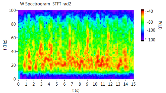
Fig. 7. Doppler radar spectrograms for leg swing during walker usage after wavelets based signal processing
