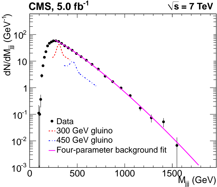
Figure 2: Mass distribution for selected jet triplets. The four-parameter background fit is shown by the solid line. The NLO expectation for a 300 GeV gluino signal is shown by the dotted line, and that of a 450 GeV gluino signal by the dash-dotted line. Each of the two is normalized to the integrated luminosity of the data sample.
