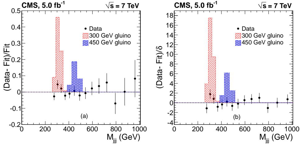
Figure 3: Difference between the measured triplet mass distribution and the fitted background parametrization, divided by the fitted value (a) or by the statistical uncertainty \delta on the fitted value (b), shown for both data and the NLO expectation of two gluino models, one with a gluino mass of 300 GeV and the other with a gluino mass of 450 GeV.
