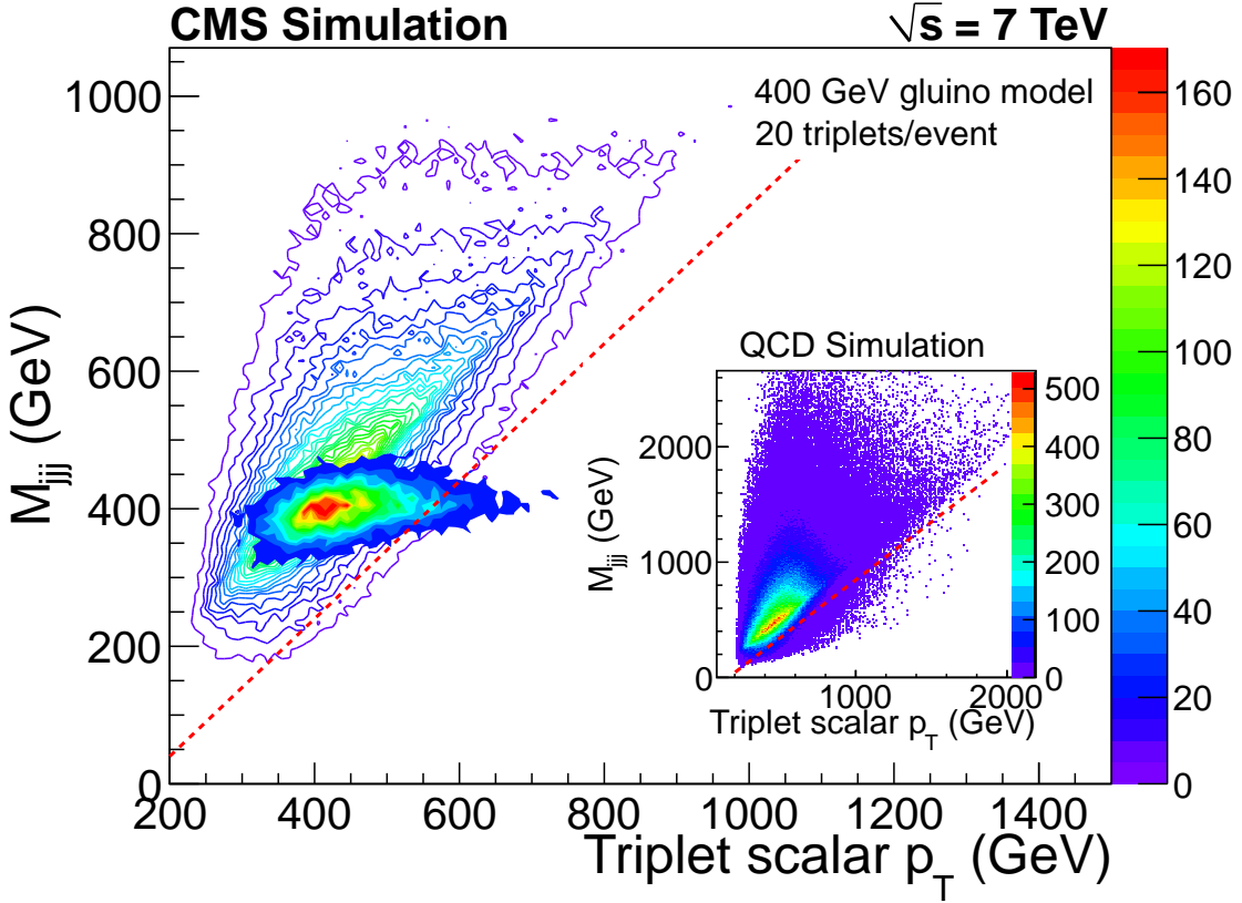
Figure 1: Simulated triplet jet mass M_{jjj} versus the triplet scalar p_T of all 20 triplets for a gluino mass of 400 GeV, shown as a contoured distribution, with that of the triplets whose jets all originate from the same gluino parent overlaid. The overlaid “correct” triplets are shown to lie along a horizontal line corresponding to the generated gluino mass, while the behavior of all other triplets resembles the expectation for the QCD background, which is shown in the inset. All triplets falling to the right of the dashed line pass the requirement of Eq. (1) for a value of \Delta = 160 GeV.
