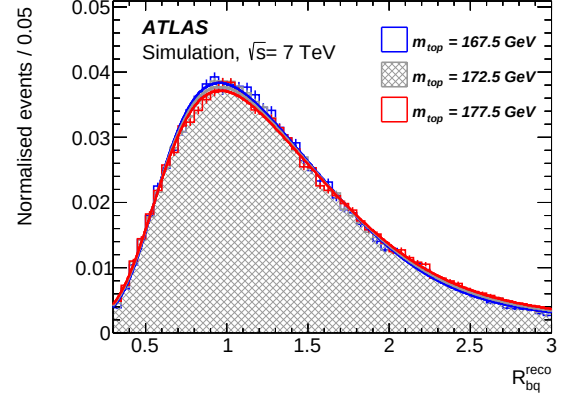
(b) R_{bq}^{\text{reco}} , at least two b -tagged jets
