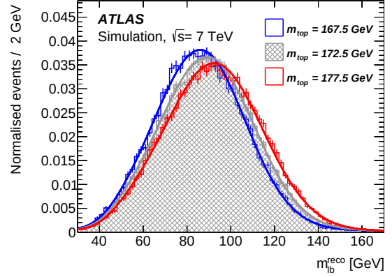
(b) m_{\ell b}^{\text{reco}} , exactly two b -tagged jets
