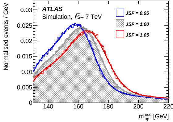
(c) m_{\text{top}}^{\text{reco}} , at least two b -tagged jets
