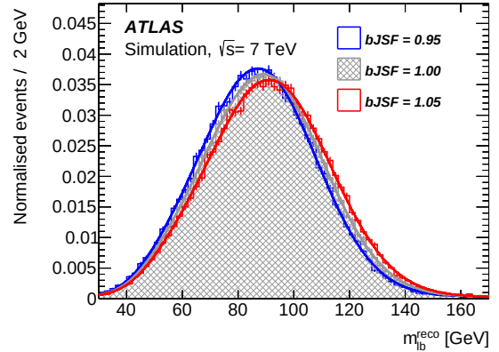
(f) m_{\ell b}^{\text{reco}} , exactly two b -tagged jets
