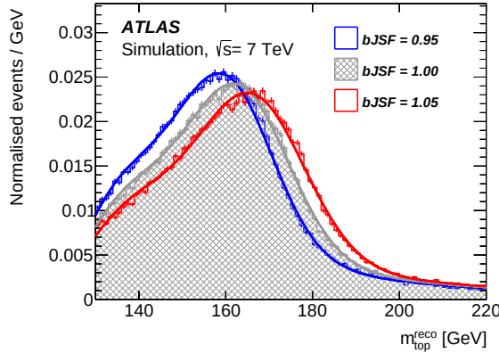
(e) m_{\text{top}}^{\text{reco}} , at least two b -tagged jets
