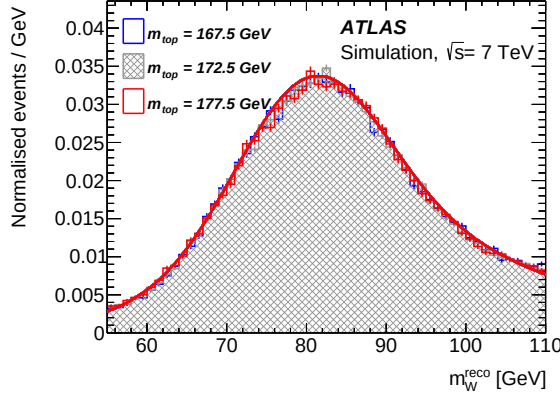
(a) m_W^{\text{reco}} , at least two b -tagged jets
