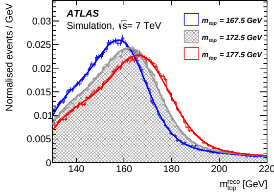
(a) m_{\text{top}}^{\text{reco}} , at least two b -tagged jets
