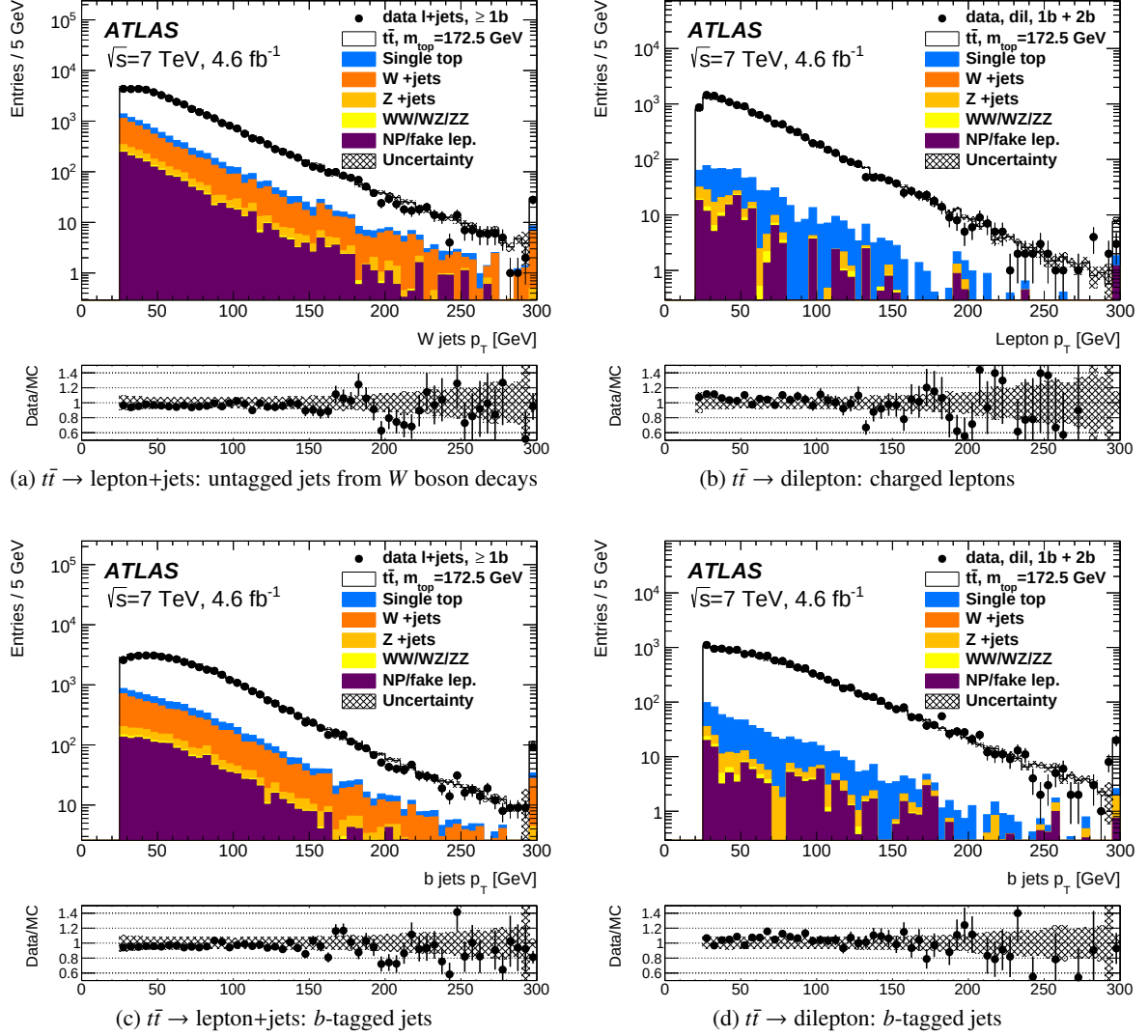
Figure 1: Distributions of the transverse momentum of the untagged and b -tagged jets in the t\bar{t} \rightarrow lepton+jets analysis (a, c) and of the charged lepton and b -tagged jets p_T in the t\bar{t} \rightarrow dilepton analysis (b, d). The data are shown by the points and the signal-plus-background prediction by the solid histogram. The hatched area is the combined uncertainty on the prediction described in Sect. 4.3.3, and the rightmost bin contains the overflow if present. For each figure, the ratio of the data to the MC prediction is also presented.
