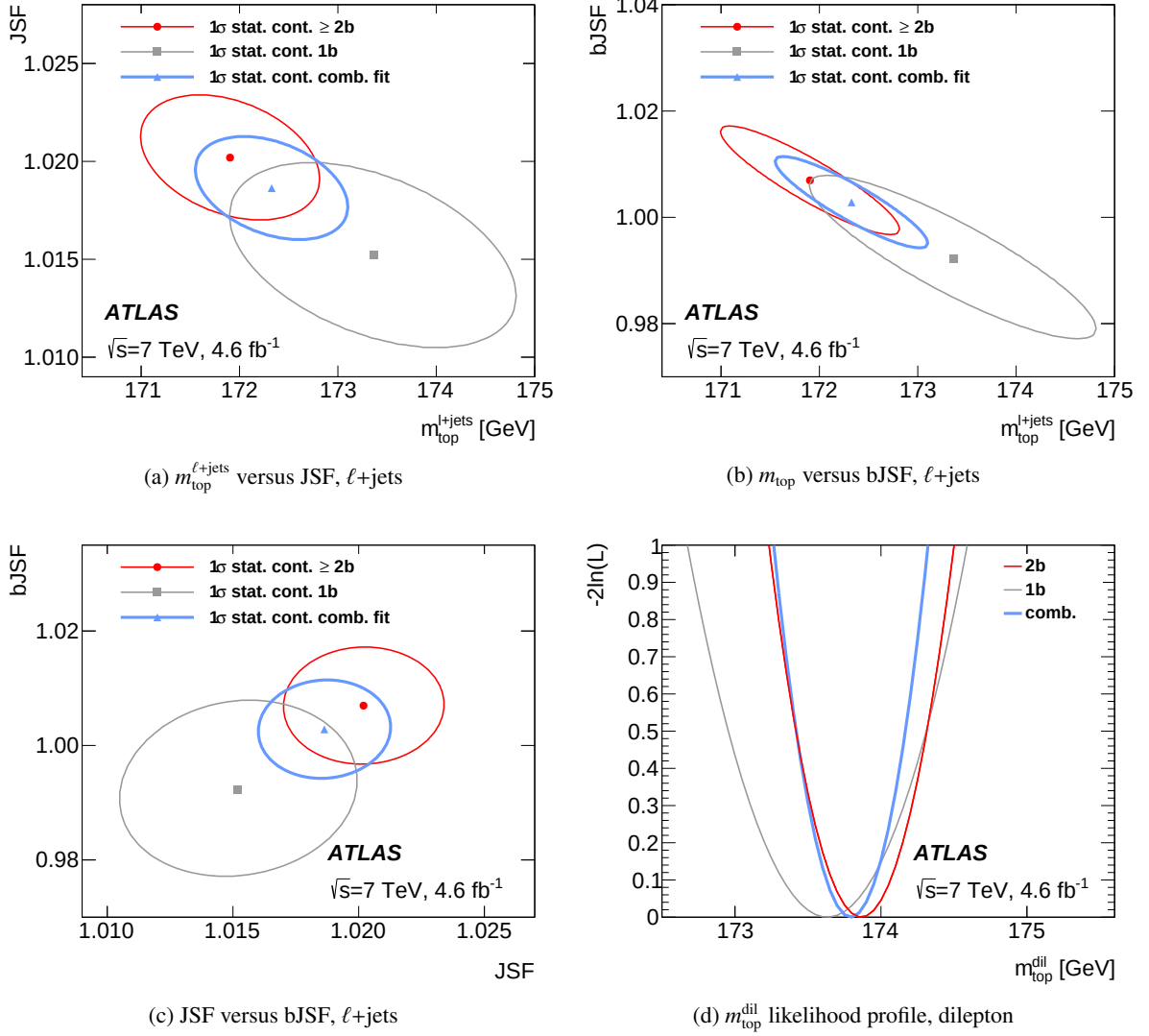
Figure 5: Likelihood contours showing the correlation determined in data of the measured m_{\text{top}}^{\ell+\text{jets}} to (a) the JSF and (b) the bJSF, and (c) the correlation of the two scales JSF and bJSF, within the t\bar{t} \rightarrow \text{lepton} + \text{jets} analysis. Figures (a-c) show the results using the events with one b -tagged jet only (grey ellipses), with at least two b -tagged jets (red ellipses) and finally with all selected events, i.e. the ones with at least one b -tagged jet (blue ellipses). The ellipses correspond to the \pm 1\sigma (statistical) uncertainties, including the statistical components from the JSF and bJSF determination. While tracing the contours the additional parameters of the likelihood are fixed to their best fit values. Figure (d) reports the likelihood profile as a function of m_{\text{top}}^{\text{dil}} for the sample with one b -tagged jet, the sample with two b -tagged jets and the combined result. The colour coding is analogous to figures (a-c).
