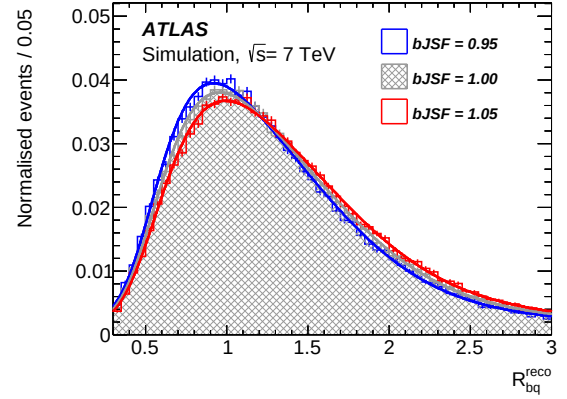
(f) R_{bq}^{\text{reco}} , at least two b -tagged jets
