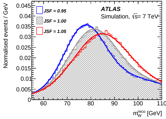
(c) m_W^{\text{reco}} , at least two b -tagged jets
