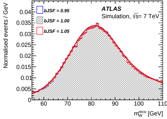
(e) m_W^{\text{reco}} , at least two b -tagged jets
