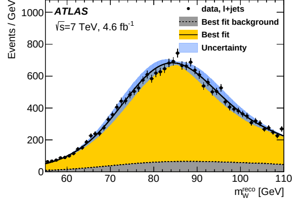
(b) m_W^{\text{reco}}, \ell+\text{jets}
