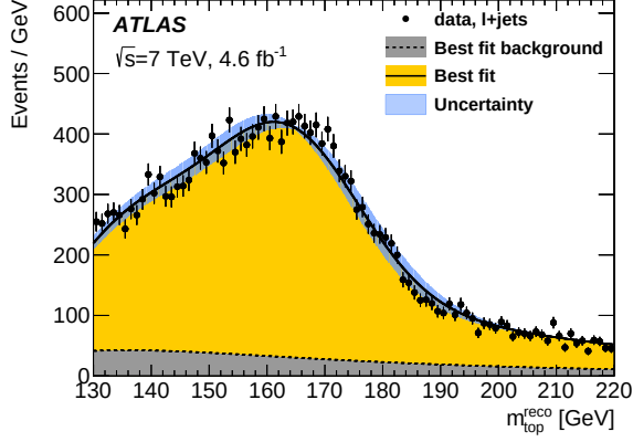
(a) m_{\text{top}}^{\text{reco}}, \ell+\text{jets}
