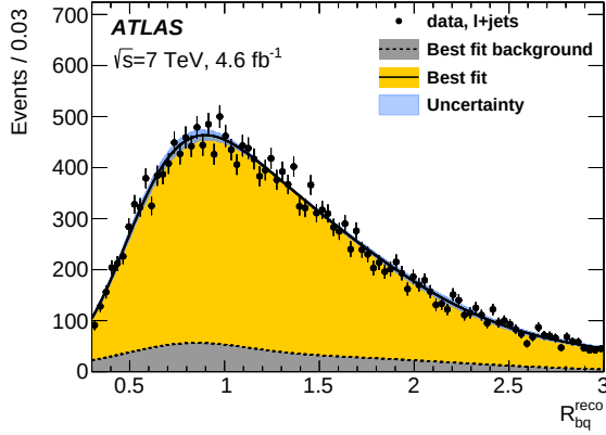
(c) R_{bq}^{\text{reco}}, \ell+\text{jets}
