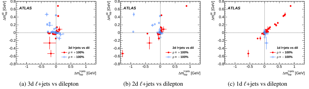
Figure 6: The systematic uncertainties of m_{\text{top}} in the \ell +jets analysis versus those of the dilepton analysis. Figures (a–c) refer to the results evaluated for the three-dimensional analysis (3d), two-dimensional analysis (2d) and one-dimensional analysis (1d). The points show the estimated systematic uncertainties on m_{\text{top}} for the two analyses, and the uncertainty bars reflect the corresponding statistical uncertainties. The different colours reflect the different correlations described in Sect. 8.1.
