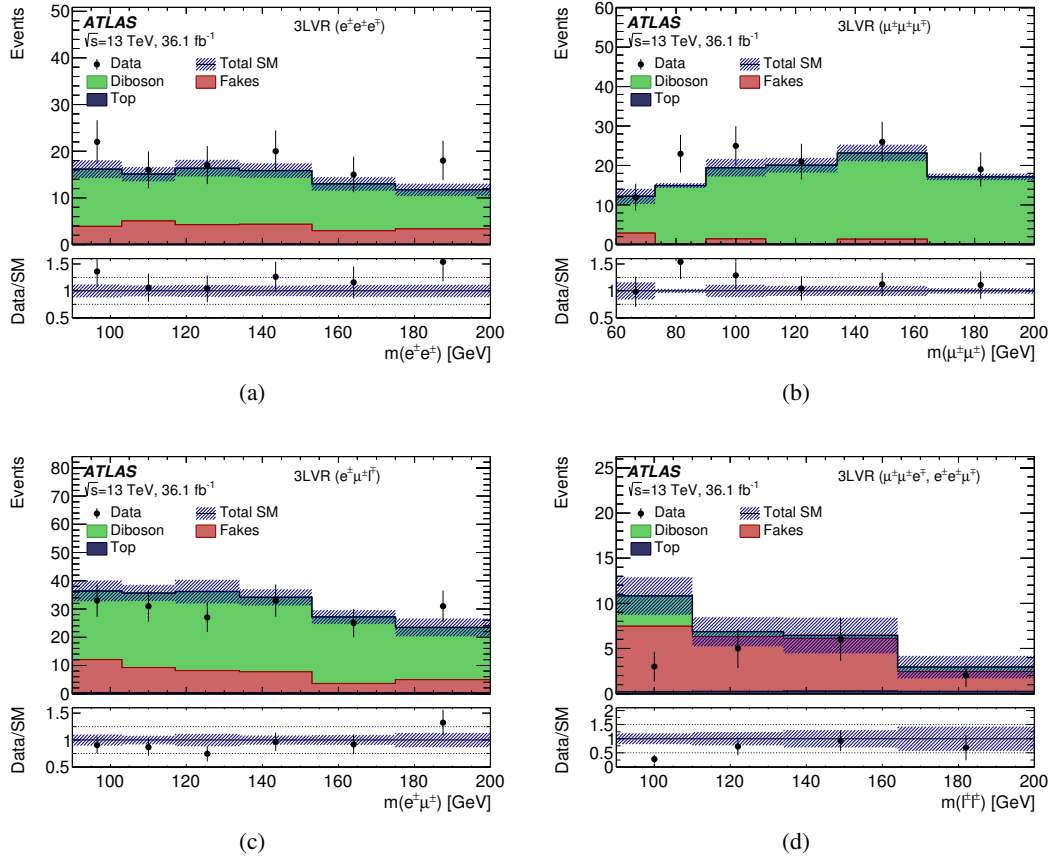
Figure 5: Distribution of dilepton mass for data and SM background predictions in three-lepton validation regions: (a) the three-electron validation region, (b) the three-muon validation region, (c) the 3LVR with an electron–muon same-charge pair ( e^\pm\mu^\pm\ell^\mp ), and (d) the 3LVR with a same-flavour same-charge pair ( e^\pm e^\pm\mu^\mp or \mu^\pm\mu^\pm e^\mp ). The hatched bands include all systematic uncertainties post-fit, with the correlations between various sources taken into account.
