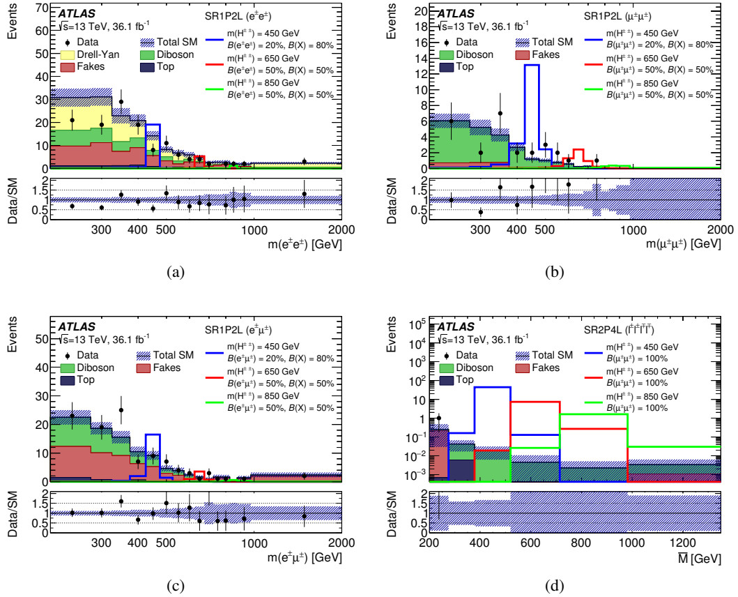
Figure 8: Distributions of m(\ell^\pm \ell^\pm) in representative signal regions, namely (a) the electron–electron two-lepton signal region (SR1P2L), (b) the muon–muon two-lepton signal region (SR1P2L), (c) the electron–muon two-lepton signal region (SR1P2L), and (d) the four-lepton signal region (SR2P4L). The hatched bands include all systematic uncertainties post-fit with the correlations between various sources taken into account. The solid coloured lines correspond to signal samples, normalised using the theory cross-section, with the H^{\pm\pm} mass and decay modes marked in the legend.
