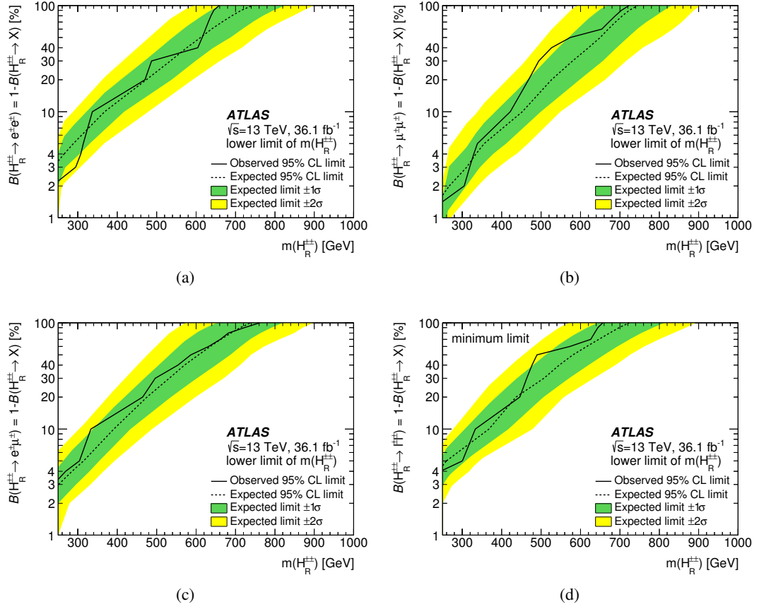
Figure 14: Lower limit on the H_R^{\pm\pm} boson mass as a function of the branching ratio B(H_R^{\pm\pm} \rightarrow \ell^\pm \ell^\pm) . Several cases are presented: (a) H_R^{\pm\pm} decays only into electrons and "X", (b) H_R^{\pm\pm} decays only into muons and "X", and (c) H_R^{\pm\pm} decays only into electron–muon pairs and "X", with "X" not entering any of the signal regions. Plot (d) shows the minimum observed and expected limit as a function of B(H_R^{\pm\pm} \rightarrow \ell^\pm \ell^\pm) .
