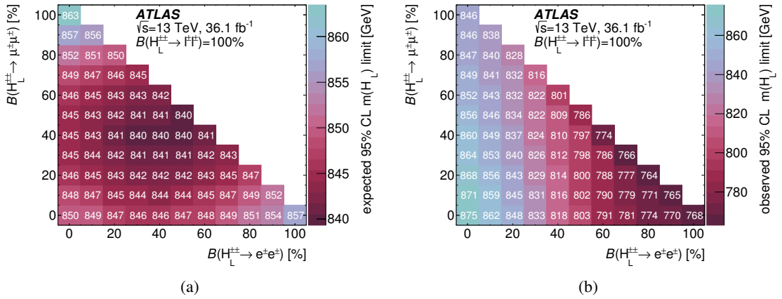
Figure 11: The (a) expected and (b) observed lower limits on the H_L^{\pm\pm} boson mass for all branching ratio combinations that sum to 100%.
