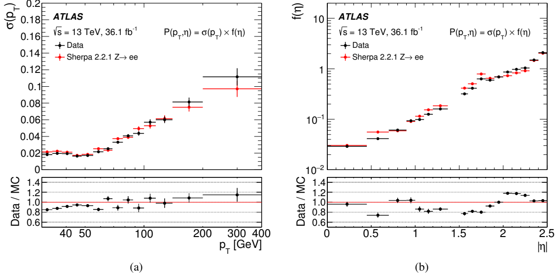
Figure 3: Comparison of the factors composing the charge misidentification probability P(p_T, \eta) = \sigma(p_T) \times f(\eta) measured in data and in simulation using the likelihood fit in the Z/\gamma^* \rightarrow ee region. The area of the distribution describing f(\eta) was set to unity (see text for details). Error bars correspond to the statistical uncertainties estimated with the likelihood fit. Plot (a) shows the charge misidentification probability component as a function of p_T and plot (b) shows the component as a function of |\eta| .
