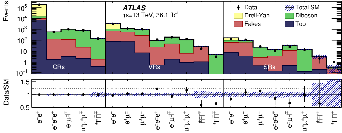
Figure 7: Number of observed and expected events in the control, validation, and signal regions for all channels considered. The background expectation is the result of the fit described in the text. The hatched bands include all systematic uncertainties post-fit with the correlations between various sources taken into account. The notation \ell^\pm\ell'^\pm\ell^\mp indicates that the same-charge leptons have different flavours and \ell^\pm\ell^\pm\ell'^\mp indicates that same-charge leptons have the same flavour, while the opposite-charge lepton has a different flavour.
