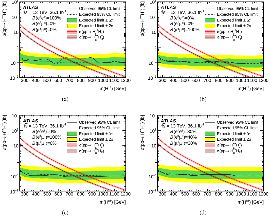
Figure 10: Upper limit on the cross-section for pp \rightarrow H^{++}H^{--} for several branching ratio values presented in the form B(ee)/B(e\mu)/B(\mu\mu) : (a) 100%/0%/0%, (b) 0%/0%/100%, (c) 0%/100%/0%, and (d) 30%/40%/30%. The theoretical uncertainty in the cross-section for pp \rightarrow H^{++}H^{--} is presented with the shaded band around the central value.
