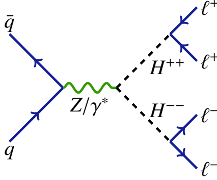
Figure 1: Feynman diagram of the pair production process pp \rightarrow H^{++}H^{--} . The analysis studies only the electron and muon channels, where at least one of the lepton pairs is e^{\pm}e^{\pm} , e^{\pm}\mu^{\pm} , or \mu^{\pm}\mu^{\pm} .
