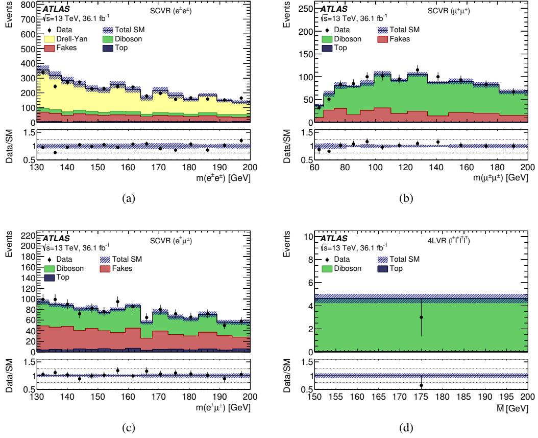
Figure 4: Distributions of dilepton mass for data and SM background predictions in two- and four-lepton validation regions: (a) the electron–electron, (b) the muon–muon, and (c) the electron–muon two-lepton validation regions, as well as (d) the four-lepton validation region. The hatched bands include all systematic uncertainties post-fit, with the correlations between various sources taken into account.
