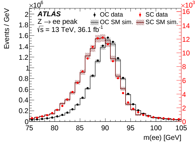
Figure 2: Dielectron mass distributions for opposite-charge (black) and same-charge (red) pairs for data (filled circles) and MC simulation (continuous line). The latter includes a correction for charge misidentification. The hatched band indicates the statistical error and the luminosity uncertainty summed in quadrature applied to MC simulated events.
