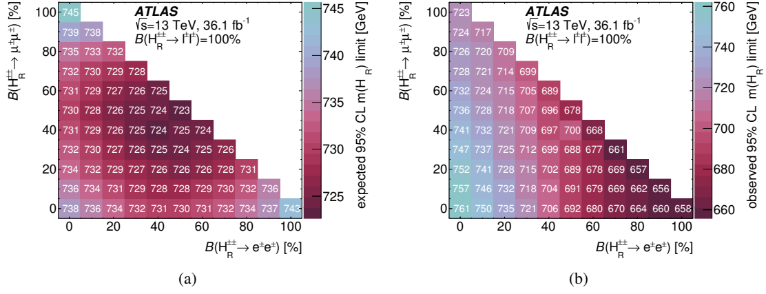
Figure 12: The (a) expected and (b) observed lower limits on the H_R^{\pm\pm} boson mass for all branching ratio combinations that sum to 100%.
