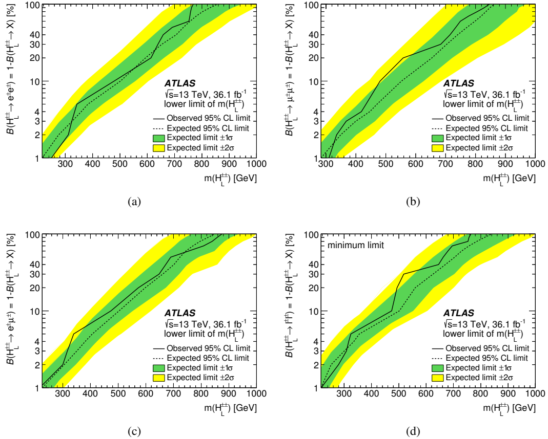
Figure 13: Lower limit on the H_L^{\pm\pm} boson mass as a function of the branching ratio B(H_L^{\pm\pm} \rightarrow \ell^+\ell^-) . Several cases are presented: (a) H_L^{\pm\pm} decays only into electrons and "X", (b) H_L^{\pm\pm} decays only into muons and "X", and (c) H_L^{\pm\pm} decays only into electron-muon pairs and "X", with "X" not entering any of the signal regions. Plot (d) shows the minimum observed and expected limit as a function of B(H_L^{\pm\pm} \rightarrow \ell^+\ell^-) .
