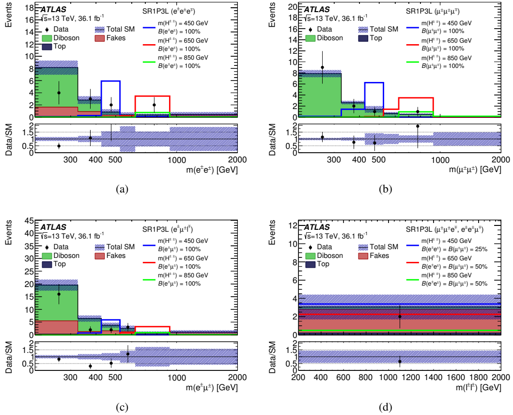
Figure 9: Distributions of m(\ell^\pm \ell^\pm) in three-lepton signal regions, namely (a) the three-electron SR (SR1P3L), (b) the three-muon SR (SR1P3L), (c) the SR1P3L with an electron–muon same-charge pair ( e^\pm \mu^\pm \ell^\mp ), and (d) the SR1P3L with a same-flavour same-charge pair ( e^\pm e^\pm \mu^\mp or \mu^\pm \mu^\pm e^\mp ). The hatched bands include all systematic uncertainties post-fit with the correlations between various sources taken into account. The solid coloured lines correspond to signal samples, normalised using the theory cross-section, with the H^{\pm\pm} mass and decay modes marked in the legend.
