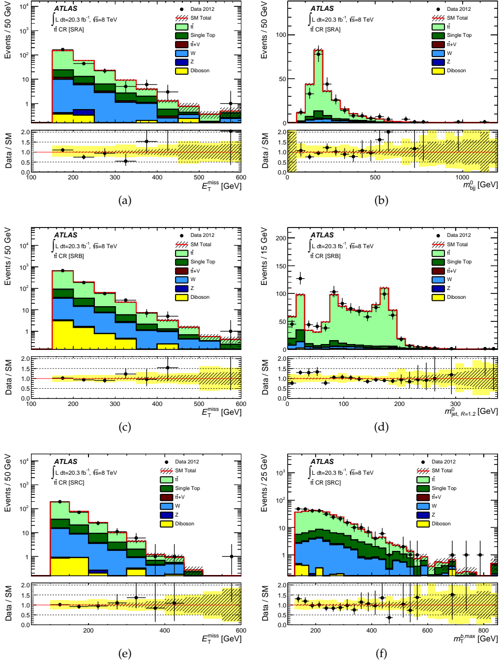
Figure 3. Distributions in the semileptonic t\bar{t} control region of (a) E_T^{\text{miss}} and (b) m_{b_{jj}}^0 for SRA, (c) E_T^{\text{miss}} and (d) m_{\text{jet}, R=1.2}^0 for SRB, and (e) E_T^{\text{miss}} and (f) m_T^{b, \text{max}} for SRC after the application of all selection requirements. All kinematic quantities were recalculated after treating the lepton as a jet. The stacked histograms show the Standard Model expectation, normalized using the factors summarized in table 8. The “Data/SM” plots show the ratio of data events to the total Standard Model expectation. The rightmost bin includes all overflows. The hatched uncertainty band around the Standard Model expectation shows the statistical uncertainty and the yellow band (shown only for the “Data/SM” plots) shows the combination of statistical and detector-related systematic uncertainties.
