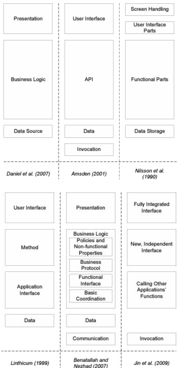
Figure 1 – Classification of levels [10]
