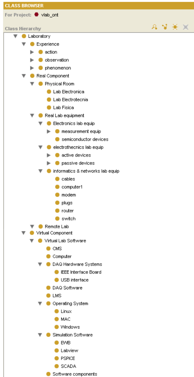
Figure 7 – EuronetLab Ontology definition
