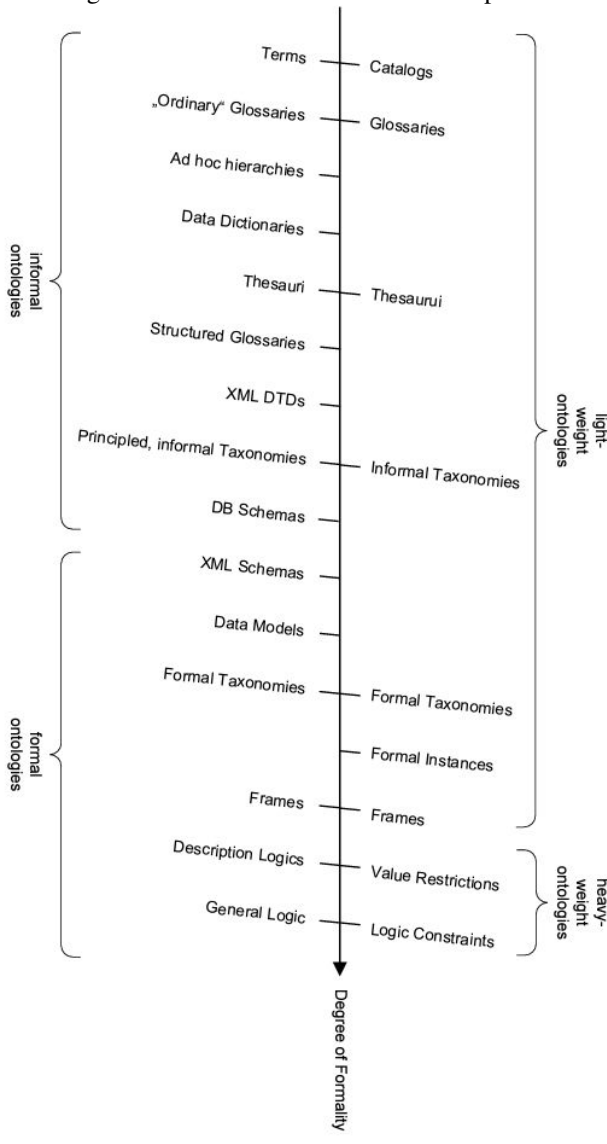
Figure 5 – Ontology types based on the degree of formality
