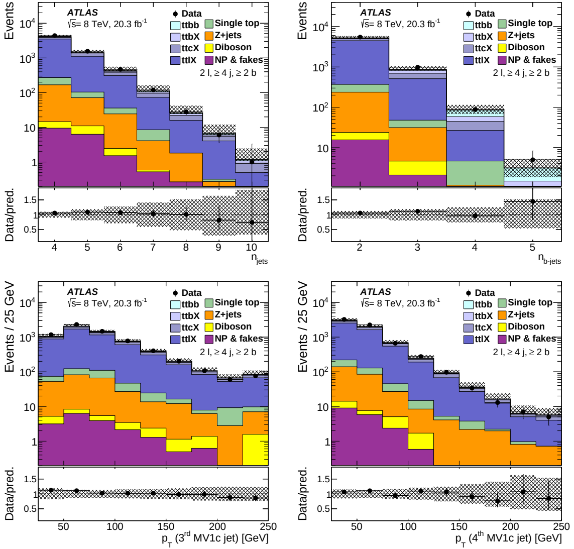
Figure 2: Jet multiplicity, b -tagged jet multiplicity, and transverse momentum p_T of the jets with the third and fourth highest MV1c values, in the dilepton channel using the t\bar{t}b\bar{b} fit-based selection; events are required to have at least four jets, two b -tagged jets and two leptons ( ee , e\mu or \mu\mu ). The data are shown in black points with their statistical uncertainty. The stacked distributions are the nominal predictions from Monte Carlo simulation; the hashed area shows the total uncertainty on the prediction. The bottom sub-plot shows the ratio of the data to the prediction. The non-prompt and fake lepton backgrounds are referred to as ‘NP & fakes’. The last bin of the distribution includes the overflow.
