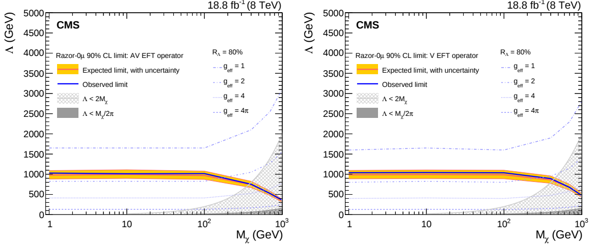
Figure 7: Lower limit at 90% CL on the cutoff scale \Lambda as a function of the DM mass M_\chi in the case of axial-vector (left) and vector (right) currents. The validity of the EFT is quantified by R_\Lambda = 80\% contours, corresponding to different values of the effective coupling g_{\text{eff}} . For completeness, regions forbidden by the EFT validity condition \Lambda > 2M_\chi/g_{\text{eff}} are shown for two choices of the effective coupling: g_{\text{eff}} = 1 (light gray) and g_{\text{eff}} = 4\pi (dark gray).
