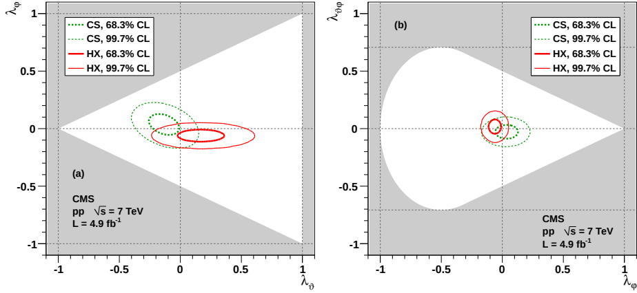
Figure 2: Two-dimensional projections of the PPD in the \lambda_\phi vs. \lambda_\theta (a) and \lambda_{\theta\phi} vs. \lambda_\phi (b) planes, for Y(1S) with |y| < 0.6 and 30 < p_T < 50 GeV. The 68.3% and 99.7% CL contours are shown for the CS and HX frames. The shaded areas represent physically forbidden regions of parameter space [18].
