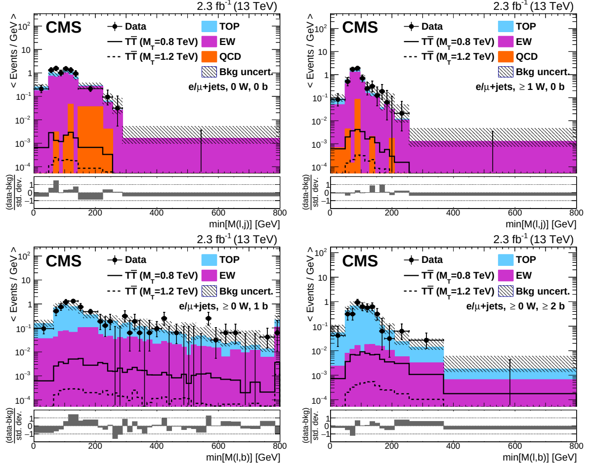
Figure 8: Distributions of \min[M(\ell, j)] in the W + jets control region of the boosted W channel (upper) for 0/ \geq 1 W tag categories (left/right), and \min[M(\ell, b)] in the t\bar{t} control region of the boosted W channel (lower) for 1/ \geq 2 b tag categories (left/right). Also shown are the distributions of T\bar{T} signal events with T quark masses of 0.8 and 1.2 TeV. The uncertainty in the background includes the statistical and systematic uncertainties described in Section 7.
