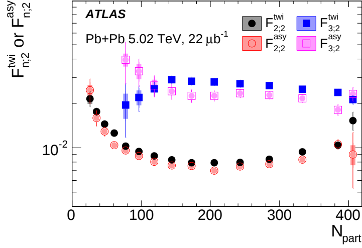
Figure 20: The estimated event-plane twist component F_{n;2}^{twi} and FB asymmetry component F_{n;2}^{asy} as a function of N_{part} for n = 2 and 3 for Pb+Pb collisions at 5.02 TeV. The error bars and shaded boxes are statistical and systematic uncertainties, respectively.
