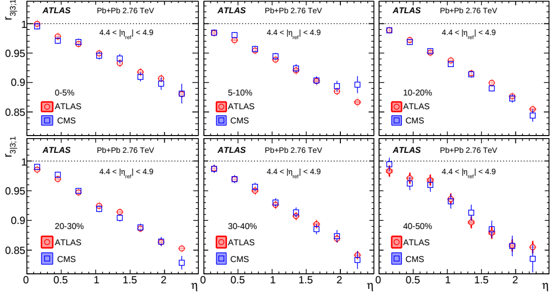
Figure 26: The values of r_{3|3,1} measured by ATLAS and by CMS [19] for Pb+Pb collisions at 2.76 TeV, for the same reference pseudorapidity 4.4 < |\eta_{\text{ref}}| < 4.9 .
