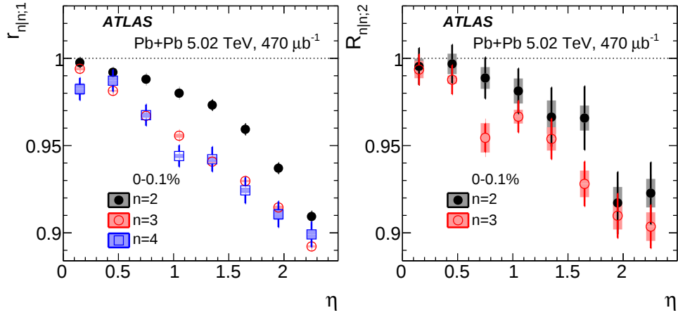
Figure 29: The r_{\eta|n;1}(\eta) (left panel) and R_{\eta|n;2}(\eta) (right panel) in ultra-central Pb+Pb collisions at 5.02 TeV. The error bars and shaded boxes are statistical and systematic uncertainties, respectively.
