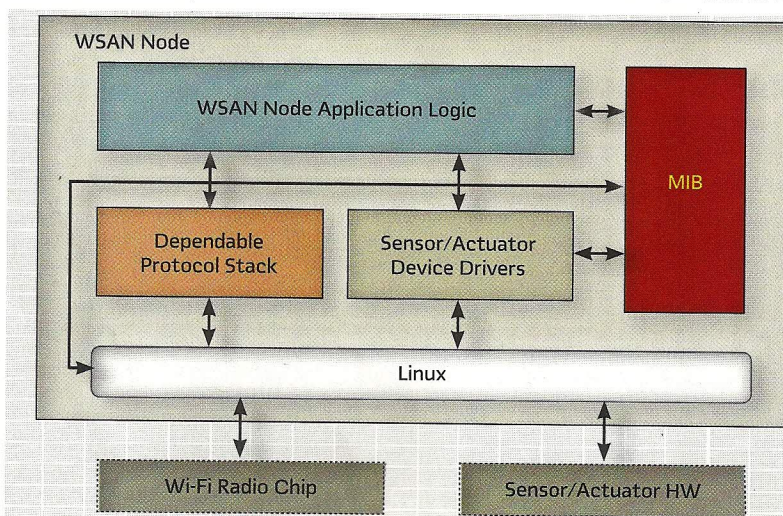
Figure 6 depicts the software modules of the WSAN node. The selected Operating System is Linux.
