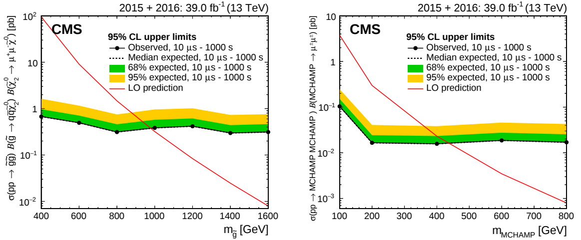
Figure 8: 95% CL upper limits on B\sigma for gluino (left) and MCHAMP (right) pair production as a function of mass, for lifetimes between 10 \mu\text{s} and 1000 s, for combined 2015 and 2016 data for the muon search. The theory curves assume B = 100\% .
