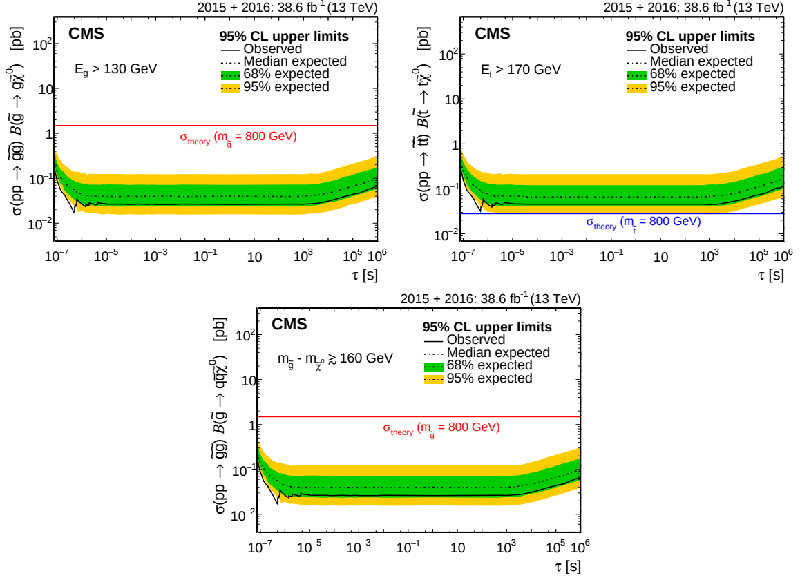
Figure 4: The 95% CL upper limits on B\sigma for gluino and top squark pair production, using the cloud model of R-hadron interactions, as a function of lifetime, for combined 2015 and 2016 data for the calorimeter search. We show gluinos that undergo a two-body decay (upper left), top squarks that undergo a two-body decay (upper right), and gluinos that undergo a three-body decay (lower). The discontinuous structure observed between 10^{-7} and 10^{-5} s is due to the increase of the number of observed events in the search window as the lifetime increases. The theory lines assume B = 100\% .
