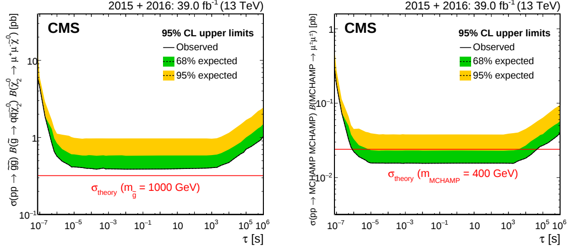
Figure 7: The 95% CL upper limits on B\sigma for 1000 GeV gluino (left) and 400 GeV MCHAMP (right) pair production as a function of lifetime, for combined 2015 and 2016 data for the muon search. The theory lines assume B = 100\% .
