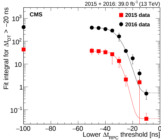
Figure 3: The background extrapolation for the muon search. The integral of the fit function to \Delta t_{\text{DT}} with the sum of two Gaussian distributions and a Crystal Ball function, for \Delta t_{\text{DT}} > -20 ns, is plotted as a function of the lower \Delta t_{\text{RPC}} selection, for 2015 (red squares) and 2016 (black circles) data. The points are fitted with an error function and used to extrapolate to the signal region, which is defined as \Delta t_{\text{RPC}} > -7.5 ns.
