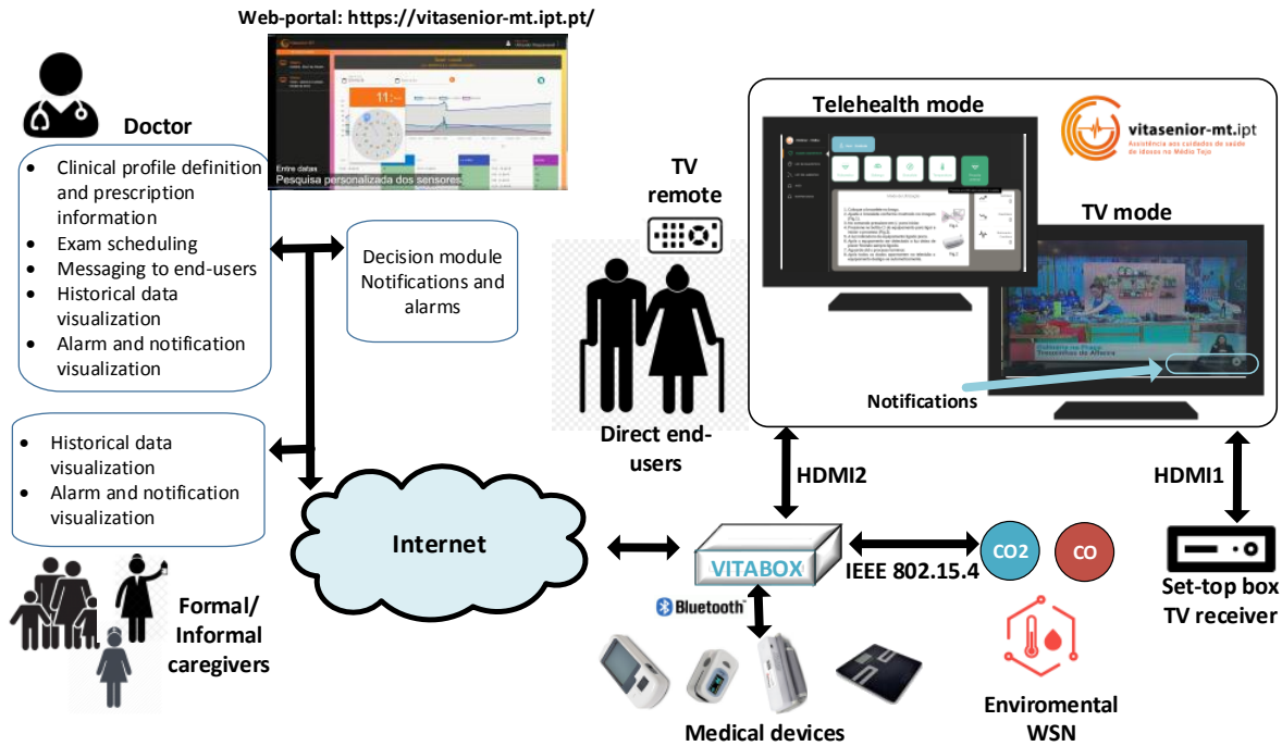
Fig. 1 VITASENIOR-MT architecture overview.
