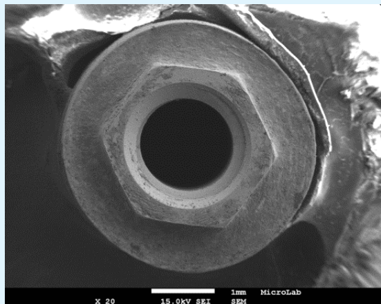
Figure 2: SEM of implant hexagon group A.
