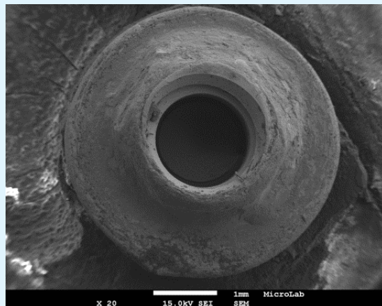
Figure 5: SEM of implant hexagon group D Zirconia abutment.
