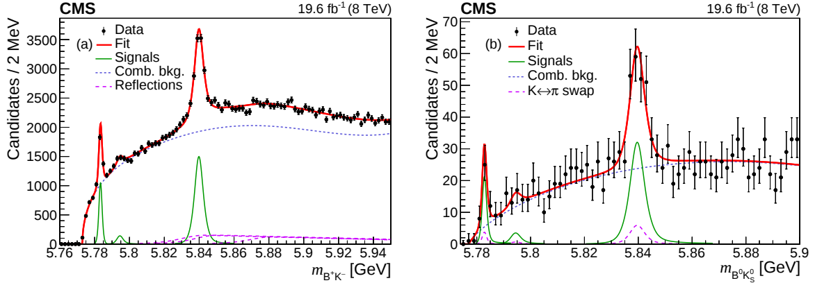
Figure 3: Invariant mass distributions of (a) B^+ K^- and (b) B^0 K_S^0 candidates with the results of the fit overlaid. The points represent the data, the thick solid curves are the results of the overall fits, and the thin solid lines display the signal contributions. The short-dashed lines show the combinatorial background contributions. The long-dashed lines show: in (a) the contributions from excited B^0 meson decays, and in (b) the contributions from swapping K^\pm \rightarrow \pi^\pm in the reconstruction of the B^0 mesons.
