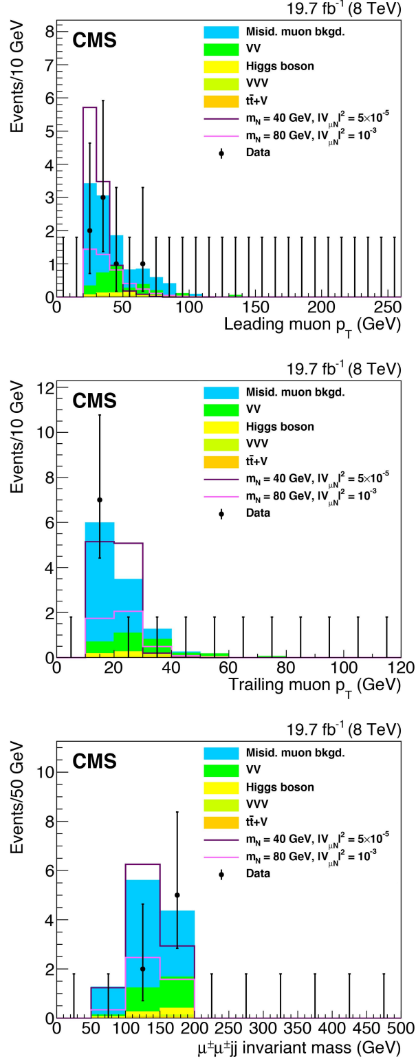
Figure 2: Kinematic distributions for the low-mass region after all selections are applied except for the final optimization requirements: leading muon p_T (top), trailing muon p_T (middle), and \mu^\pm\mu^\pm jj invariant mass (bottom). The plots show the data, backgrounds, and two choices for the heavy Majorana neutrino signal: m_N = 40 GeV, |V_{\mu N}|^2 = 5 \times 10^{-5} and m_N = 80 GeV, |V_{\mu N}|^2 = 1 \times 10^{-3} . The backgrounds shown are from misidentified muons and from diboson (VV), Higgs boson, triboson (VVV), and t\bar{t}W production.
