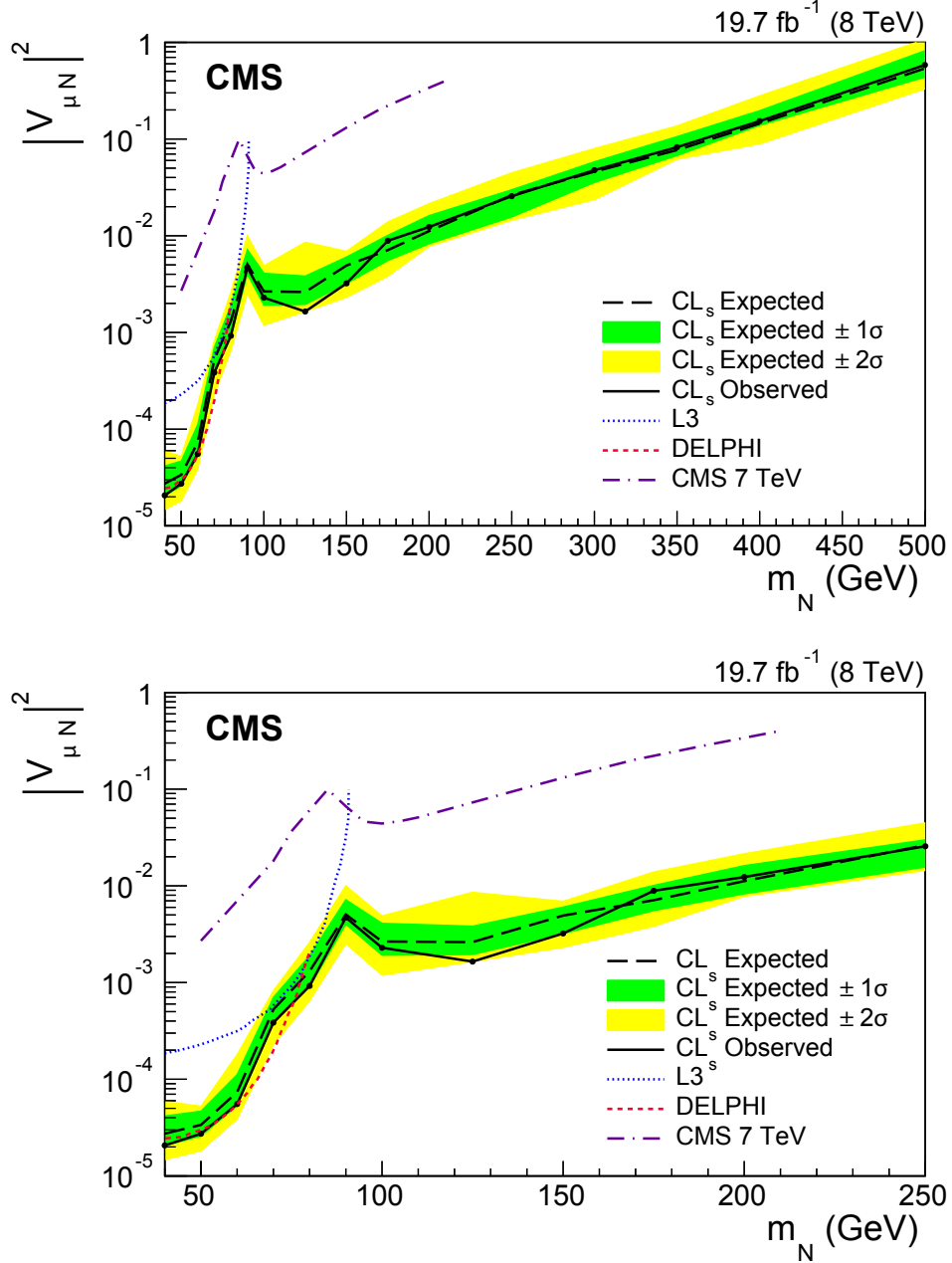
Figure 6: Exclusion region at 95% CL in the square of the heavy Majorana neutrino mixing parameter as a function of the heavy Majorana neutrino mass: ( |V_{\mu N}|^2 vs. m_N ). The long-dashed black curve is the expected upper limit, with one and two standard deviation bands shown in dark green and light yellow, respectively. The solid black curve is the observed upper limit. Also shown are the upper limits from other direct searches: L3 [20], DELPHI [21], and the upper limits from CMS obtained with the 2011 LHC data at \sqrt{s} = 7 TeV [22]. The regions above the exclusion curves are ruled out. The lower panel shows an expanded view of the region 40 \text{ GeV} < m_N < 250 \text{ GeV} .
