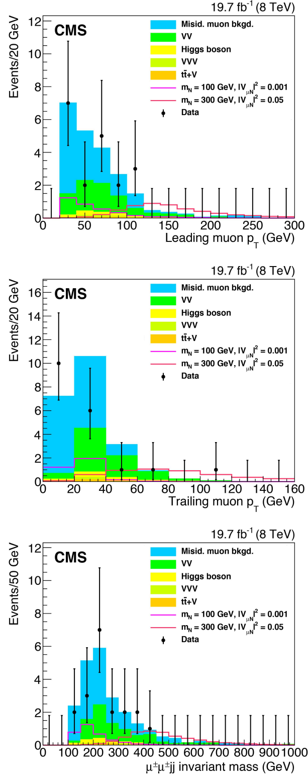
Figure 3: Kinematic distributions for the high-mass region after all selections are applied except for the final optimization requirements: leading muon p_T (top), trailing muon p_T (middle), and \mu^\pm\mu^\pm jj invariant mass (bottom). The plots show the data, backgrounds, and two choices for the heavy Majorana neutrino signal: m_N = 100 \text{ GeV} , |V_{\mu N}|^2 = 0.001 and m_N = 300 \text{ GeV} , |V_{\mu N}|^2 = 0.05 . The backgrounds shown are from misidentified muons and from diboson (VV), Higgs boson, triboson (VVV), and t\bar{t}W production.
