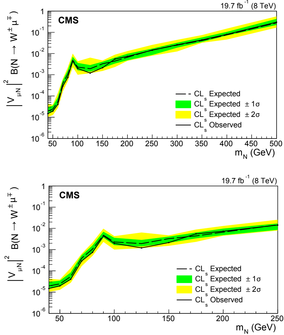
Figure 5: Exclusion region at 95% CL in the square of the heavy Majorana neutrino mixing parameter times branching fraction of the N to a W boson and a muon, as a function of the heavy Majorana neutrino mass: ( |V_{\mu N}|^2 \mathcal{B}(N \rightarrow W^\pm \mu^\mp) vs. m_N ). The long-dashed black curve is the expected upper limit, with one and two standard deviation bands shown in dark green and light yellow, respectively. The solid black curve is the observed upper limit. The regions above the exclusion curves are ruled out. The lower panel shows an expanded view of the region 40 \text{ GeV} < m_N < 250 \text{ GeV} .
