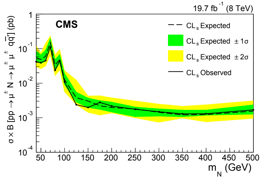
Figure 4: Exclusion region at 95% CL in the cross section times branching fraction, as a function of the heavy Majorana neutrino mass. The long-dashed black curve is the expected upper limit, with one and two standard deviation bands shown in dark green and light yellow, respectively. The solid black curve is the observed upper limit. The region above the exclusion curves is ruled out.
