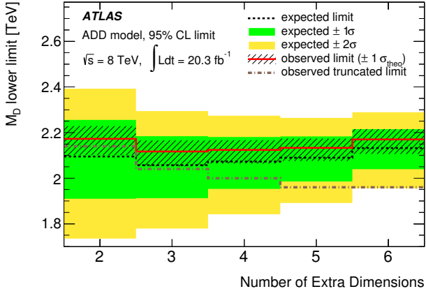
FIG. 18. Lower limits at 95% C.L. on the mass scale M_D in the ADD model of large extra dimensions, for several values of the number of extra dimensions. The expected and observed limits are shown, along with the limit obtained after applying truncation.
