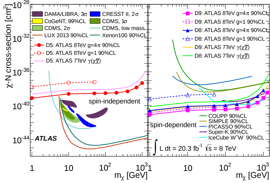
FIG. 13. Upper limits at 90% C.L. on the WIMP–nucleon ( \chi -N) scattering cross section as a function of m_\chi for spin-independent (left) and spin-dependent (right) interactions, for a coupling strength g = \sqrt{g_f g_\chi} of unity or the maximum value ( 4\pi ) that keeps the model within its perturbative regime. The truncation procedure is applied for both cases. The results obtained from ATLAS with 7 TeV data for the same channel are shown for comparison. Also shown are results from various dark-matter search experiments [73–85].
