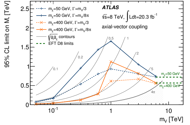
FIG. 16. Observed limits at 95% C.L. on the EFT suppression scale M_* as a function of the mediator mass m_V , for a Z' -like mediator with axial-vector interactions. For a dark-matter mass m_\chi of 50 or 400 GeV, results are shown for different values of the mediator total decay width \Gamma and compared to the EFT observed limit results for a D8 (axial-vector) interaction. M_* vs m_V contours for an overall coupling \sqrt{g_f g_\chi} = 0.1, 0.2, 0.5, 1, 2, 5, 4\pi are also shown. The corresponding limits from the D8 operator are shown as a dashed line.
