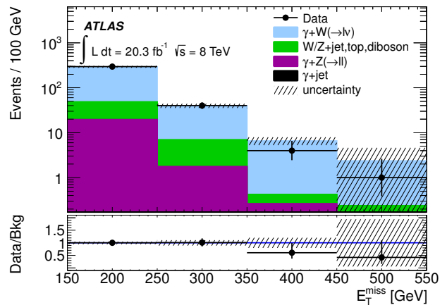
FIG. 6. Distribution of E_T^{\text{miss}} in the data and for the expected background in the single-muon control region. The total background expectation is normalized to the observed number of events in this control region. The dashed band includes statistical and systematic uncertainties. Overflows are included in the final bin. The lower part of the figure shows the ratios of data to expected-background event yields.
