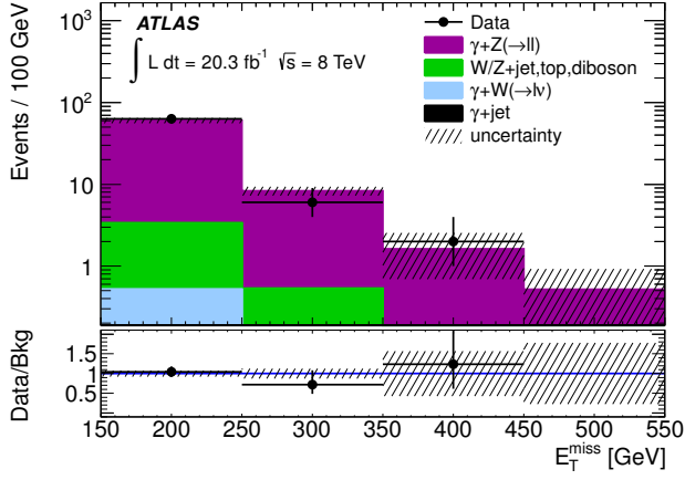
FIG. 7. Distribution of E_T^{\text{miss}} in the data and for the expected background in the two-muon control region. The total background expectation is normalized to the observed number of events in this control region. The dashed band includes statistical and systematic uncertainties. Overflows are included in the final bin. The lower part of the figure shows the ratios of data to expected-background event yields.
