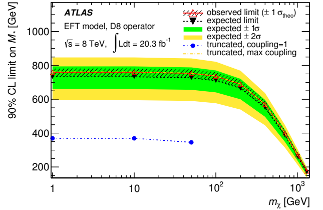
FIG. 11. Limits at 90% C.L. on the EFT suppression scale M_* as a function of the WIMP mass m_\chi , for the axial-vector operator D8. Results where EFT truncation has been applied (see text) are also shown, assuming coupling values \sqrt{g_f g_\chi} = 1, 4\pi .
