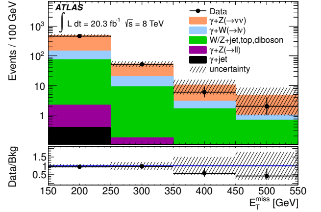
FIG. 9. Distribution of E_T^{\text{miss}} in the signal region for data and for the background predicted from the fit in the CRs. The dashed band includes statistical and systematic uncertainties. Overflows are included in the final bin. The lower part of the figure shows the ratios of data to expected-background event yields.
