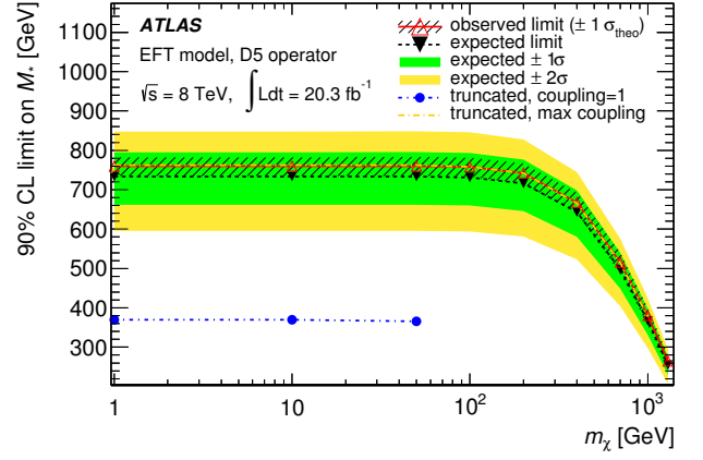
FIG. 10. Limits at 90% C.L. on the EFT suppression scale M_* as a function of the WIMP mass m_\chi , for the vector operator D5. Results where EFT truncation is applied (see text) are also shown, assuming coupling values \sqrt{g_f g_\chi} = 1, 4\pi .
