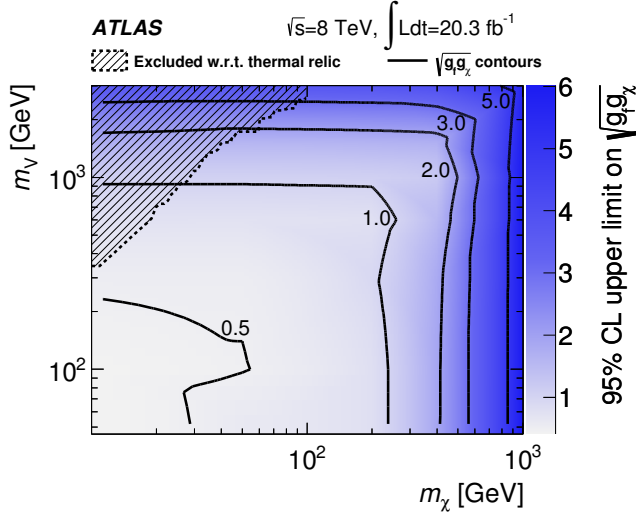
FIG. 14. Upper limits at 95% C.L. on the WIMP simplified-model coupling parameter, \sqrt{g_f g_\chi} , with vector coupling and mediator width \Gamma = m_V/3 , as a function of the WIMP ( m_\chi ) and the mediator particle ( m_V ) masses. Solid lines indicate contours in the coupling parameter. The lower limit on the coupling resulting from the relic abundance of DM is also shown.
