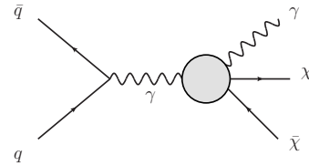
FIG. 4. Production of pairs of dark-matter particles ( \chi\bar{\chi} ) via an effective \gamma\chi\bar{\chi} vertex.
