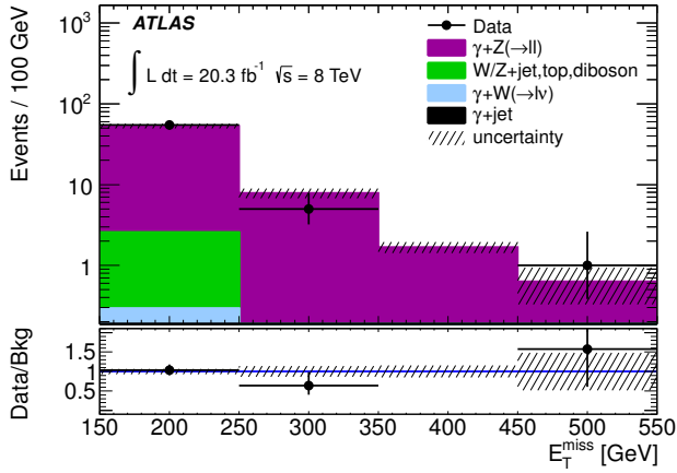
FIG. 8. Distribution of E_T^{\text{miss}} in the data and for the expected background in the two-electron control region. The total background expectation is normalized to the observed number of events in this control region. The dashed band includes statistical and systematic uncertainties. Overflows are included in the final bin. The lower part of the figure shows the ratios of data to expected-background event yields.
