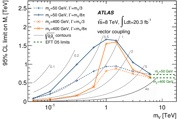
FIG. 15. Observed lower limits at 95% C.L. on the EFT suppression scale M_* as a function of the mediator mass m_V , for a Z' -like mediator with vector interactions. For a dark-matter mass m_\chi of 50 or 400 GeV, results are shown for different values of the mediator total decay width \Gamma and compared to the EFT observed limit results for a D5 (vector) interaction. M_* vs m_V contours for an overall coupling \sqrt{g_f g_\chi} = 0.1, 0.2, 0.5, 1, 2, 5, 4\pi are also shown. The corresponding limits from the D5 operator are shown as a dashed line.
