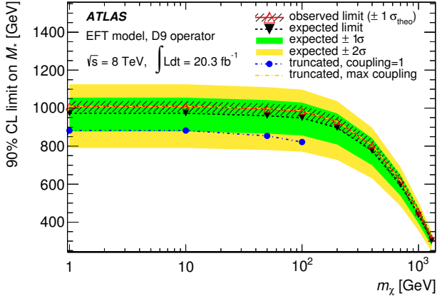
FIG. 12. Limits at 90% C.L. on the EFT suppression scale M_* as a function of the WIMP mass m_\chi , for the tensor operator D9. Results where EFT truncation is applied (see text) are also shown, assuming coupling values \sqrt{g_f g_\chi} = 1, 4\pi .
