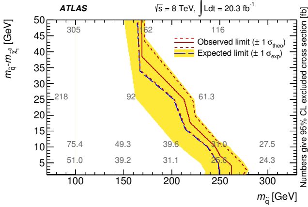
FIG. 19. Upper limits at 95% C.L. on the cross section for the compressed squark model, as a function of the squark mass, m_{\tilde{q}} , and of the difference between the squark mass and the mass of the neutralino, m_{\tilde{q}} - m_{\tilde{\chi}_1^0} , in the compressed region of m_{\tilde{q}} - m_{\tilde{\chi}_1^0} < 50 GeV. The observed (solid line) and expected (dashed line) upper limits from this analysis are shown; the upper limit on the cross section (in fb) is indicated for each model point.
