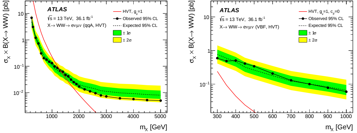
Figure 11: Upper limits at 95% CL on the resonance production cross section times branching fraction \sigma_X \times B(X \rightarrow WW) in the e\nu\mu\nu channel, for HVT qqA (left) and VBF (right) signals. The inner and outer bands show the \pm 1\sigma and \pm 2\sigma ranges around the expected limit. The full curves without dots correspond to the predicted theoretical cross sections.
