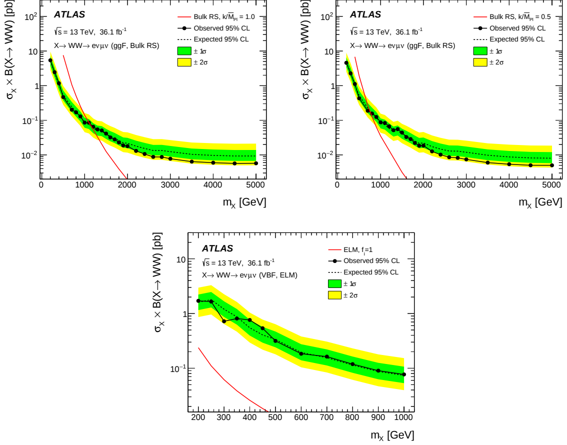
Figure 12: Upper limits at 95% CL on the resonance production cross section times branching fraction \sigma_X \times B(X \rightarrow WW) in the e\nu\mu\nu channel, for a graviton signal with two different couplings of k/\bar{M}_{Pl} = 1 (left) and k/\bar{M}_{Pl} = 0.5 (right), and for an ELM spin-2 VBF signal (bottom). The inner and outer bands show the \pm 1\sigma and \pm 2\sigma ranges around the expected limit. The full curves without dots correspond to the predicted theoretical cross sections.
