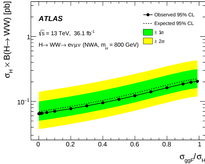
Figure 6: Upper limits at 95% CL on the total ggF and VBF Higgs boson production cross section times branching fraction \sigma_H \times B(H \rightarrow WW) in the e\nu\mu\nu channel, for a signal at 800 GeV as a function of the ggF cross section divided by the combined ggF and VBF production cross section. The inner and outer bands show the \pm 1\sigma and \pm 2\sigma ranges around the expected limit.
