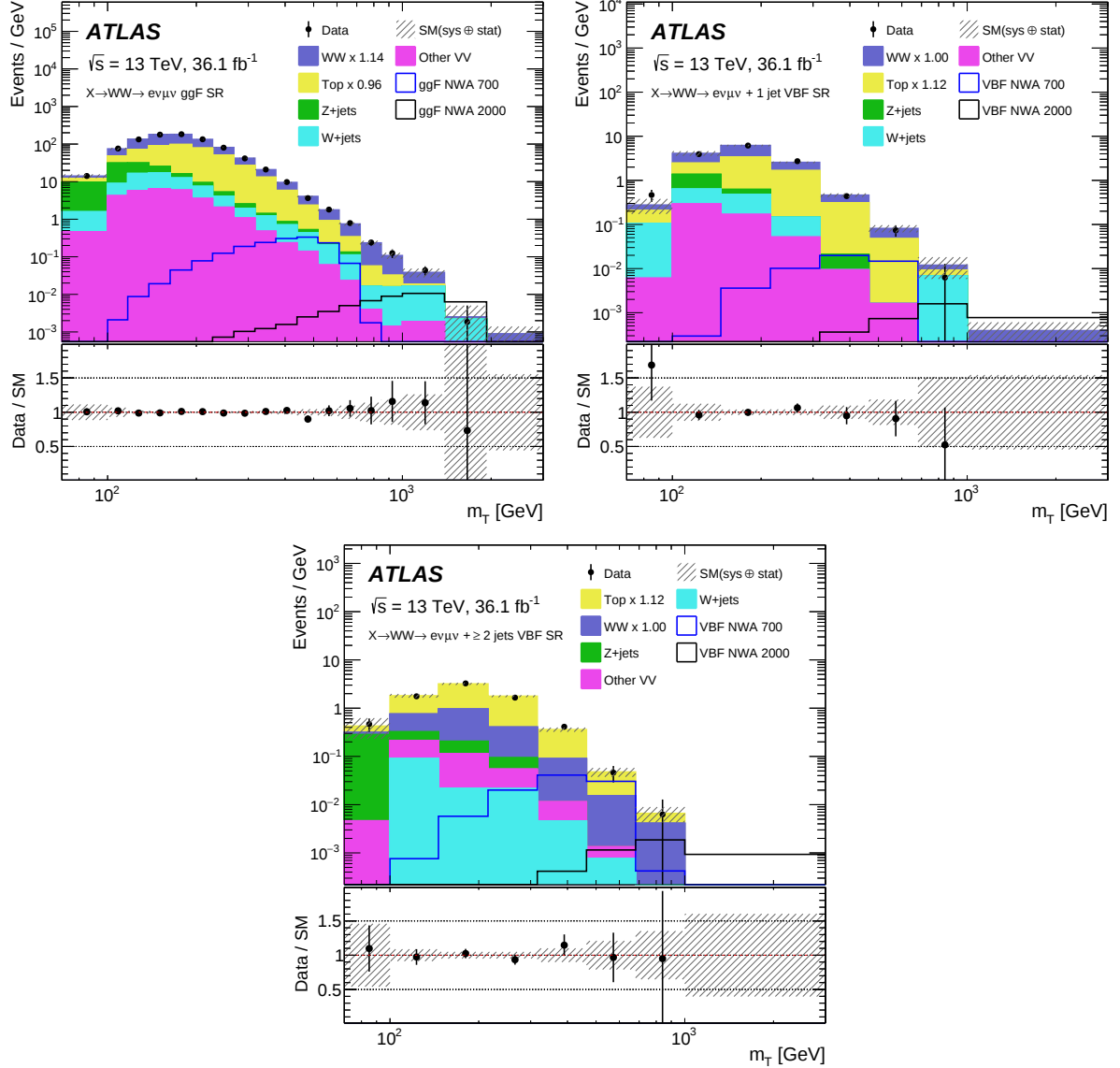
Figure 4: Post-fit distributions of the transverse mass m_T in the SR_{ggF} (top left), SR_{VBF1J} (top right) and SR_{VBF2J} (bottom) categories. In each plot, the last bin contains the overflow. The hatched band in the upper and lower panels shows the total uncertainty of the fit. The top-quark and WW background event yields are scaled using the indicated normalisation factors obtained from the simultaneous fit to all signal and control regions. The heavy Higgs boson signal event yield is normalised to the expected limits on \sigma_H \times B(H \rightarrow WW) and is shown for masses of 700 GeV and 2 TeV in the NWA scenario.
