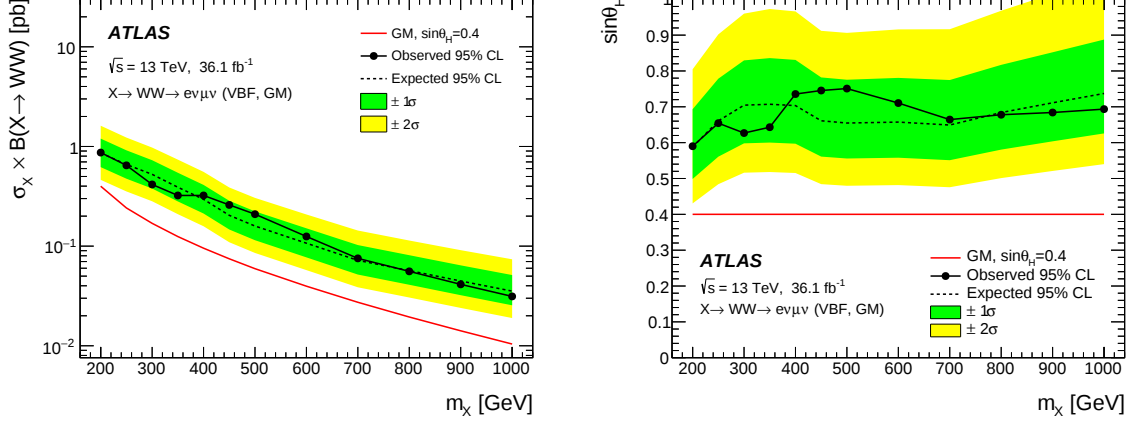
Figure 10: Upper limits at 95% CL on the resonance production cross section times branching fraction \sigma_X \times B(X \rightarrow WW) (left) and on \sin\theta_H (right) in the e\nu\mu\nu channel, for a GM signal. The inner and outer bands show the \pm 1\sigma and \pm 2\sigma ranges around the expected limit. The full curves without dots correspond to the predicted theoretical cross section and the model parameter used in the benchmark model, respectively.
