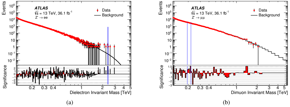
Figure 3: Dilepton mass distribution in the (a) dielectron and (b) dimuon channel, showing the observed data together with their statistical uncertainty, combined background prediction, and corresponding bin-by-bin significance. The most significant interval is indicated by the vertical blue lines. Exact bin edges and contents are provided in Table 10 and Table 11 in the appendix.
