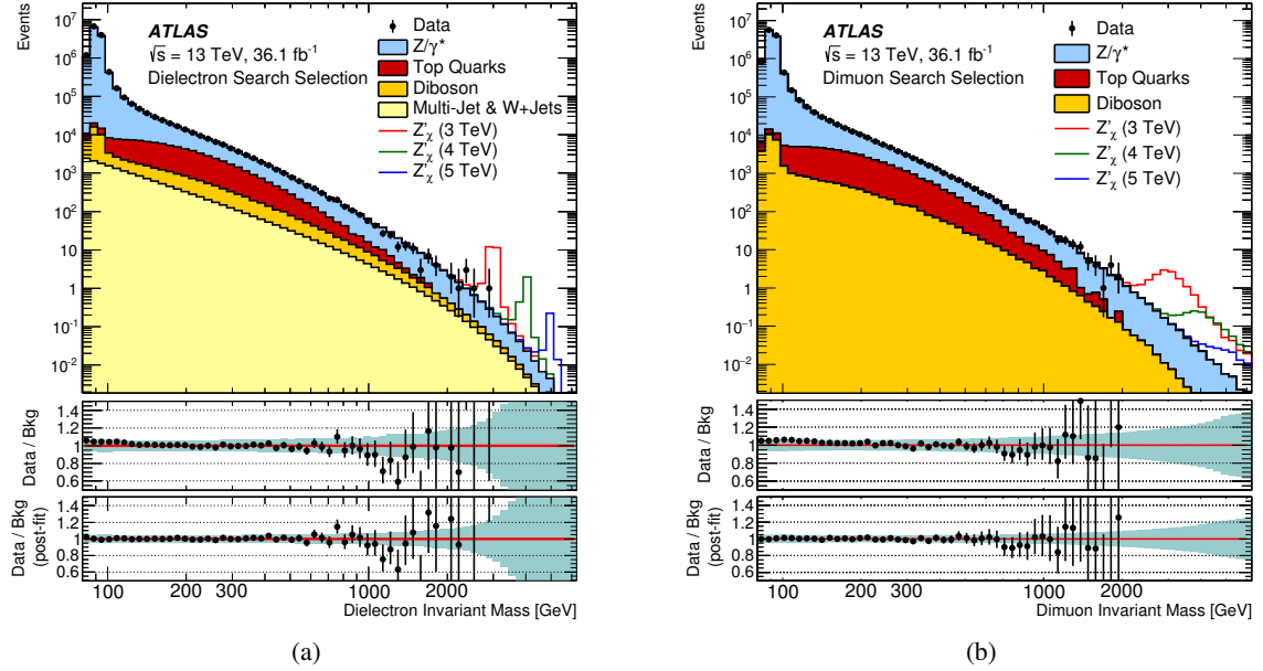
Figure 1: Distributions of (a) dielectron and (b) dimuon reconstructed invariant mass ( m_{\ell\ell} ) after selection, for data and the SM background estimates as well as their ratio before and after marginalisation. Selected Z'_\chi signals with a pole mass of 3, 4 and 5 TeV are overlaid. The bin width of the distributions is constant in \log(m_{\ell\ell}) and the shaded band in the lower panels illustrates the total systematic uncertainty, as explained in Section 7. The data points are shown together with their statistical uncertainty. Exact bin edges and contents are provided in Table 8 and Table 9 in the appendix.
