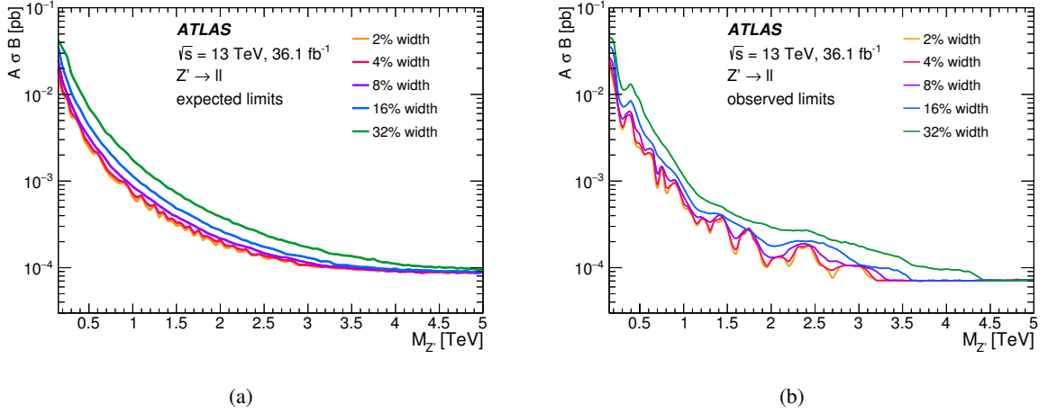
Figure 6: Upper 95% CL limits on the acceptance times Z' production cross-section times branching ratio to two leptons of a single flavour as a function of Z' pole mass ( M_{Z'} ). (a) Expected and (b) observed limits in the combined dilepton channel for different widths with an applied mass window of two times the true width of the signal around the pole mass.
