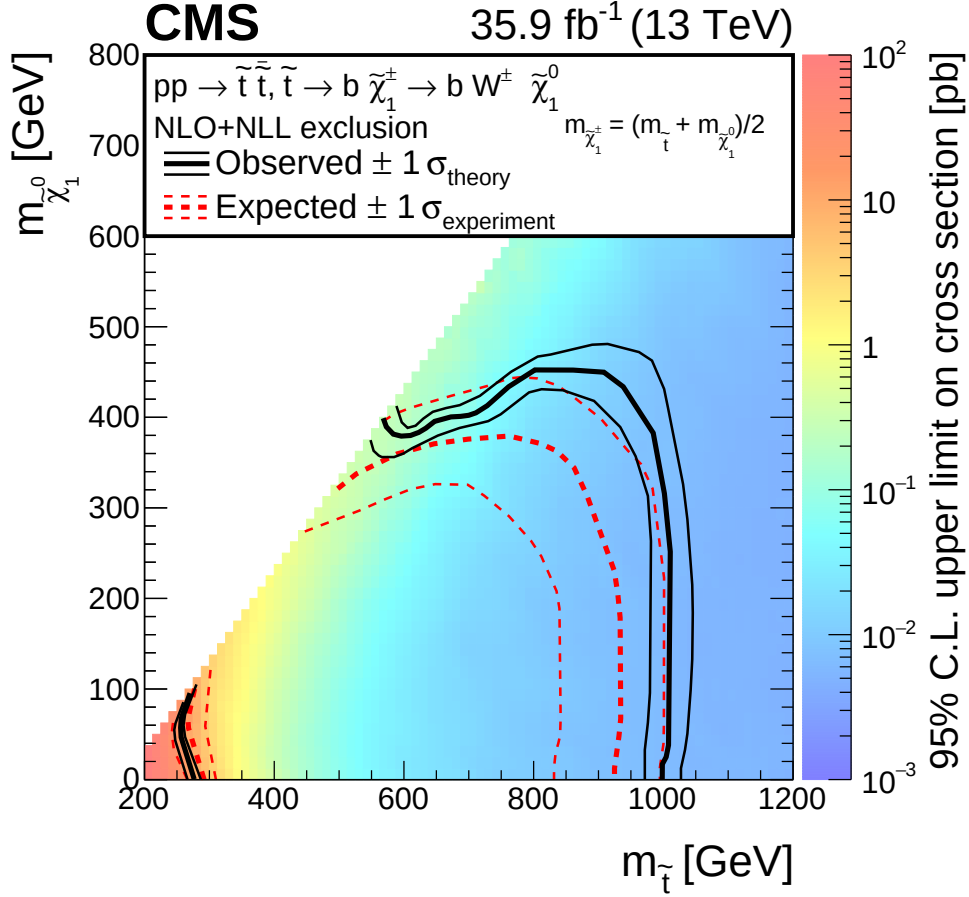
Figure 6: The exclusion limit at 95% CL for direct top squark pair production with decay \tilde{t}\tilde{t}^* \rightarrow b\tilde{\chi}_1^+ \bar{b}\tilde{\chi}_1^- , \tilde{\chi}_1^\pm \rightarrow W^\pm \tilde{\chi}_1^0 . The mass of the chargino is chosen to be (m_{\tilde{t}} + m_{\tilde{\chi}_1^0})/2 . The interpretation is done in the two-dimensional space of m_{\tilde{t}} vs. m_{\tilde{\chi}_1^0} . The color indicates the 95% CL upper limit on the cross section times branching fraction at each point in the m_{\tilde{t}} vs. m_{\tilde{\chi}_1^0} plane. The area between the thick black curves represents the observed exclusion region at 95% CL assuming 100% branching fraction, while the dashed red lines indicate the expected limits at 95% CL and their \pm 1\sigma experimental standard deviation uncertainties. The thin black lines show the effect of the theoretical uncertainties ( \sigma_{\text{theory}} ) in the signal cross section.
