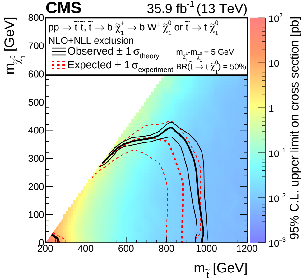
Figure 7: The exclusion limit at 95% CL for direct top squark pair production with decay \tilde{t}\tilde{t}^* \rightarrow b\tilde{\chi}_1^\pm\tilde{\chi}_1^0, \tilde{\chi}_1^\pm \rightarrow W^\pm\tilde{\chi}_1^0 . The mass splitting of the chargino and neutralino is fixed to 5 GeV. The interpretation is done in the two-dimensional space of m_{\tilde{t}} vs. m_{\tilde{\chi}_1^0} . The color indicates the 95% CL upper limit on the cross section at each point in the m_{\tilde{t}} vs. m_{\tilde{\chi}_1^0} plane. The area between the thick black curves represents the observed exclusion region at 95% CL, while the dashed red lines indicate the expected limits at 95% CL and their \pm 1\sigma experimental standard deviation uncertainties. The thin black lines show the effect of the theoretical uncertainties ( \sigma_{\text{theory}} ) in the signal cross section.
