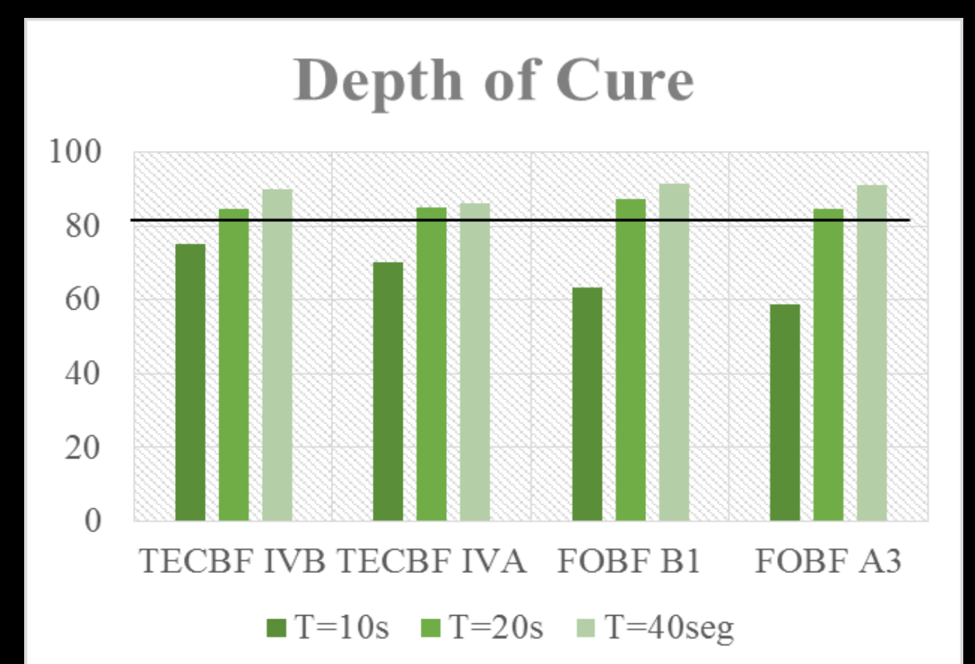
Fig. 6—Depth of cure of TECBF and FOBF according to their shade and curing time (%)
