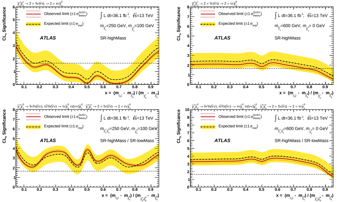
Figure 8: The CL s significance for the benchmark models described in Section 3 as a function of the parameter x . The benchmark scenario with large mass splitting ( m(\tilde{\chi}_1^\pm, \tilde{\chi}_2^0) = 600 \text{ GeV} and m(\tilde{\chi}_1^0) = 0 \text{ GeV} ) is shown on the right, and the compressed benchmark scenario ( m(\tilde{\chi}_1^\pm, \tilde{\chi}_2^0) = 250 \text{ GeV} and m(\tilde{\chi}_1^0) = 100 \text{ GeV} ) on the left, for \tilde{\chi}_1^+ \tilde{\chi}_1^- production (top), and \tilde{\chi}_1^+ \tilde{\chi}_1^- and \tilde{\chi}_1^\pm \tilde{\chi}_2^0 production (bottom). SR-highMass is used for \tilde{\chi}_1^+ \tilde{\chi}_1^- production, while the SR with the best expected CL s value for each point of the parameter space is used for \tilde{\chi}_1^+ \tilde{\chi}_1^- and \tilde{\chi}_1^\pm \tilde{\chi}_2^0 production.
