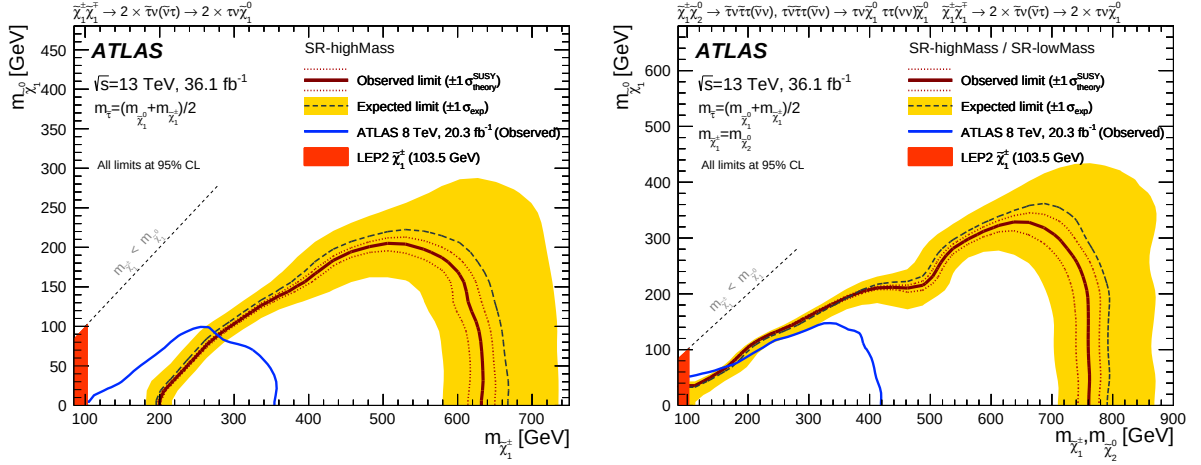
Figure 7: The 95% CL exclusion contours for simplified models with \tilde{\chi}_1^+ \tilde{\chi}_1^- production (left) and production of \tilde{\chi}_1^+ \tilde{\chi}_1^- and \tilde{\chi}_1^\pm \tilde{\chi}_2^0 (right). The text provides details of exclusion curves and uncertainty bands. The LEP limit on the chargino mass is also shown. Results are compared with the observed limits obtained by previous ATLAS searches [29] as blue contours.
