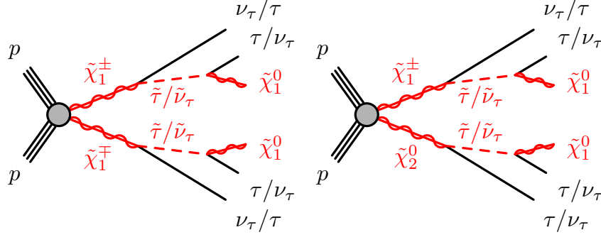
Figure 1: Representative diagrams for the electroweak production and decay processes of supersymmetric particles considered in this work: (left) \tilde{\chi}_1^+ \tilde{\chi}_1^- and (right) \tilde{\chi}_1^\pm \tilde{\chi}_2^0 production.
