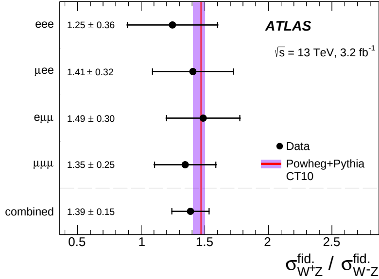
Figure 3: Measured ratios \sigma_{W^+Z}^{fid.} / \sigma_{W^-Z}^{fid.} of W^+Z and W^-Z integrated cross sections in the fiducial phase space in each of the four channels and for their combination. The error bars on the data points represent the total uncertainties, which are dominated by the statistical uncertainties. The NLO SM prediction from PowHEG+PYTHIA using the CT10 PDF set is represented by the red line; the shaded violet band is the total uncertainty in this prediction.
