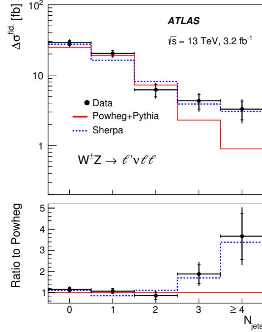
Figure 4: The measured W^{\pm}Z differential cross section in the fiducial phase space as a function of the exclusive jet multiplicity of jets with p_T > 25 GeV. The inner and outer error bars on the data points represent the statistical and total uncertainties, respectively. The measurements are compared to the prediction from POWHEG+PYTHIA (red line) and SHERPA (dashed blue line).
