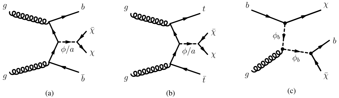
Figure 1: Representative diagrams at the lowest order for spin-0 mediator associated production with top and bottom quarks: (a) colour-neutral spin-0 mediator associated production with bottom quarks b\bar{b} + \phi/a ; (b) colour-neutral spin-0 mediator associated production with top quarks t\bar{t} + \phi/a ; (c) colour-charged scalar mediator model decaying into a bottom quark and a DM particle b -FDM.
