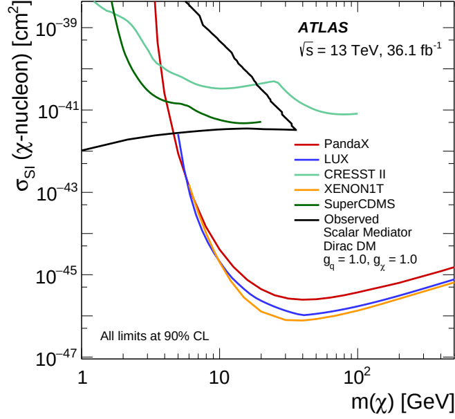
Figure 7: Comparison of the 90% CL limits on the spin-independent DM–nucleon cross-section as a function of DM mass between these results and the direct-detection experiments, in the context of the colour-neutral simplified model with scalar mediator. The black line indicates the exclusion contour derived from the observed limits of SRt3. Values inside the contour are excluded. The exclusion limit is compared with limits from the LUX [103], PandaX-II [104], XENON [105], SuperCDMS [106] and CRESST-II [107] experiments.
