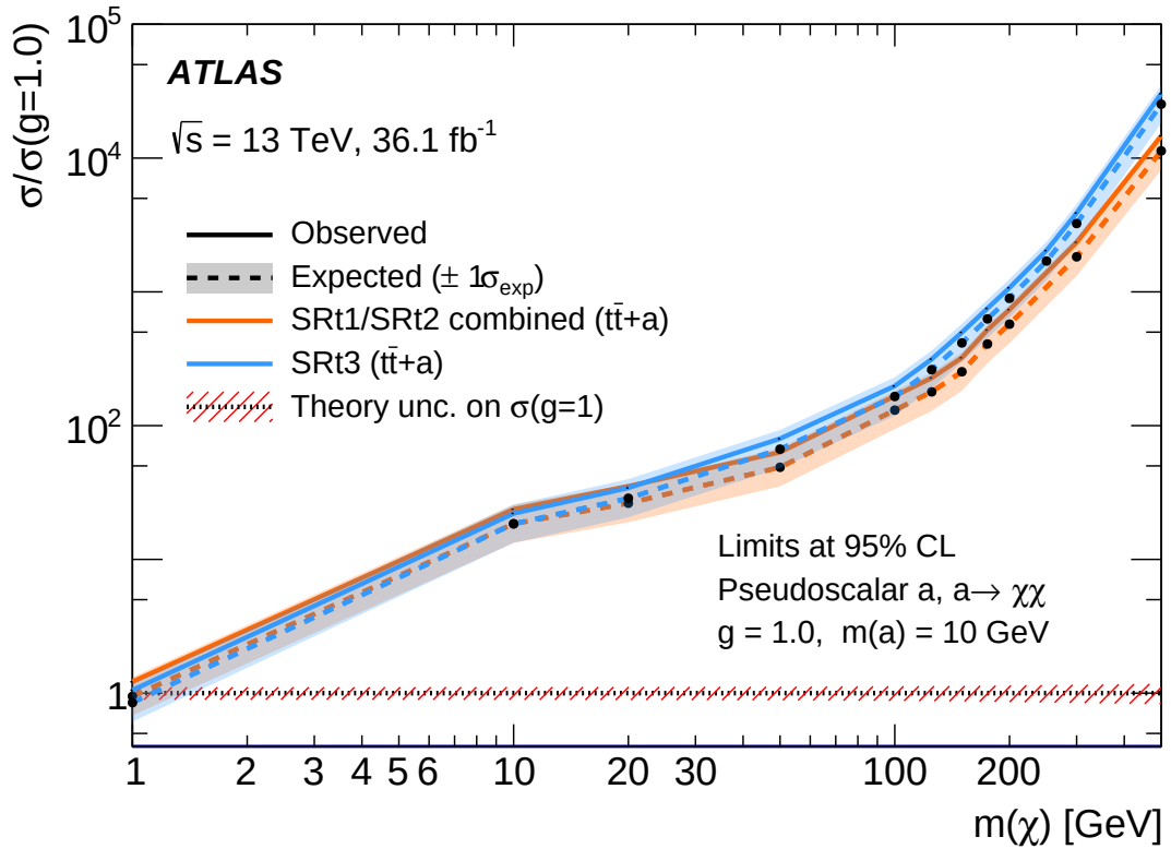
Figure 6: Exclusion limits for colour-neutral t\bar{t} + \phi scalar (top) and t\bar{t} + a pseudoscalar (bottom) models as a function of the DM mass for a mediator mass of 10 GeV. The limits are calculated at 95% CL and are expressed in terms of the ratio of the excluded cross-section to the nominal cross-section for a coupling assumption of g = g_q = g_\chi = 1 . The solid (dashed) lines shows the observed (expected) exclusion limits for the different signal regions, according to the colour code specified in the legend. To derive the results for the fully hadronic t\bar{t} final state the region SRt1 or SRt2 providing the better expected sensitivity is used.
