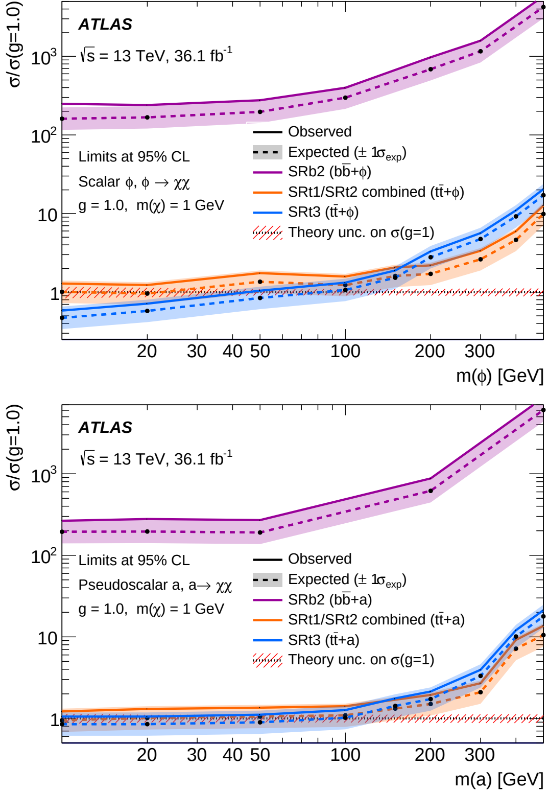
Figure 5: Exclusion limits for colour-neutral t\bar{t}/b\bar{b} + \phi scalar (top) and t\bar{t}/b\bar{b} + a pseudoscalar (bottom) models as a function of the mediator mass for a DM mass of 1 GeV. The limits are calculated at 95% CL and are expressed in terms of the ratio of the excluded cross-section to the nominal cross-section for a coupling assumption of g = g_q = g_\chi = 1 . The solid (dashed) lines shows the observed (expected) exclusion limits for the different signal regions, according to the colour code specified in the legend. To derive the results for the fully hadronic t\bar{t} final state the region SRt1 or SRt2 providing the better expected sensitivity is used.
