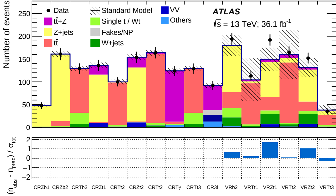
Figure 3: Comparison of the data with the post-fit SM prediction of the background in each control and validation region. The different background components are denoted by the colour specified in the legend. All systematic uncertainties defined in Sect. 6 and statistical uncertainties are included in the shaded band. The lower panel shows the pulls in each VR. The total uncertainty \sigma_{\text{tot}} includes systematic and Poisson uncertainties for each given region.
