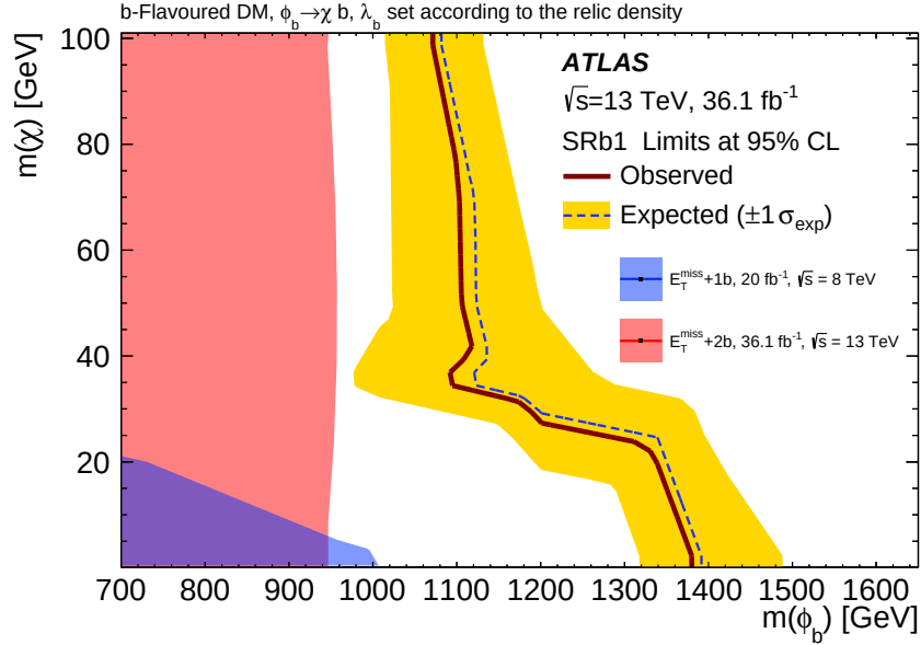
Figure 8: Exclusion limits for colour-charged scalar mediators ( b -FDM) as a function of the mediator and DM masses for 36.1 \text{ fb}^{-1} of data. The limits are calculated at 95% CL. The solid (dashed) line show the observed (expected) exclusion contour for a coupling assumption \lambda_b yielding the measured relic density. No uncertainties on the LO cross-sections are considered for this model. The results are compared with the ATLAS search for b -FDM models [27], represented by the blue contour, and the ATLAS search for direct sbottom pair production [25], represented by the red contour.
