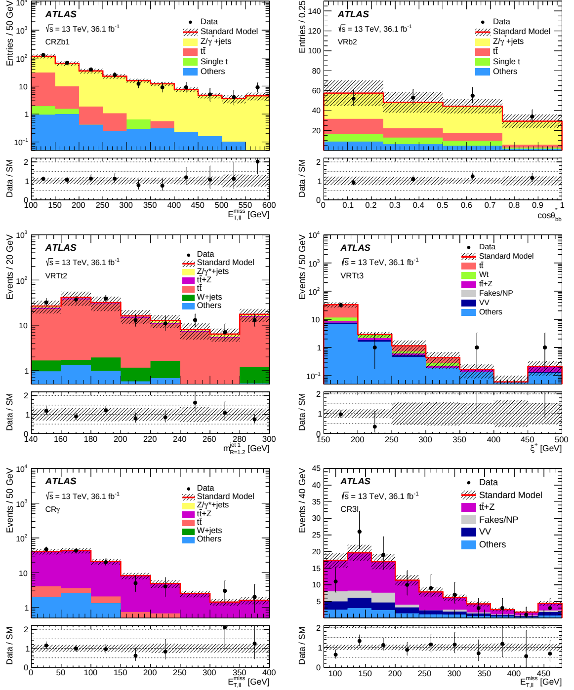
Figure 2: Comparison of the data with the post-fit Monte Carlo prediction of some kinematic distributions in control and validation regions. The bottom panel shows the ratio of the data to the Monte Carlo prediction. The band includes all systematic uncertainties defined in Sect. 6. The last bins include overflows, where applicable. The top left panel shows the E_{T,\ell\ell}^{\text{miss}} distribution in CRZb1. The E_{T,\ell\ell}^{\text{miss}} requirement is relaxed to 100 GeV. The other panels show the \cos\theta_{bb}^* distribution in VRb2 (top right), the m_{R=1.2}^{\text{jet1}} distribution in VRTt2 (middle left), the \xi^+ distribution in VRTt3 (middle right), the E_{T,\ell\ell}^{\text{miss}} distribution in CR \gamma (bottom left) and the E_{T,\ell\ell}^{\text{miss}} distribution in CR3 \ell (bottom right).
