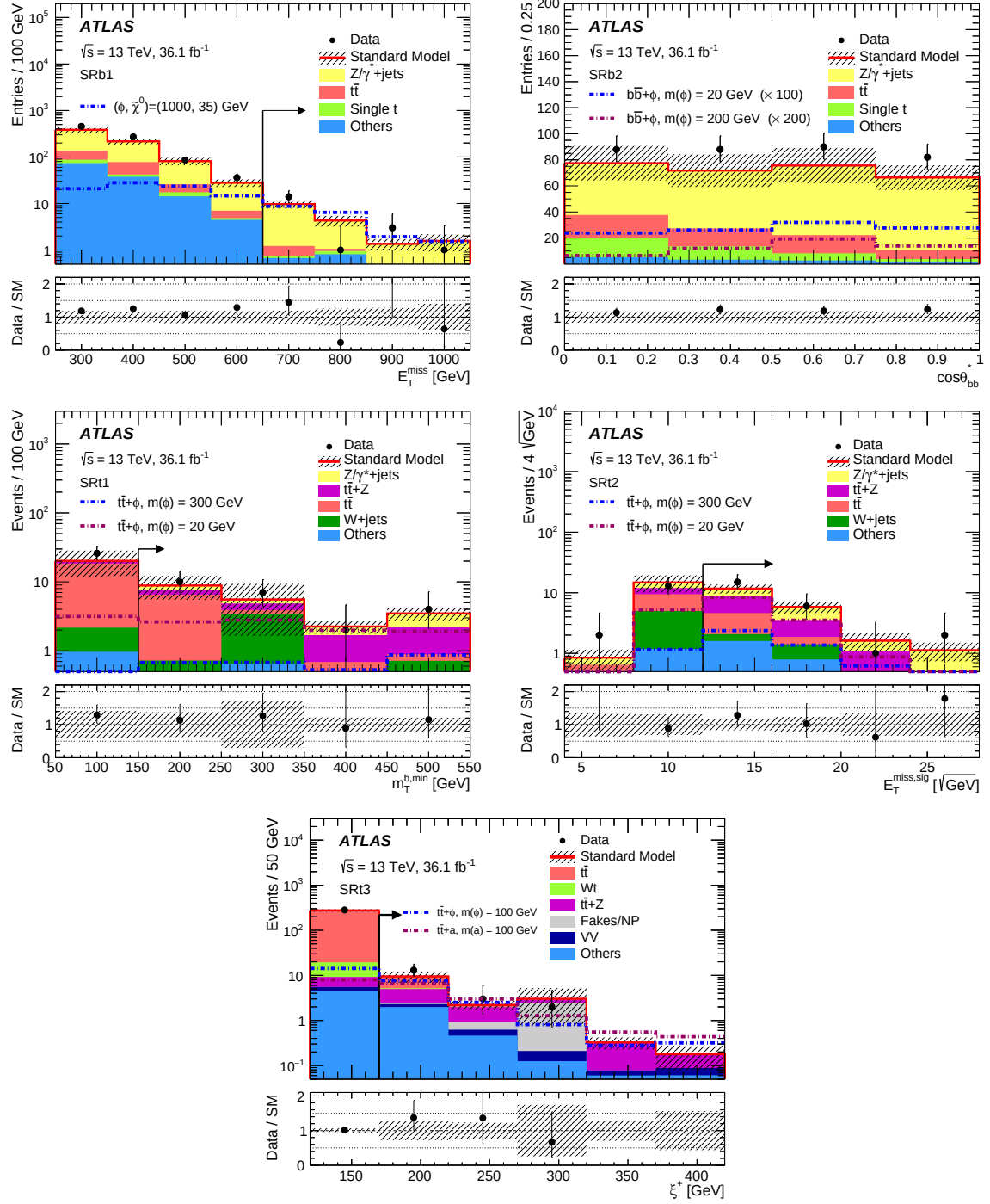
Figure 4: Comparison of the data with the post-fit SM prediction of the E_T^{\text{miss}} distribution in SRb1 (top left), \cos \theta_{bb}^* distribution in SRb2 (top right), m_T^{b,\min} distribution in SRT1 (middle left), E_T^{\text{miss,sig}} distribution in SRT2 (middle right) and \xi^+ distribution in SRT3 (bottom). The last bins include overflows, where applicable. All signal region requirements except the one on the distribution shown are applied. The signal region requirement on the distribution shown is indicated by an arrow. The bottom panel shows the ratio of the data to the prediction. The band includes all systematic uncertainties defined in Sect. 6.
