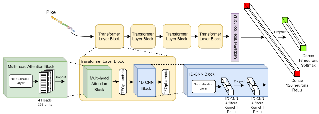
FIGURE 8: Transformer architecture implemented based in [64].
