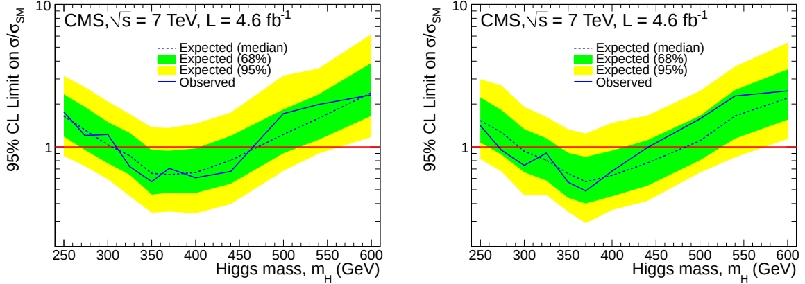
Figure 4: The ratio R of the 95% CL cross section upper limit \sigma to the SM Higgs boson production cross section \sigma_{\text{SM}} as a function of the Higgs boson mass m_H for the cut-based (left) and shape-based (right) analyses.
