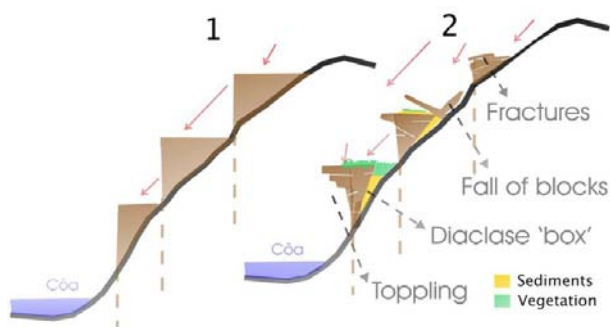
Figure 3: Schematic illustration of mechanical instability in the slopes caused by gravitational pressure aided by seismic forces and rock expansion and retraction cycles.
