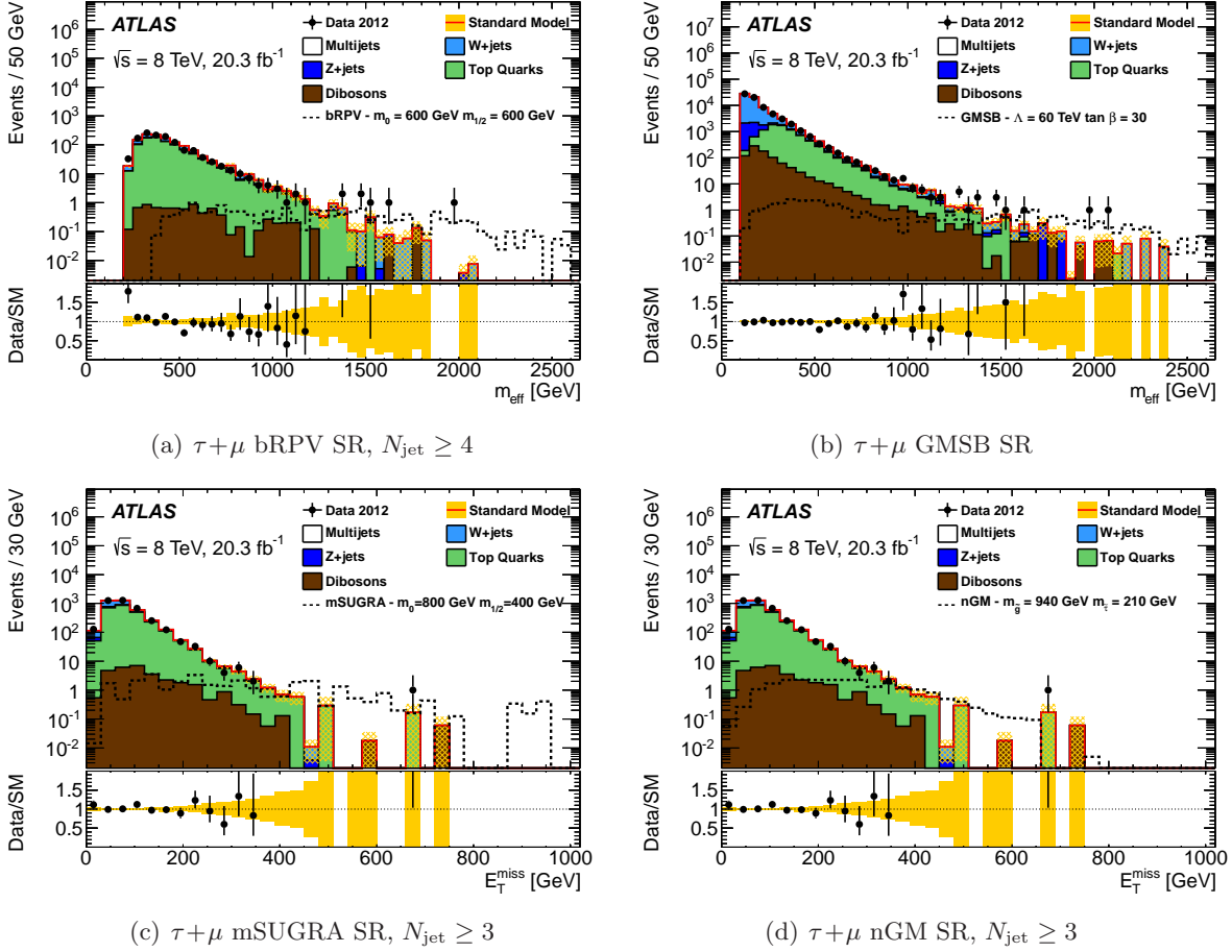
Figure 7. Distribution of the final kinematic variables in the \tau+\mu channel after all analysis requirements but the final SR selections on m_{\text{eff}} and E_{\text{T}}^{\text{miss}} . Data are represented by the points. The SM prediction includes the data-driven corrections discussed in the text. The shaded band centred around the total SM background indicates the statistical uncertainty on the background expectation. MC events are normalized to data in the CRs described in the text. Also shown is the expected signal from typical bRPV, GMSB, mSUGRA and nGM signal samples. The last bin in the expected background distribution is an overflow bin. There are no data events in the overflow bin after all analysis requirements are applied.
