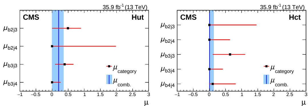
Figure 8: The best fit signal strength ( \mu ) for Hut (left) and Hct (right), which is restricted to positive values in the fit.
