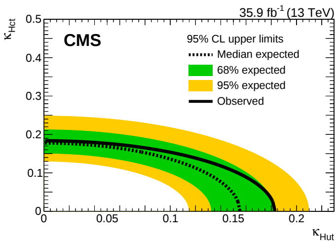
Figure 7: Upper limits on \kappa_{\text{Hut}} and \kappa_{\text{Hct}} at 95% CL.
